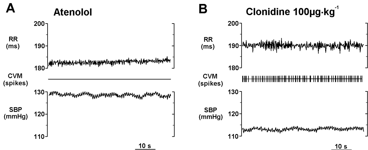
Figure 24. BP lability, sinus arrhythmia and CVM activity following cardiac vagal activation with clonidine 100 \mu\text{g.kg}^{-1} i.v.
