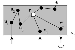
FIG. 2. In the perturbative approach, we assume a single nonlinear two-photon scattering event ( \square ), but arbitrarily many linear scattering events ( \bullet ). One of the two photons is finally annihilated by the detector, thereby defining the photodetection signal, whereas the other one is scattered into an arbitrary direction.
