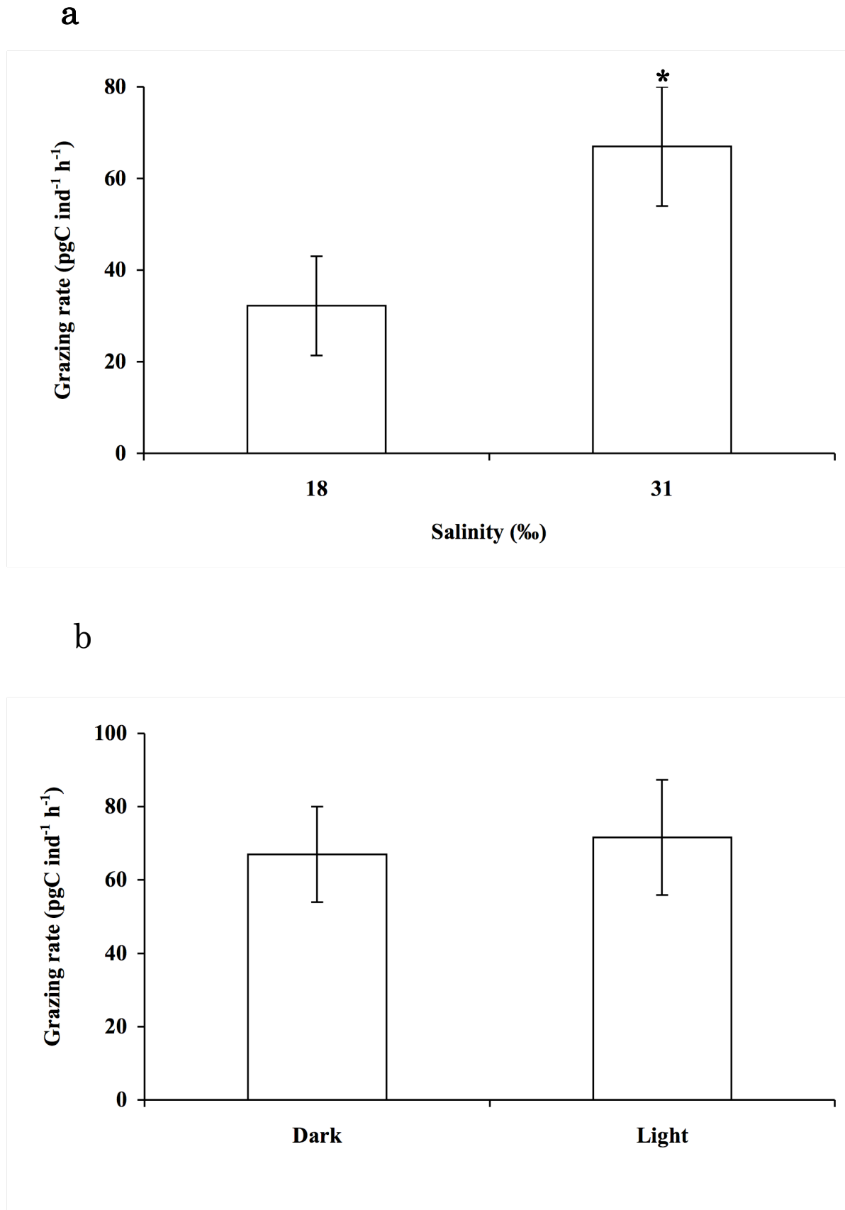
Figure 3a & 3b. Bacteria uptake rate (mean \pm SD, N = 3) under low versus high salinity (a) and dark versus light incubation (b). * indicate significant difference (t-test).
