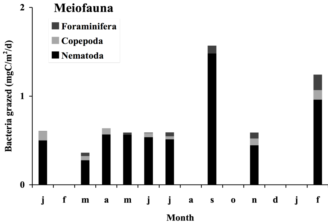
Figure 5. Bacteria grazed (mgC m -2 d -1 ) by meiofauna in surficial sediment at station 3 through the year.
