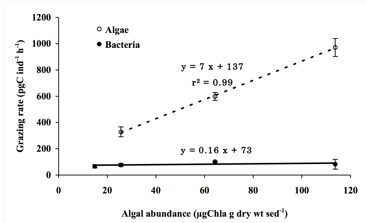
Figure 5. Algae uptake rate ○ (mean ± SD, N = 3) and bacteria uptake rate ● (mean ± SD, N = 3) as function of algal abundance (µgChla g dry wt sed -1 ) under constant bacteria abundance ( 10.5 \times 10^8 cell ml wt sed -1 ).
