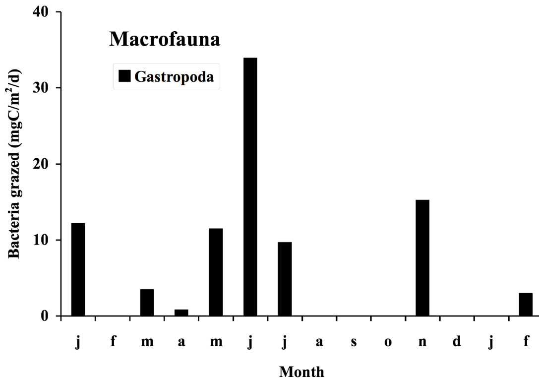
Figure 6. Bacteria grazed (mgC m -2 d -1 ) by H. ulvae in surficial sediment at station 3 through the year.
