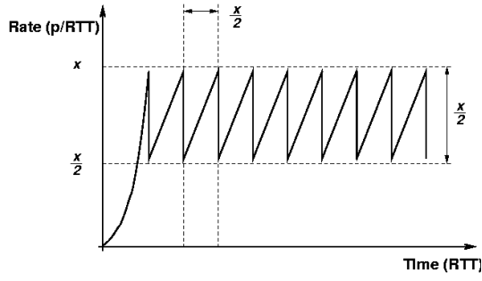
(a) Standard TCP - Small Capacity
