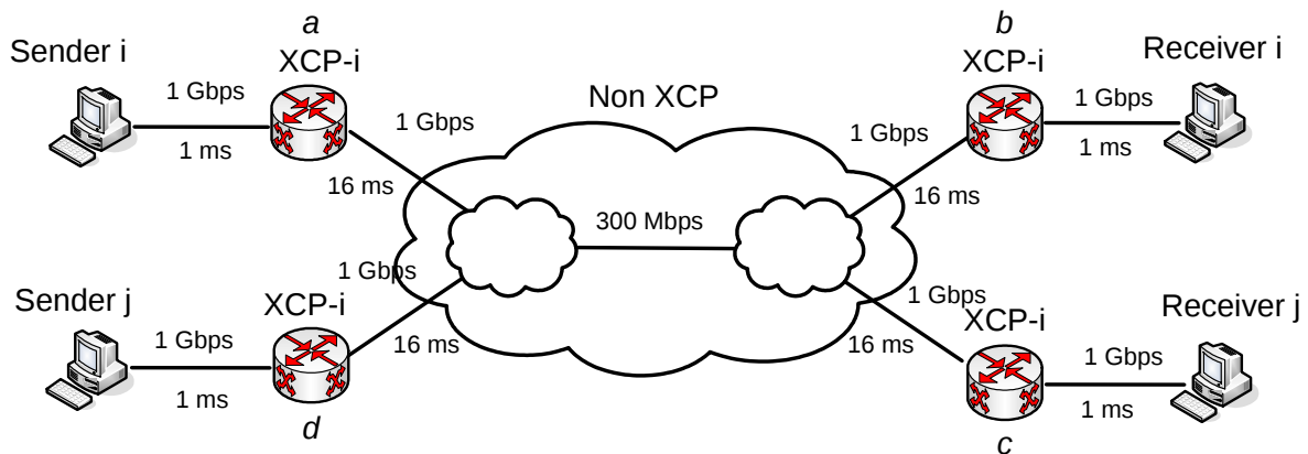
Figure 4.18: 1 bottleneck link shared by n XCP paths
