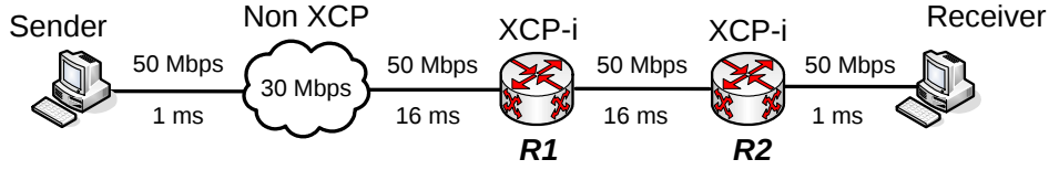
Figure 4.6: Asymmetric deployment: optimized receiver side
