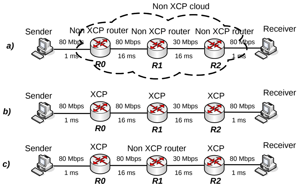
Figure 4.1: (a) scenario for TCP, (b) and (c) scenarios for XCP.
