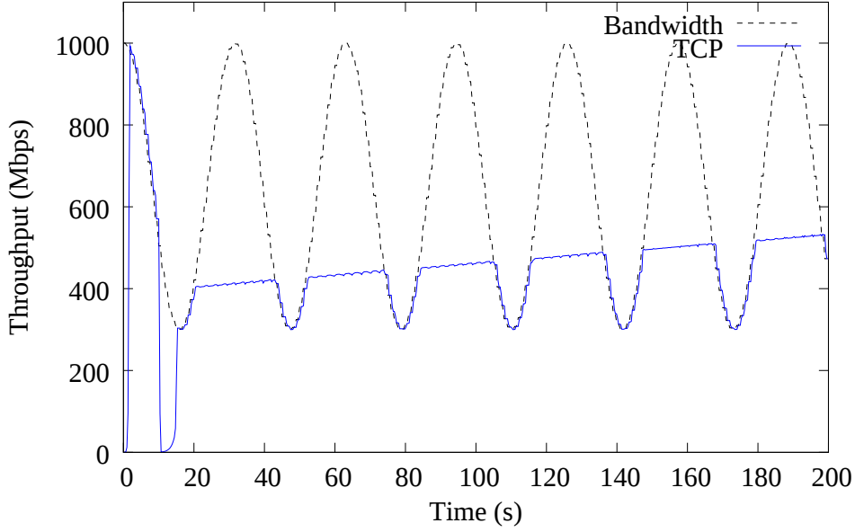
Figure 3.5: TCP New Reno ( RTT \approx 100ms ) on a sinusoidal-based VBE.
