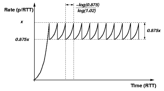
(b) STCP - Small Capacity
