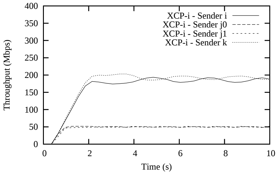
Figure 4.12: Throughput of XCP- i on Topology of Fig. 4.11
