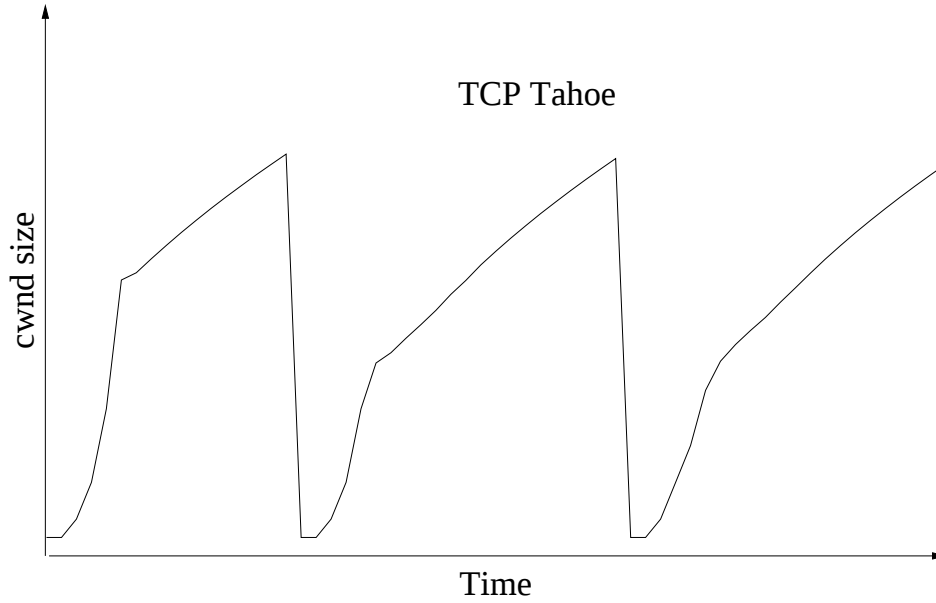
Figure 2.3: TCP Tahoe - The cwnd evolution.
