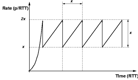
(c) Standard TCP - Large Capacity
