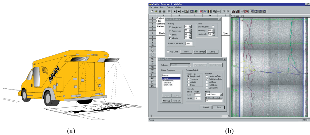
Figure 2.20: According to [Roadware Group, Inc.], (a) Roadware's Automatic Road Analyzer (ARAN ® ), (b) WiseCrax ® system screen: automatically detected cracks overlaid on pavement image.
