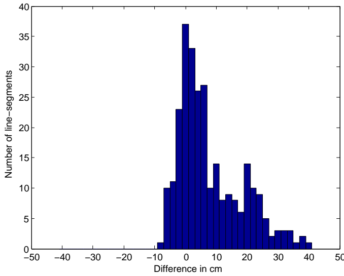
Figure 6.10: Histogram of \sigma_{C_{1,2}} corresponding to 138 reconstructed strips.
