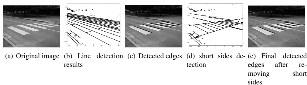
Figure 2.14: According to [Se und Brady, 2003]: Zebra-crossing detection: long sides are detected by vanishing point segmentation, short sides are detected in the orthogonal direction and removed to perform a more accurate Hough transformation for estimating long sides. Enhancement can be compared between (a) and (e)
