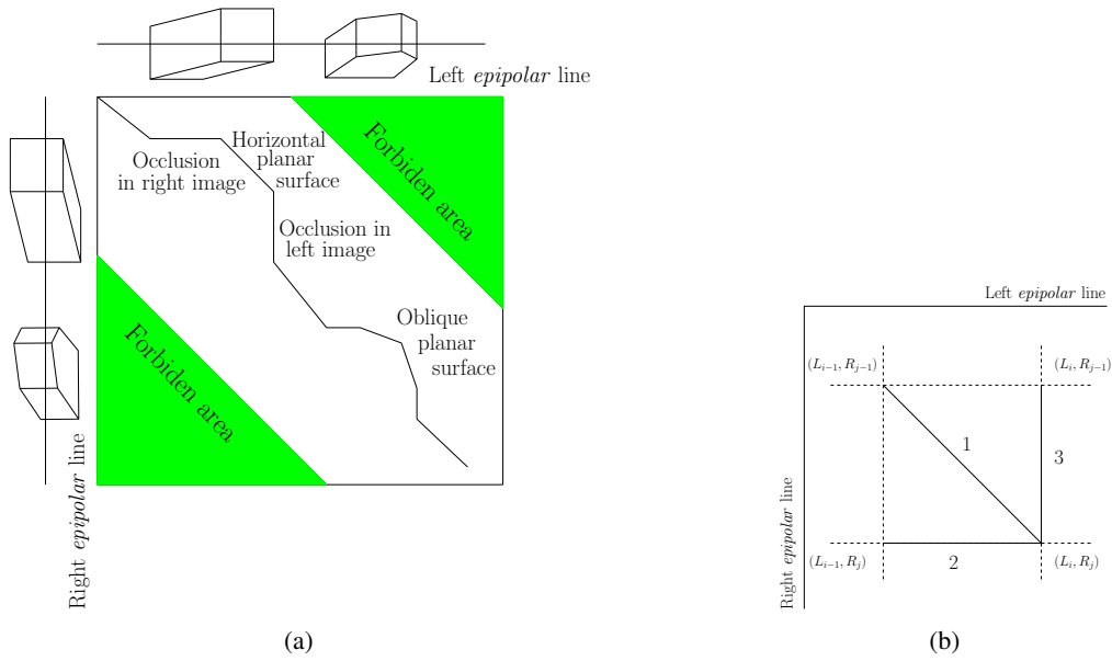
Figure 3.5: According to [Baillard und Dissard, 2000], (a) correspondence graph and matching path, (b) Elementary paths for dynamic programming
