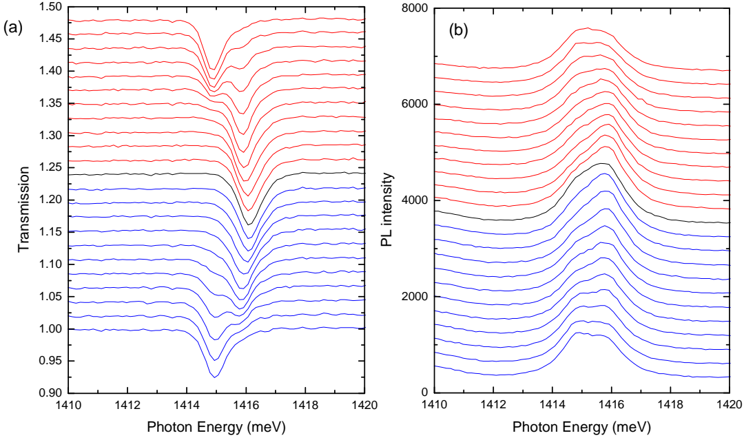
Figure 3.7: Transmission (a) and PL (b) spectra of \text{Mn}^{3+} in diluted \text{Ga}_{1-x}\text{Mn}_x\text{N} grown in Göttingen using MOCVD technique. The temperature for both measurements : PL and transmission is 1.7 K. Sample #G0117.
