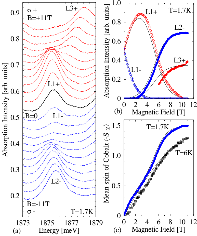
Figure 3.4: (a) Absorption spectra of \text{Zn}_{0.955}\text{Co}_{0.045}\text{O} measured in the Faraday configuration, at 1.7 K, in a magnetic field up to 11 T, in \sigma^+ and \sigma^- circular polarizations. The four transitions observed are labeled according to Fig. 3.3(d). (b) Absorption intensity measured at T = 1.7 K (symbols) and calculated using Maxwell-Boltzmann statistics (lines). (c) Mean spin of Co calculated from the absorption intensities (symbols) or from Maxwell-Boltzmann statistics and parameters of Table 3.2 (lines). Sample #Z217.
