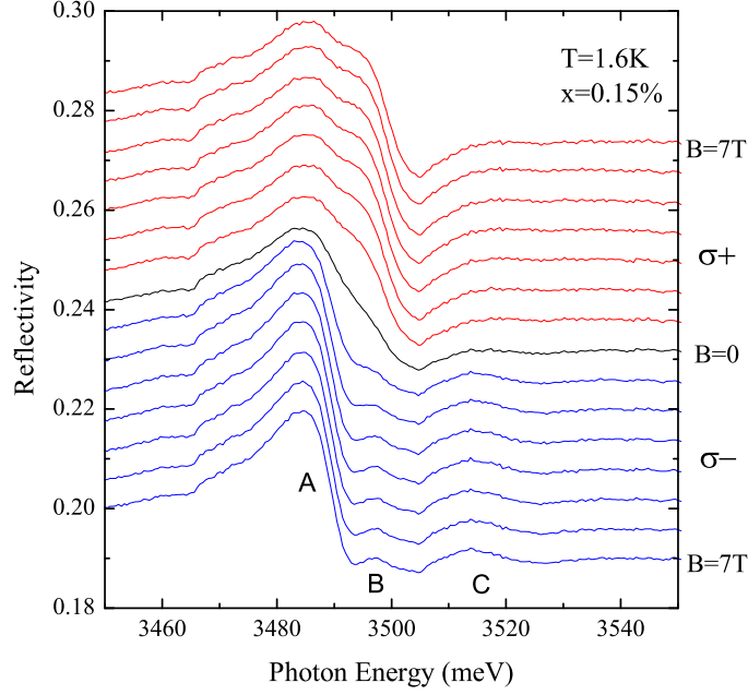
Figure 5.29: (a) Reflectivity of Ga_{1-x}Fe_xN with x = 0.15\% (sample #647) at T = 1.6 K, in Faraday configuration. In \sigma^- polarization (see bottom spectrum) A , B , and C excitons are well resolved. Exciton C is much weaker in \sigma^+ polarization (see upper spectra).
