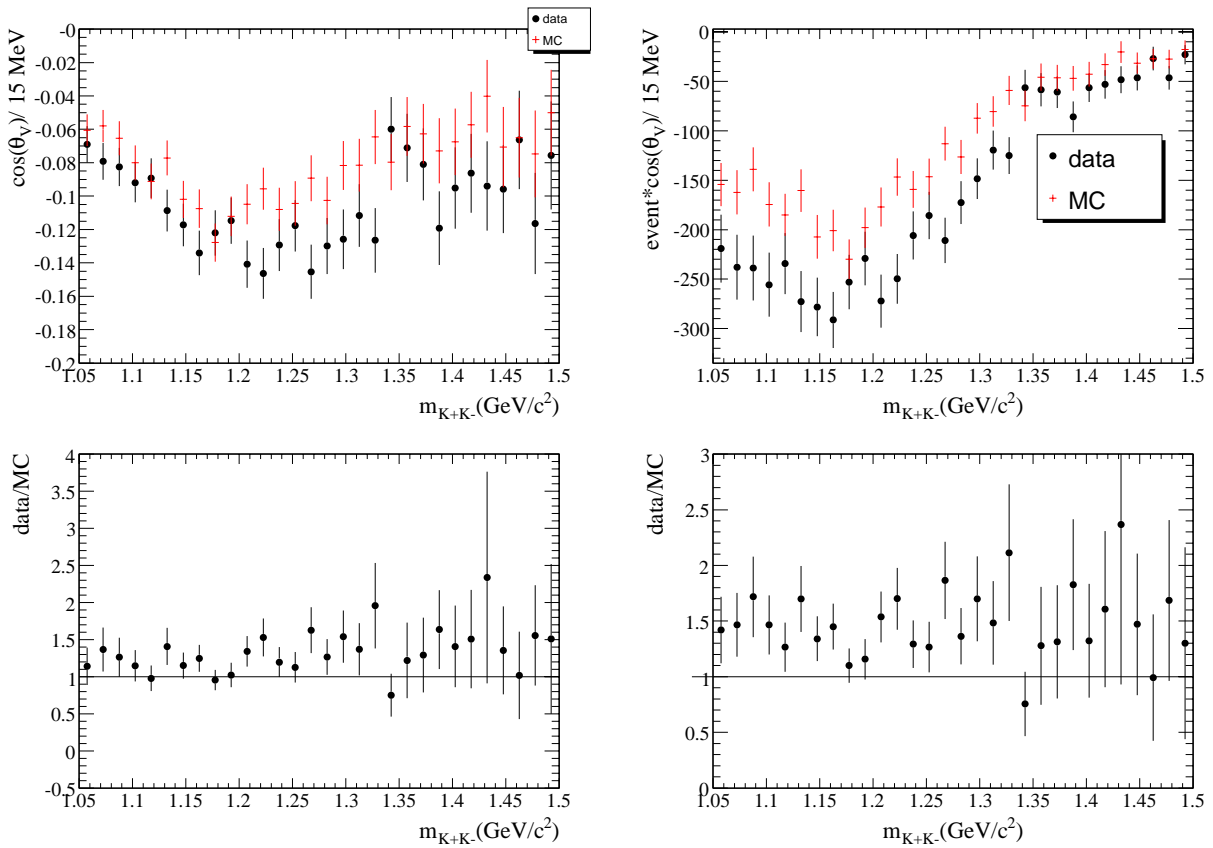
Figure 4.37: Left hand plots: \text{data}/\text{MC} comparison for the mean value of \cos(\theta_V) per K^+K^- mass bin and \text{data} over \text{MC} ratio. Left hand plots \cos(\theta_V) as function of K^+K^- mass, uds and B\bar{B} events have been subtracted from data.
