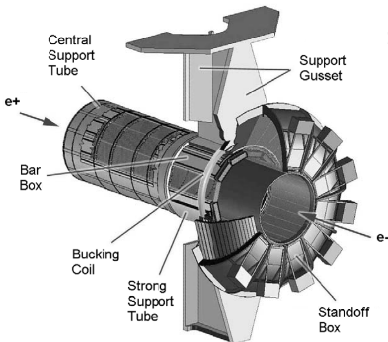
Figure 2.12: Schematic view of the principal components of the DIRC mechanical support structure.
