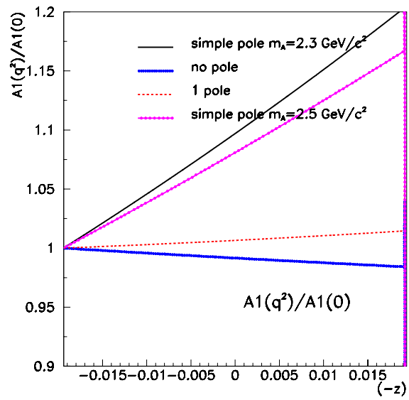
Figure 9.10: Variation of the A_1(q^2) form factor parameterization versus -z , not including the z expansion and considering that no, or one pole contributes. These distributions are compared with the simple pole parameterization.
