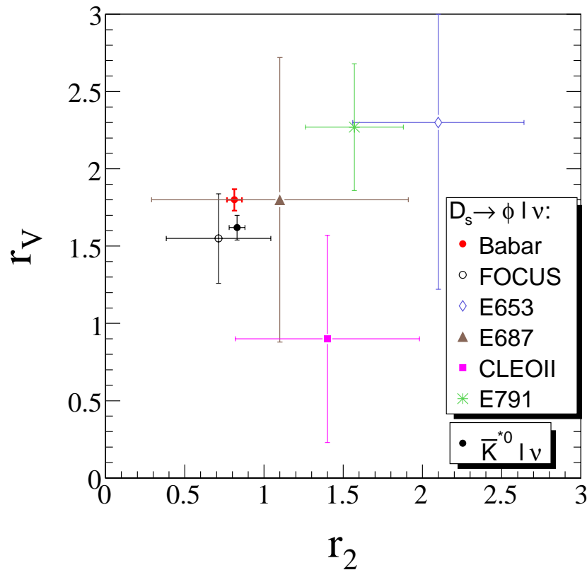
Figure 9.4: Results from previous experiments and present measurement of r_2 and r_V in D_s^+ \rightarrow \phi e^+ \nu_e decays. The error bars represent the statistical and systematic uncertainties added in quadrature. These measurements for D_s \rightarrow \phi e^+ \nu_e decays are compared with the world average of similar measurements obtained for D \rightarrow \bar{K}^{*0} e^+ \nu_e decays [4].
