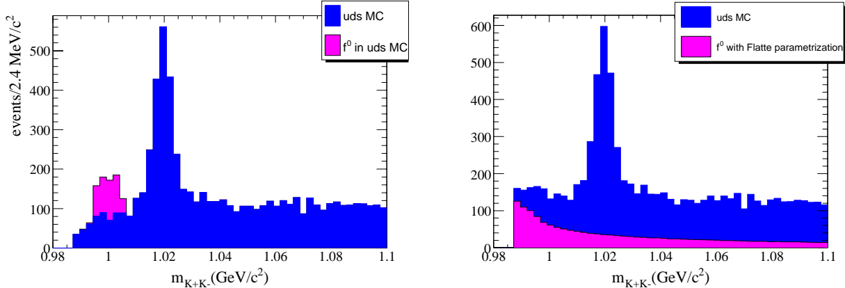
Figure 4.39: K^+K^- mass distribution from light quark simulation. The left plot is the generic MC. Apart from the \phi peak one can see the f_0 contribution (magenta histogram). In the right plot, the f_0 has been replaced by a Flatte distribution.
