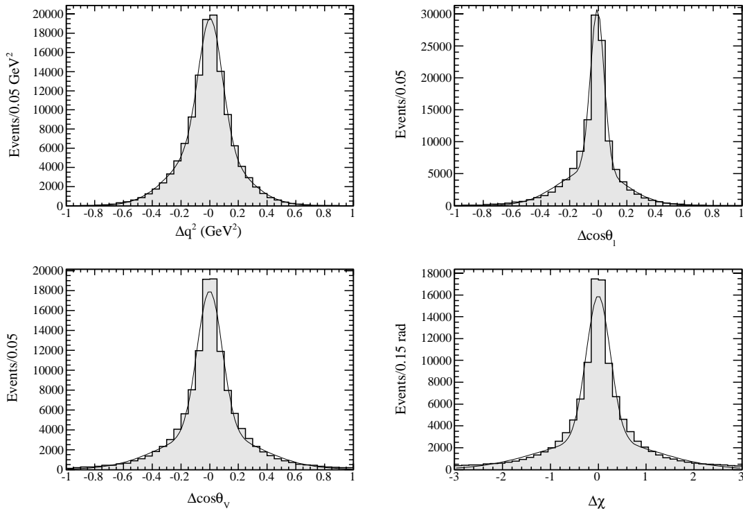
Figure 3.9: Distributions of the difference between the true and the reconstructed value of the four kinematic variables as obtained using simulated events. The fitted curve is the sum of two Gaussian distributions.
