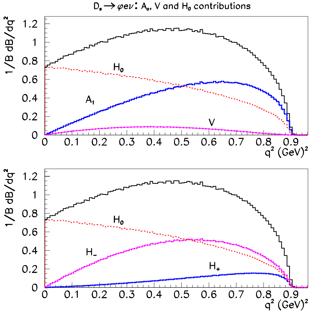
Figure 9.3: Contribution of the form factors A_1 (blue), V (magenta), H_0 (red) to the differential decay rate versus q^2 are compared with contributions from H_+ , H_- and H_0 .
