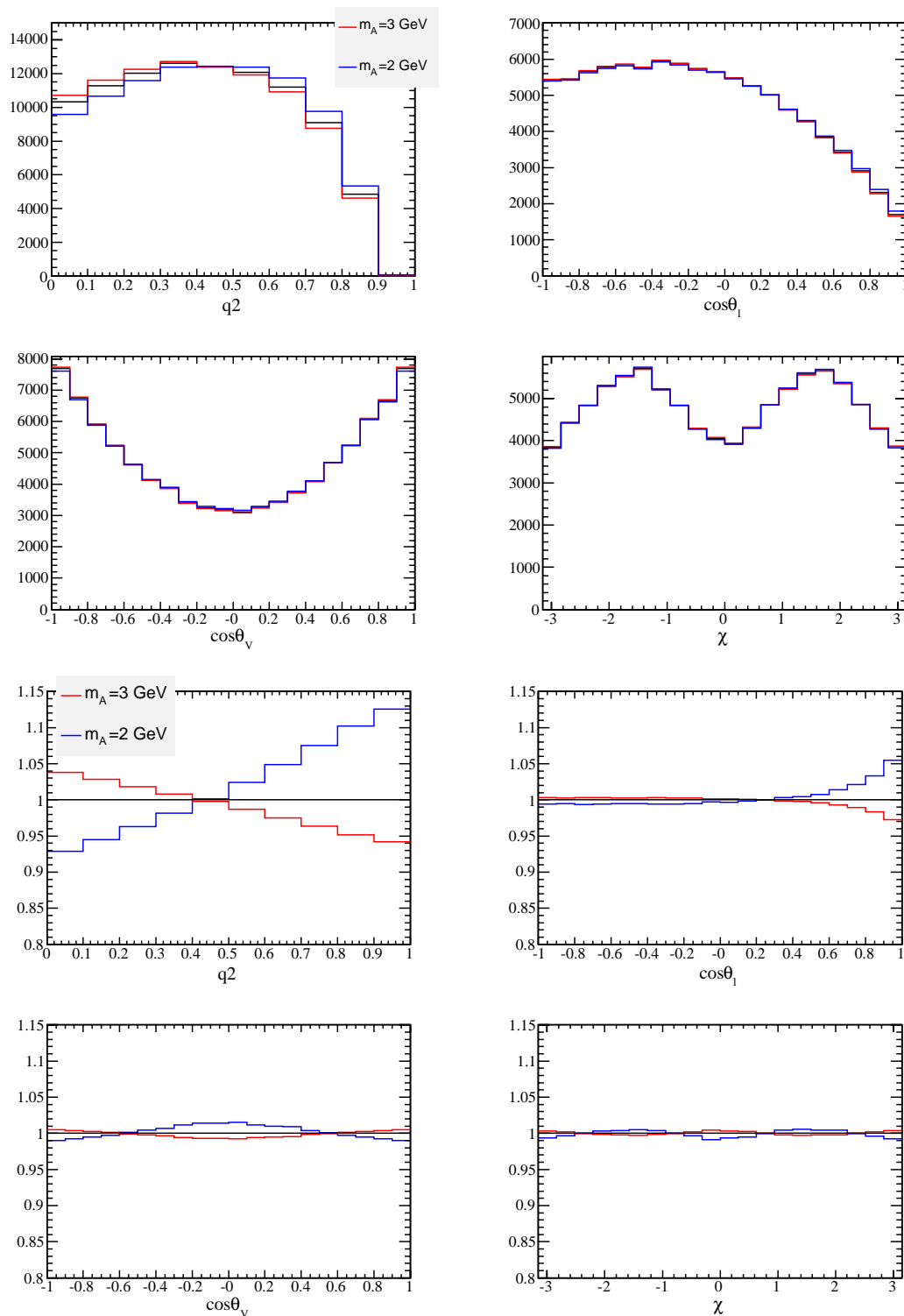
Figure 5.4: Distribution of the kinematic variables for different values of m_A . The reference histogram ( m_A = 2.5 \text{ GeV}/c^2 ) is in black. The bottom plots correspond to the ratio between the histogram m_A^{ref} \pm 0.5 \text{ GeV}/c^2 and the reference histogram.
