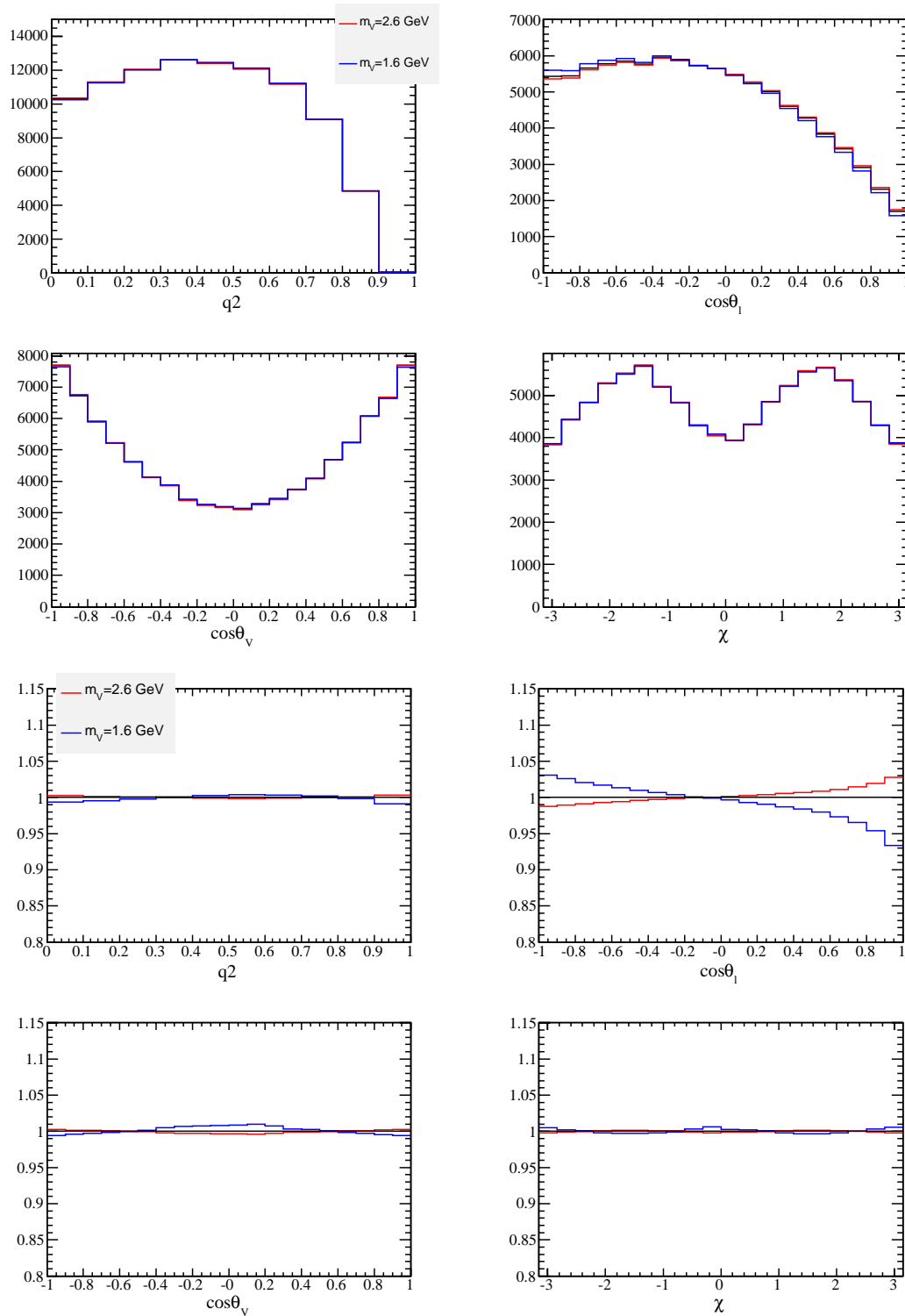
Figure 5.5: Distribution of the kinematic variables for different values of m_V . The reference histogram ( m_V = 2.1 GeV/c 2 ) is in black. The bottom plots correspond to the ratio between the histogram m_V^{ref} \pm 0.5 GeV/c 2 and the reference histogram.
