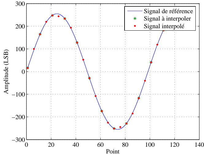
FIG. 5.15 – Interpolation cubique.
