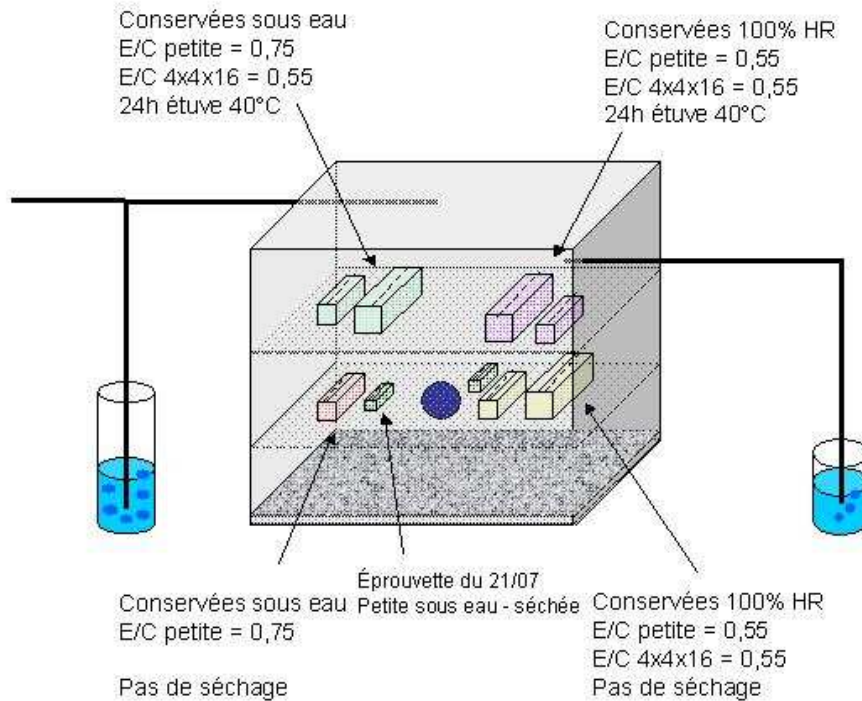
Figure 73 : montage essai 2
