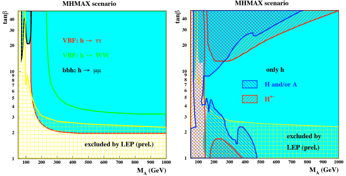
Figure 4.7: Left: lightest Higgs boson h discovery potential in the m_h -max scenario for 30 \text{ fb}^{-1} of integrated luminosity. Right: overall discovery potential for Higgs bosons in the m_h -max scenario for 300 \text{ fb}^{-1} of integrated luminosity.
