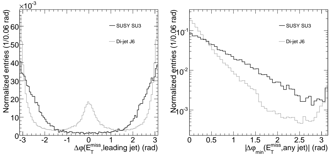
Figure 5.3: Normalized distribution of \Delta\phi(E_T^{\text{miss}}, \text{leading jet}) and |\Delta\phi_{\text{min}}(E_T^{\text{miss}}, \text{any jet})| . Full (dotted) line represents a SUSY SU3 (di-jet J6) sample, defined in the text.
