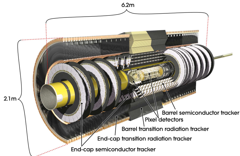
Figure 3.3: Cut-away view of the ATLAS inner tracking detector.
