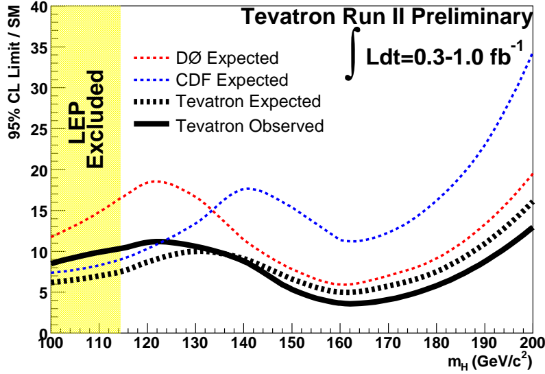
Figure 1.2: Preliminary Higgs exclusion plot from Tevatron experiments CDF and D0 [36]. The expected and observed lower limits on the Higgs production cross-section (expressed in units of the SM prediction) are shown over the accessible mass range, from 115 to 200 GeV. The integrated luminosity varies from 0.3 to 1 \text{ fb}^{-1} , depending on the Higgs decay channel.
