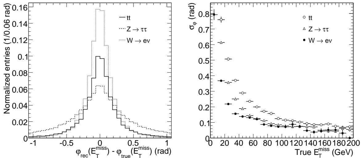
Figure 5.1: Angular difference between reconstructed and true E_T^{\text{miss}} (left) and angular resolution as a function of the true E_T^{\text{miss}} (right) for three different physics channels.
