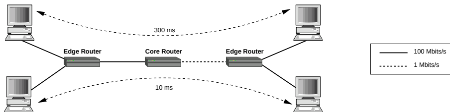
Figure 4.5 The testbed topology for DiffServ experiments
