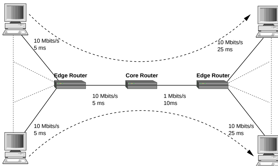
Figure 5.10 Topology
