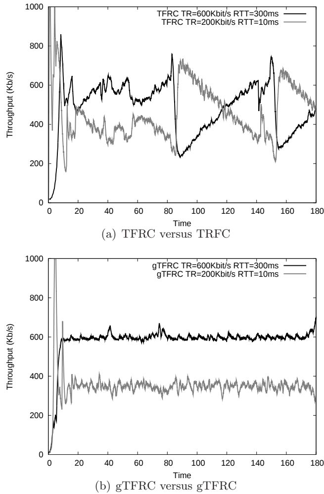
Figure 4.8 Over-provisioned network 20%
