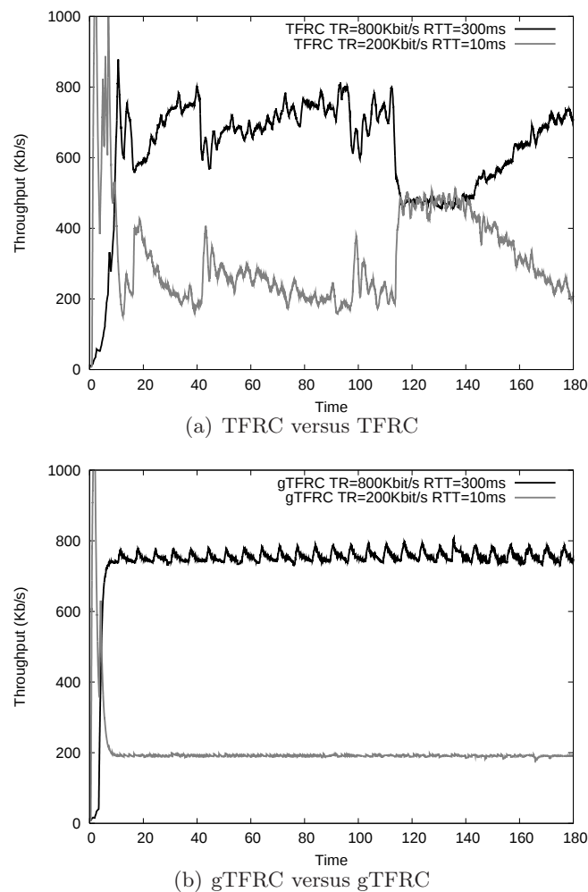
Figure 4.7 Exactly-provisioned network
