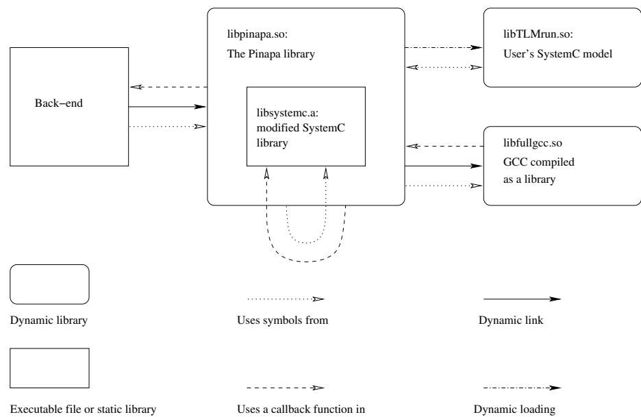
Figure 4.8: Link Mechanism in PINAPA
