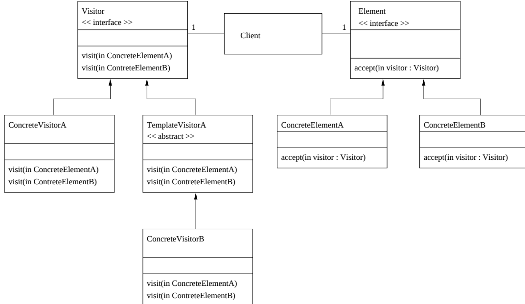
Figure 5.10: “Visitor” Design Pattern
