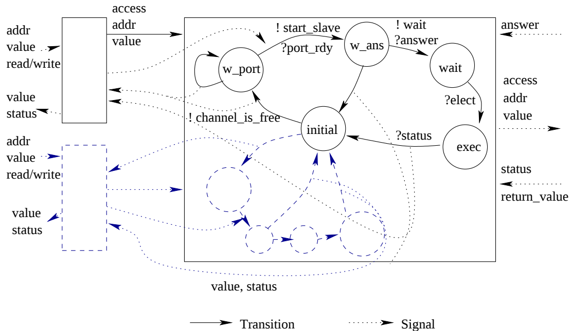
Figure 6.10: Pattern for a basic_seq
