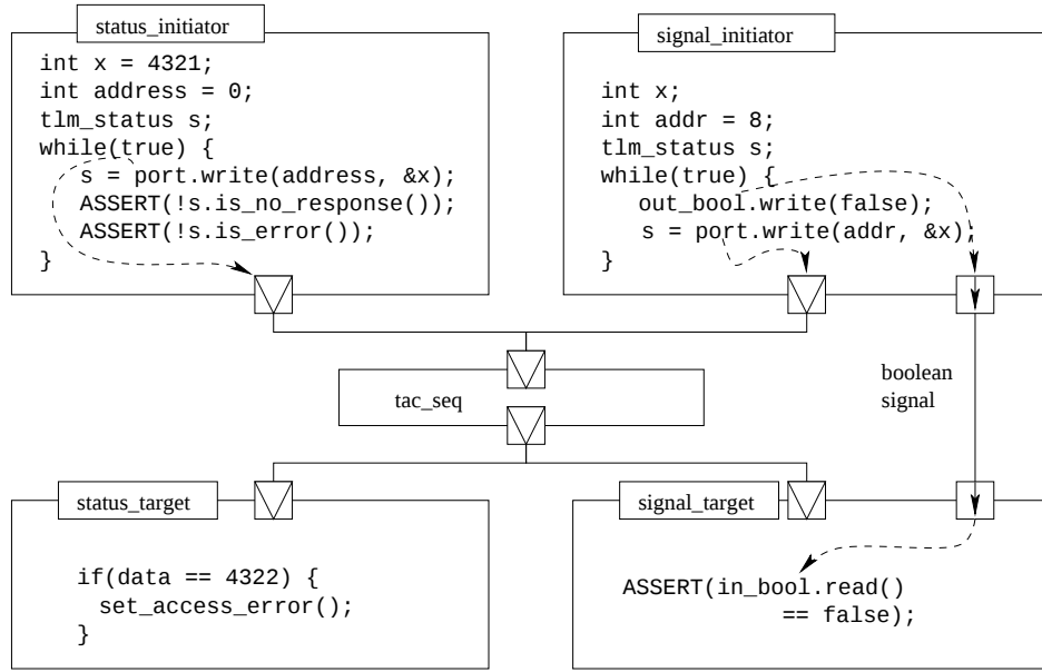
Figure 2.9: An example transactional system
