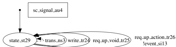
Figure A.14: Automaton for an sc_signal
