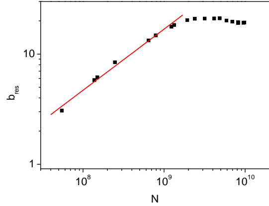
Fig. 10. Optical thickness of the MOT vs number of trapped atoms. The atoms number is changed via the intensity of the repumper laser. The solid line (red online) give a power law with an exponent of 0.55 in the low atom number regime.
