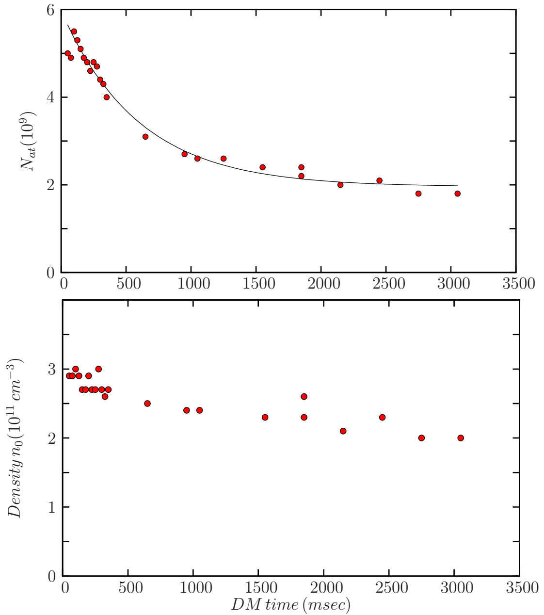
Figure 3.5: Lifetime ( \tau_{life} ) of the atoms in the 'Dark-MOT'. From the exponential fit we extracted ( \tau_{life} \sim 600 \text{ msec} ). We also noticed that our density was not limited by cold collision, as we observed a purely exponential decay.
