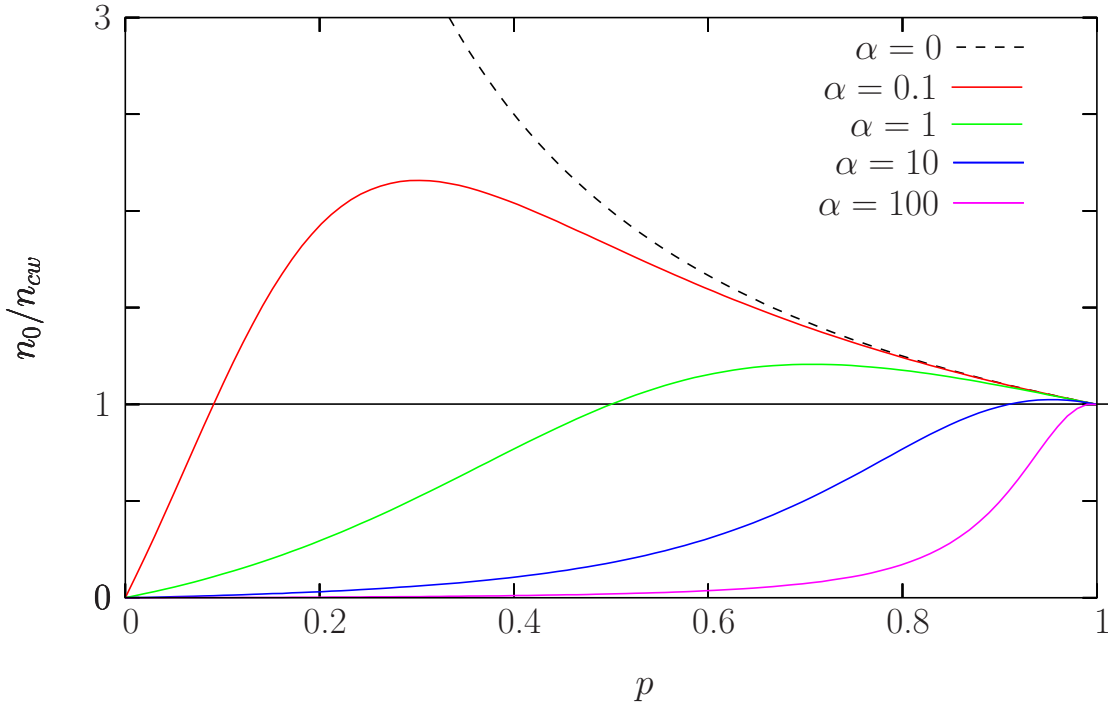
Figure 2.35: MOT center density n_0 , normalized to the density in the Wieman limit n_{cw} as a function of bright state fractions p for different values of \frac{G_2}{G_3} -coefficient( \alpha ). When \alpha=0 (neglecting repumper induced reaction), we obtain the behavior of the density as predicted by Wieman-Pritchard model.
