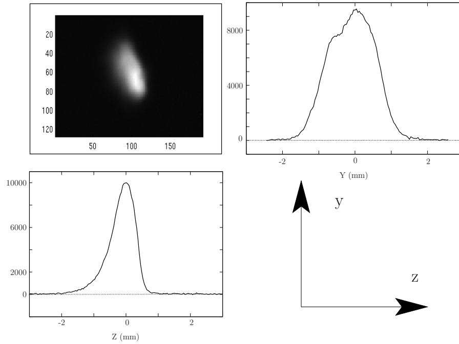
Figure 2.11: Typical MOT fluorescence signal recoded in I_d(x, y) . In the upper-right position a cut of the oy direction is plotted, while in the lower-left there is a cut of the oz direction.
