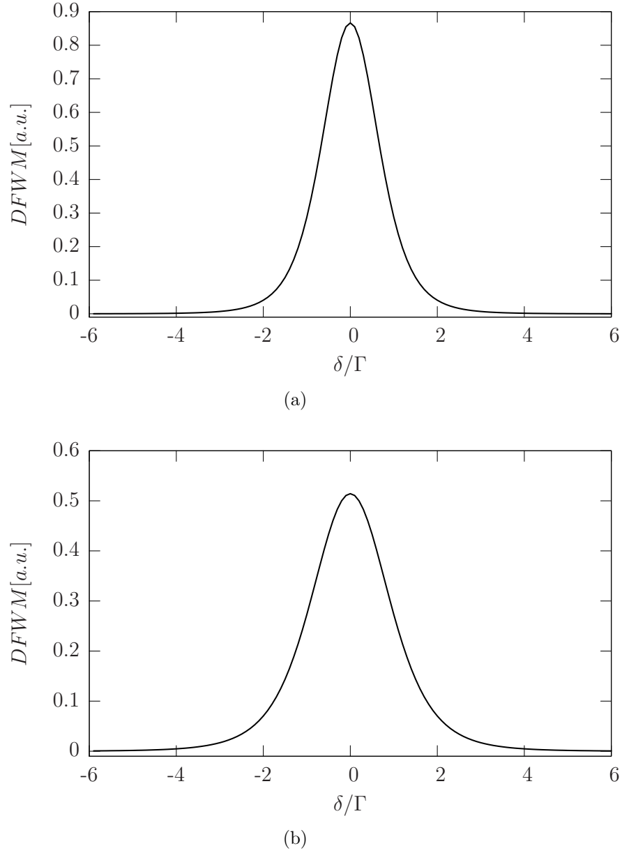
Figure 4.9: Theoretical prediction for DFWM using the Abrams and Lind theory in the parallel case. The spectra shown were obtained by using Eq. (4.31) given in the text. In order to reproduce the experimental condition, in graph (a) the saturation parameter for the pumps was set to s = 2 , while in graph (b) the saturation parameter was set equal to s = 4 .
