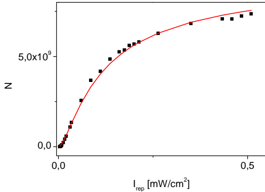
Fig. 8. Experimental result for atom number as a function of repumper intensity. All other parameters correspond to the standard parameters, as defined in the text.
