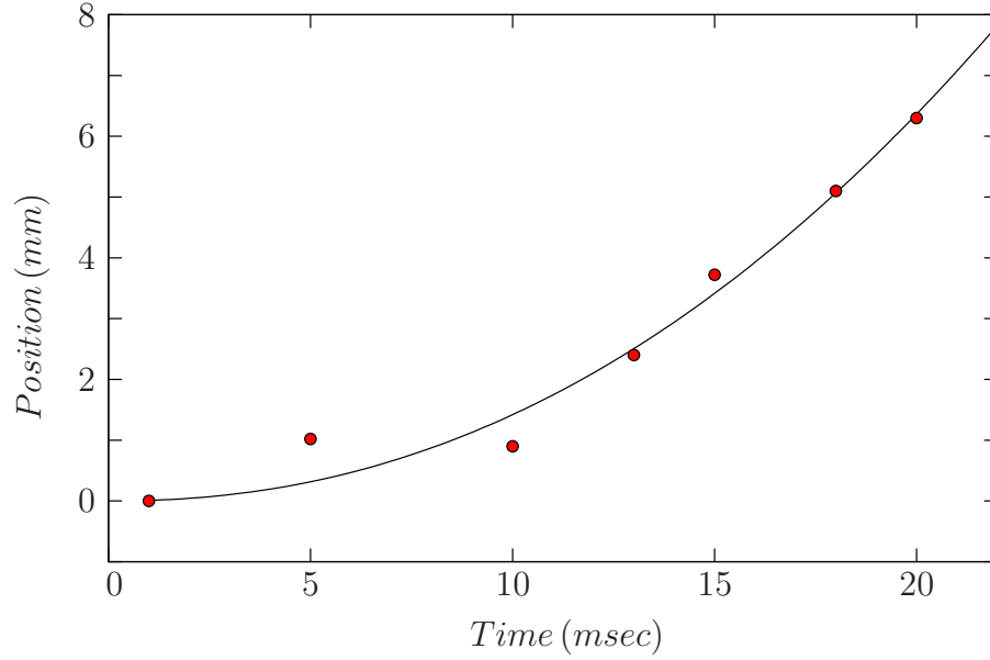
Figure 3.15: Residual "pushing".
