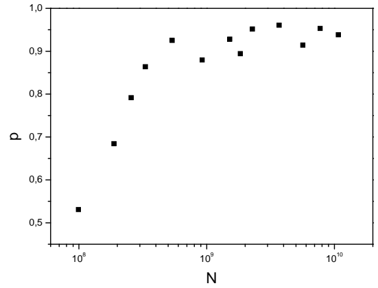
Fig. 14. Proportion p = N_3/(N_2 + N_3) of atoms in the bright ( F = 3 ) state as a function of the total number N = N_2 + N_3 . N is varied by changing the repumper size.
