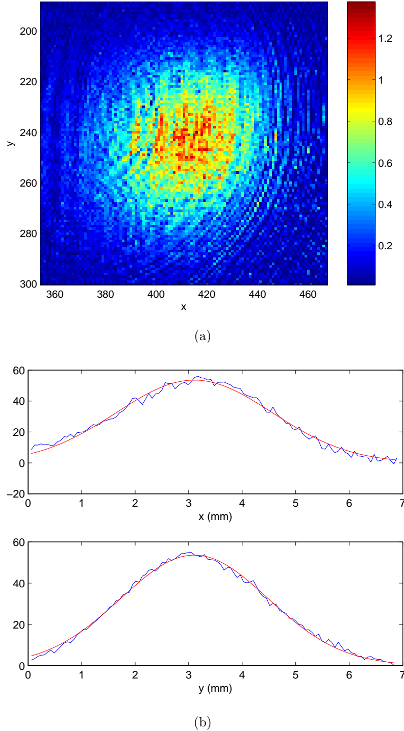
Figure 3.3: The typical absorption image (a), obtained by the method described in the text, is shown, and the projections with the relative Gaussian fit are reported (b). The typical size is found to be \sigma_r \sim 1.5\text{ mm} , with the assumption of an isotropic density distribution. The on-resonance optical thickness in the 'Dark-MOT' is b_0 \sim 100 with N_{at} \sim 10^9 and density of 10^{11}\text{ cm}^{-3} . The experimental image is taken with \delta_{\text{probe}} = -4\Gamma .
