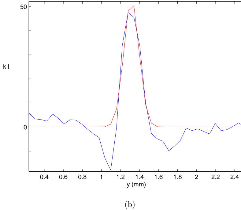
Figure 3.16: The dipole trap loaded from a 'Dark-Mot'. We found a peak-density equal to n_0 = 10^{12} \text{ at/cm}^3 , with N_{at} = 2 \cdot 10^8 atoms, and \sigma_y = 80 \mu\text{m} and \sigma_x 1.2 \text{ mm} .
