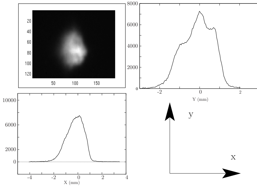
Figure 2.10: Typical MOT fluorescence signal recoded in I_g(x, y) . In the upper-right position a cut of the Y-direction is plotted, while in the lower-left there is a cut of the X-direction.
