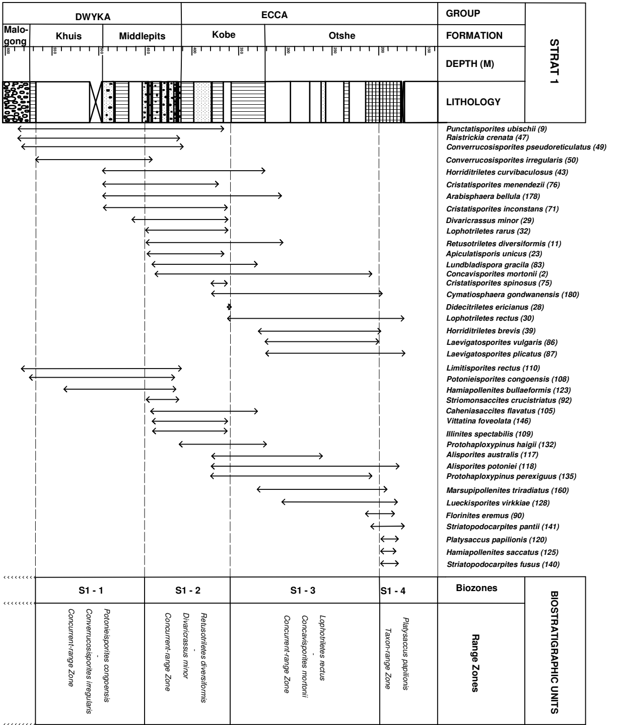
Figure 28: Stratigraphic range chart of significant taxa and biostratigraphic subdivision of STRAT 1 borehole section.
