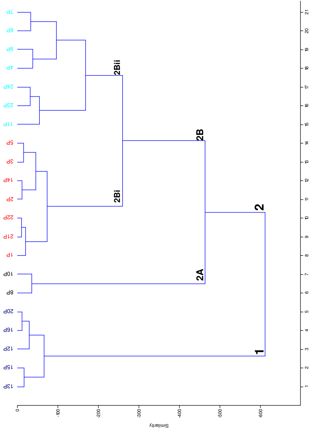
Figure 46: Cluster analysis dendrogram for total sediment organic matter using only samples from the Otshhe formation, Eccla Group.
