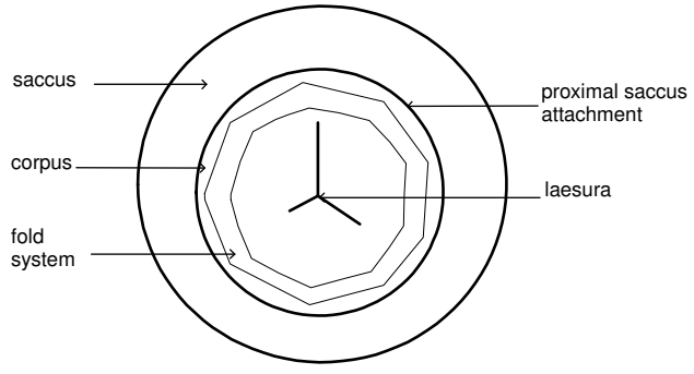
I. Polar view of a trilete monosaccate pollen.
