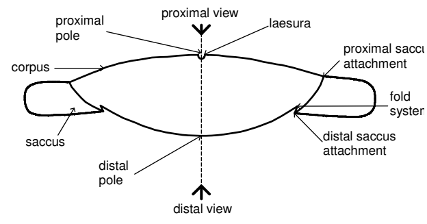
II. Lateral section of a monosaccate pollen.
