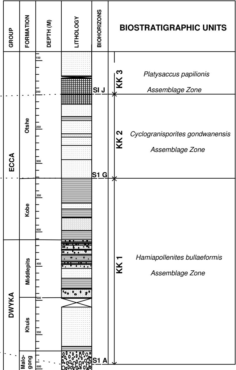
Figure 47: Biostratigraphic correlation of STRAT 1 and CKP 6 boreholes.
