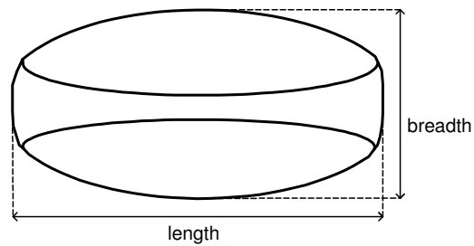
III. Measurement terminology for monocolpate pollen
