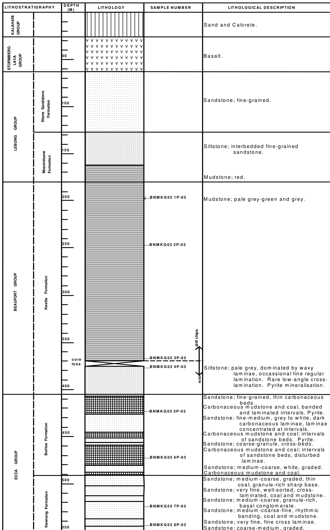
Figure 16: KGO3 borehole section indicating sampled levels.
