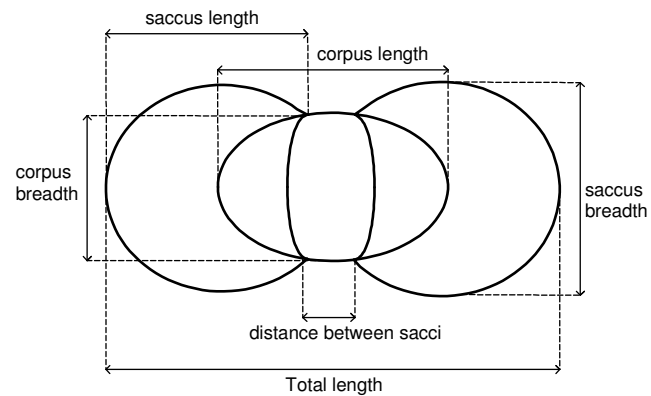
IV. Measurement terminology for bisaccate pollen.
