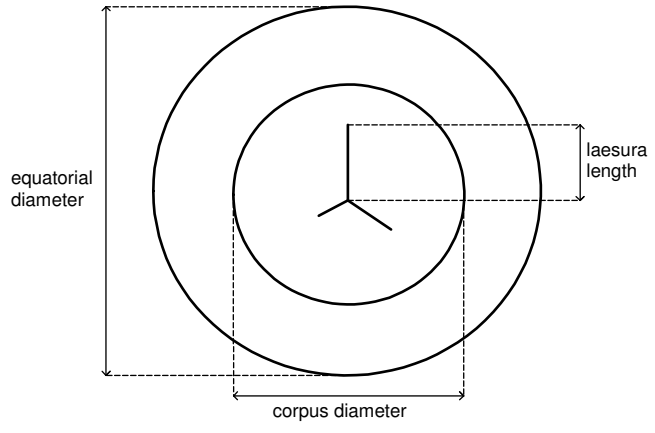
III. Measurement terminology for monosaccate pollen.
