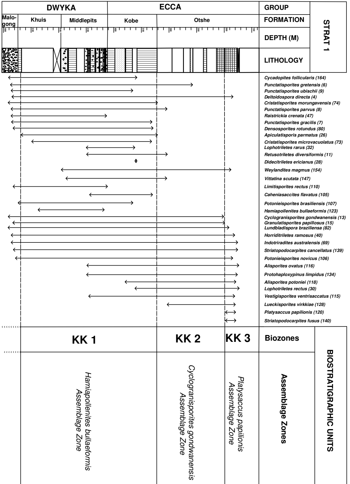
Figure 30: Significant assemblage zone taxa with subdivision of STRAT 1 borehole section.
