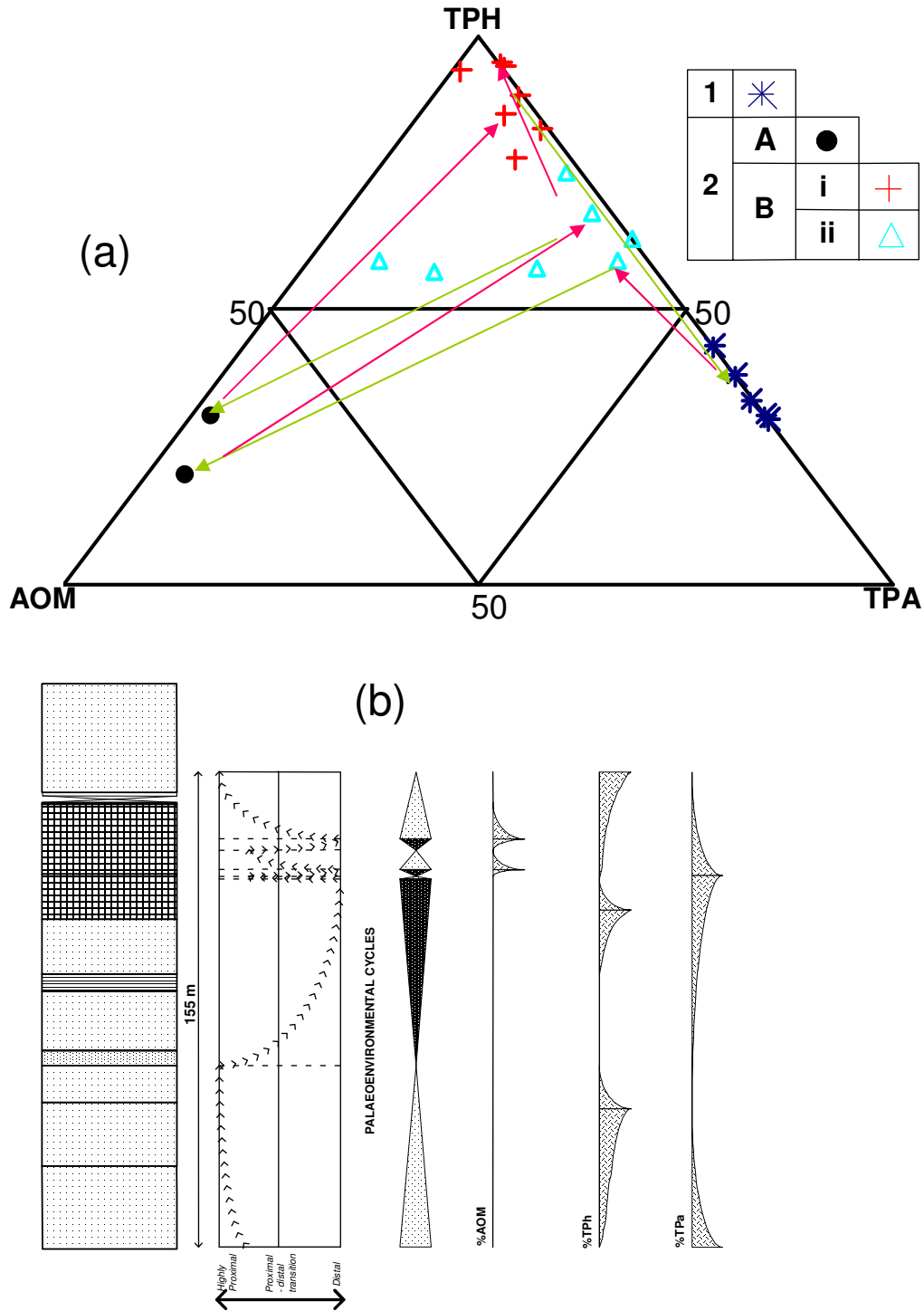
Figure 57: Small-scale palaeoenvironmental stratigraphic cycles in the Otshé Formation: (a) ternary AOM-TPH-TPA plot based on dendrogram of Figure 46, (b) proximal-distal trends, and notable relative abundances for total sediment organic matter.
