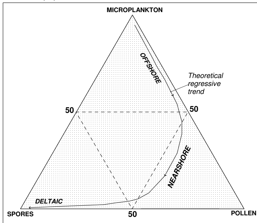
Figure 52: Ternary microplankton-spore-pollen palynomorph plot: (a) ternary plot based on dendrogram of Figure 41, (b) ternary diagram for palynomorphs indicating the characteristic depositional environments.
