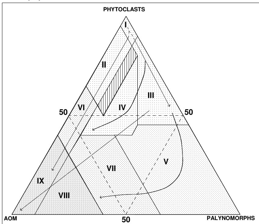
Figure 51: Ternary AOM-total phytoclasts-total palynomorphs plot: (a) ternary plot based on dendrogram of Figure 40, (b) palynofacies fields and environments (see Table 3 for explanations).
