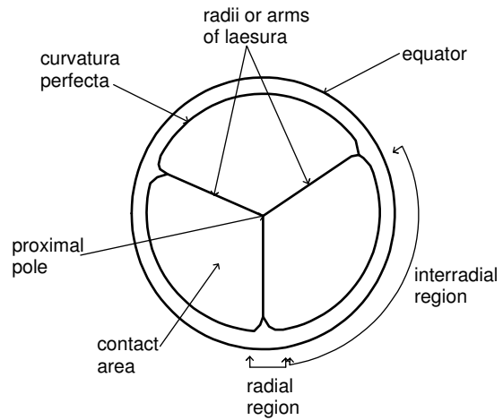
I. Polar view of trilete spore from tetrahedral tetrad.
