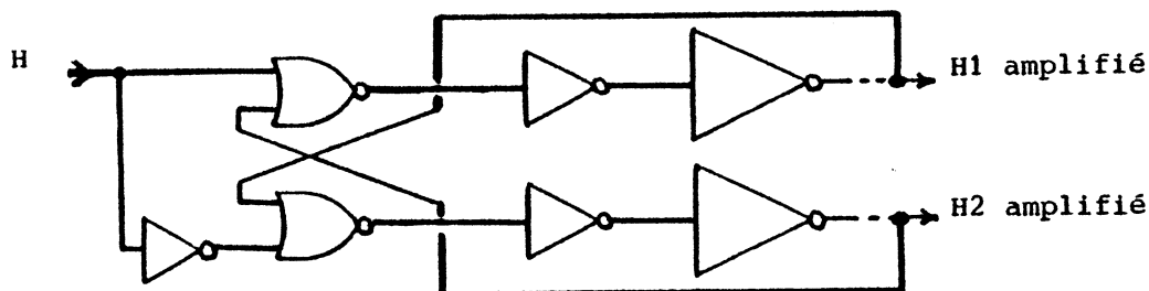
circuit (b)
