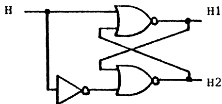
circuit (a)
