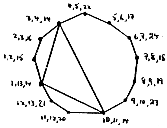
Figure 3.2: I_3(G) .
