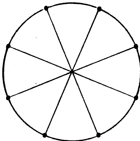
Fig.1 The graph V_8
