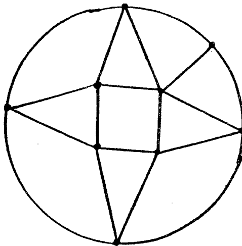
Figure 3.1. K_3 -9-holes.
