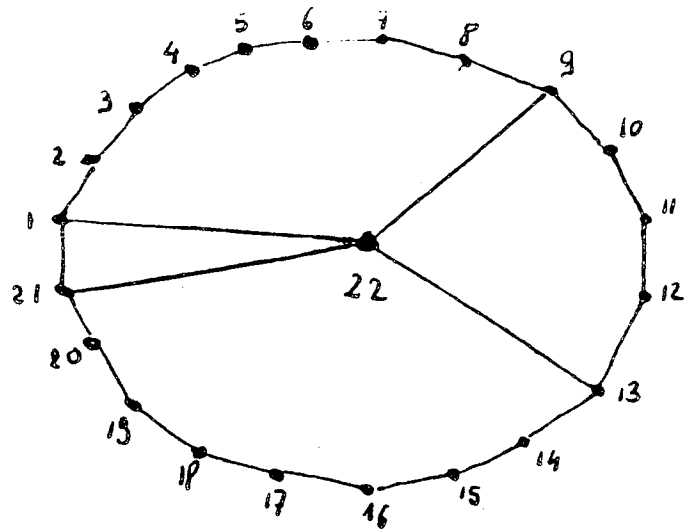
Figure 4.2: I_3(G_1)
