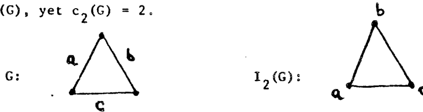
Figure 2.1: c_2(G) \neq k(I_2(G))
