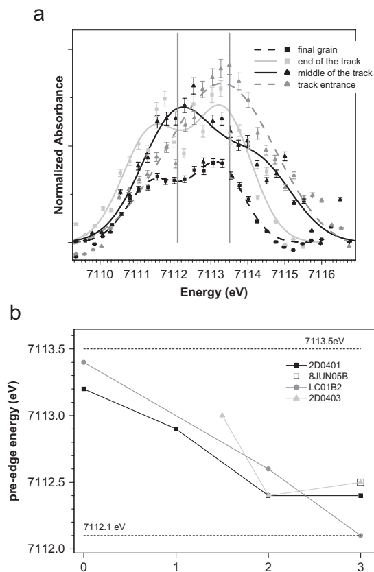
Fig. 4. (a) Normalized pre-edge features of absorption spectra in different regions of 2D0401. The two vertical black lines indicate the two average centroid positions of \text{Fe}^{2+} and \text{Fe}^{3+} compounds (7112.1 and 7113.5 eV). (b) Pre-edge energy as a function of the position in the sample. (0): track entrance, (1): middle of the track, (2): end of the track (3): final grain. The two horizontal dashed lines indicate the two average centroid positions of \text{Fe}^{2+} and \text{Fe}^{3+} compounds.
