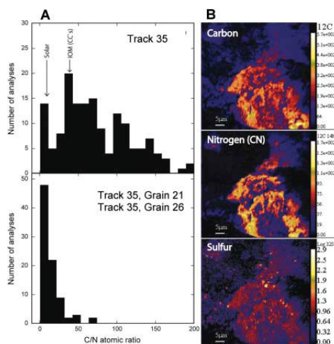
Fig. 4. Distribution of C and N. (A) Histograms of C/N ratios in organics in three different Stardust samples. One sample (top) shows a large spread in C/N, whereas two samples (bottom) have organics characterized by low C/N ratios, consistent with the presence of volatile organic molecules such as HCN or their polymer counterparts. (B) NanoSIMS images of the distribution of C, N, and S in a region of an aerogel sample from along track 35 containing cometary materials. The intensity of the signal increases from blue to red to bright yellow. C, N, and S distributions are clearly correlated, although considerable variations in their relative abundances are observed. S is also present in a population of hot spots that likely indicate the presence of sulfides.
