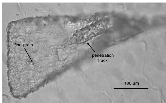
Fig. 1. Optical view of keystone LC01B2. The penetration track, with a substantial amount of the incident grain in it, is clearly identified as well as the final grain, less than 5 μm in size.
