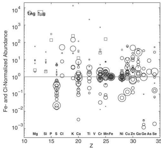
Fig. 2. CI- and Fe-normalized abundance for each element in each of the 23 whole tracks (circles) and in each of the seven crater residues (squares). The area of each data point is proportional to the cross section of an equant particle of equivalent mass. Because much larger masses were analyzed in the craters, there is a difference in the scale size of the two symbols by three orders of magnitude. There is a high degree of variability from track to track, with most elements varying by two orders of magnitude or more.
