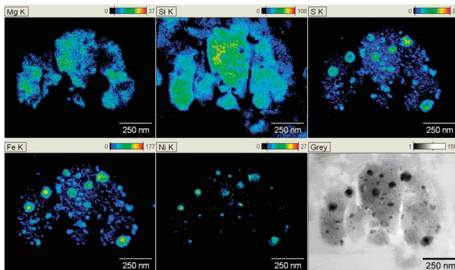
Fig. 4. Elemental x-ray (k-line) maps of a GEMS-like object from a thin section of grain C044, track 7, showing preserved chemical heterogeneity at the 0.1- \mu\text{m} scale typical of GEMS grains in IDPs (33). The Fe, Ni, and S maps show the locations of the nanophase FeNi metal and sulfide inclusions within the amorphous silicate matrix. The gray image is a bright-field TEM image of the GEMS-like object. The color scale in the element maps is x-ray counts.
