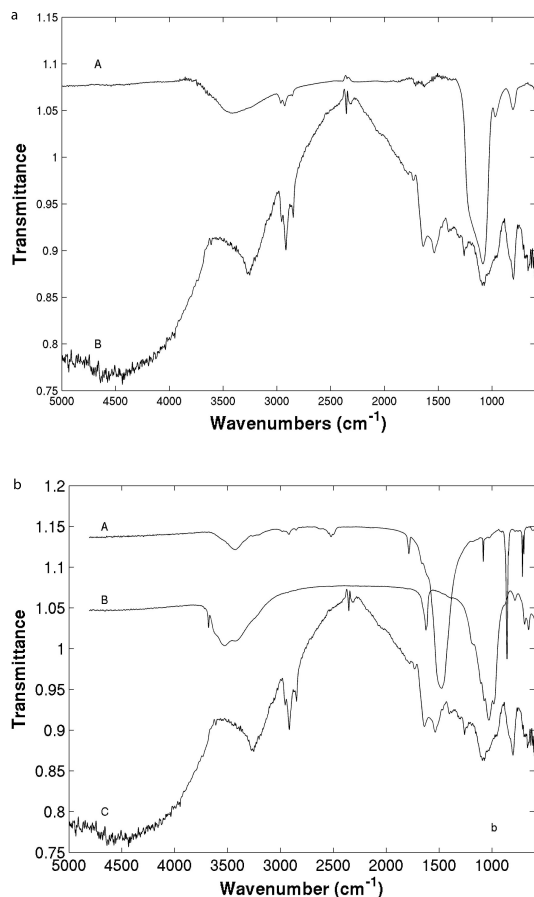
Fig. 8. a) Micro-infrared spectra of (A) aerogel #C2054,32,0,0,0 and (B) particle 35,17. The spectrum of the Stardust particle is modulated by interference of infrared light with a minimum at 4500 \text{cm}^{-1} and a maximum at 2330 \text{cm}^{-1} . Spikes observed at 2330 \text{cm}^{-1} are due to missed compensation for telluric \text{CO}_2 . b) Micro-infrared transmittance spectrum of (A) aragonite ( \text{CaCO}_3 polymorph) and of (B) sepiolite (Hydrated sheet silicate) compared with spectra of (C) particle 35,17. The spectra of the minerals were vertically shifted for sake of clarity.
