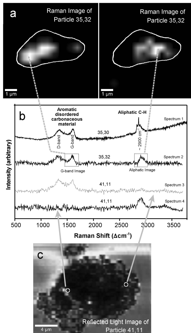
Fig. 6. a) Composite image (360 nm × 360 nm pixels) of Raman band intensities of the microtomed particle 35,32. A full Raman spectrum of each pixel is acquired (see part b), but imaged are only the relative intensities of both the D and G bands (shown on the left-hand side of Fig. 6a) and the C-H band ~2900 Δcm -1 (shown on the right-hand side of Fig. 6a) of each spectrum. Note that spectrum 2 (part b) shows the presence of both components. Overall, however, the Raman images in Fig. 6a show that most pixels in this particle are either dominated by the aromatic sp 2 -bonded carbon phase or the aliphatic hydrocarbon phase. Thus, the aromatic and aliphatic components in this particle are mostly present in spatially separated areas (i.e., as discrete phases) rather than as homogeneously intermixed nanophases. b) Examples of background-corrected Raman spectra obtained on three different particles showing the presence of both disordered carbonaceous material and aliphatic hydrocarbons. Spectrum 1 is from a ~1 μm diameter spot of particle 35,30; spectra 2, 3 and 4 are from individual image pixels from particles 35,32 and 41,11. Note that the observed channel-to-channel fluctuations are dominated by optical interference effects in the instrument, not by counting statistics. c) Visible reflected light image of particle 41,11 that was pressed into a gold foil. The spectra obtained from two selected pixels are shown in Fig. 6b.
