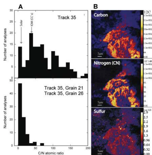
Fig. 4. Distribution of C and N. (A) Histograms of C/N ratios in organics in three different Stardust samples. One sample (top) shows a large spread in C/N, whereas two samples (bottom) have organics characterized by low C/N ratios, consistent with the presence of volatile organic molecules such as HCN or their polymer counterparts. (B) NanoSIMS images of the distribution of C, N, and S in a region of an aerogel sample from along track 35 containing cometary materials. The intensity of the signal increases from blue to red to bright yellow. C, N, and S distributions are clearly correlated, although considerable variations in their relative abundances are observed. S is also present in a population of hot spots that likely indicate the presence of sulfides.
