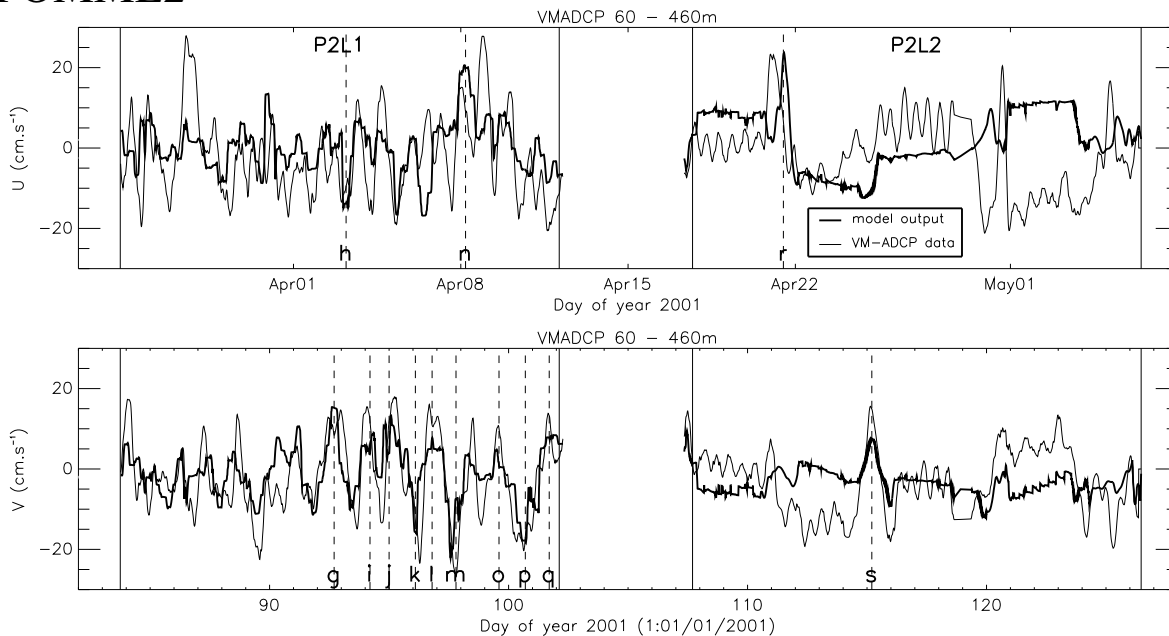
FIGURE 4.9 – VM-ADCP velocities and model velocities during POMME1 and POMME2 following the ship track.
