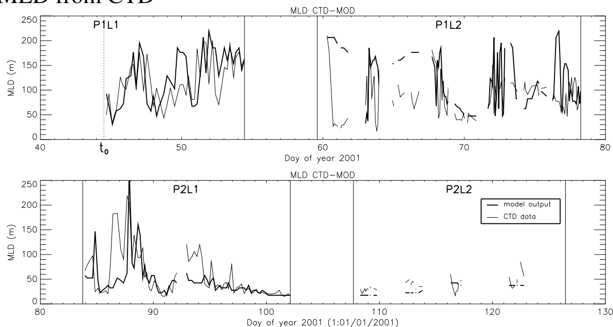
FIGURE 4.10 – Mixed layer depth (MLD) computed from CTD data and from model output during POMME1 and POMME2 following the ship track.
