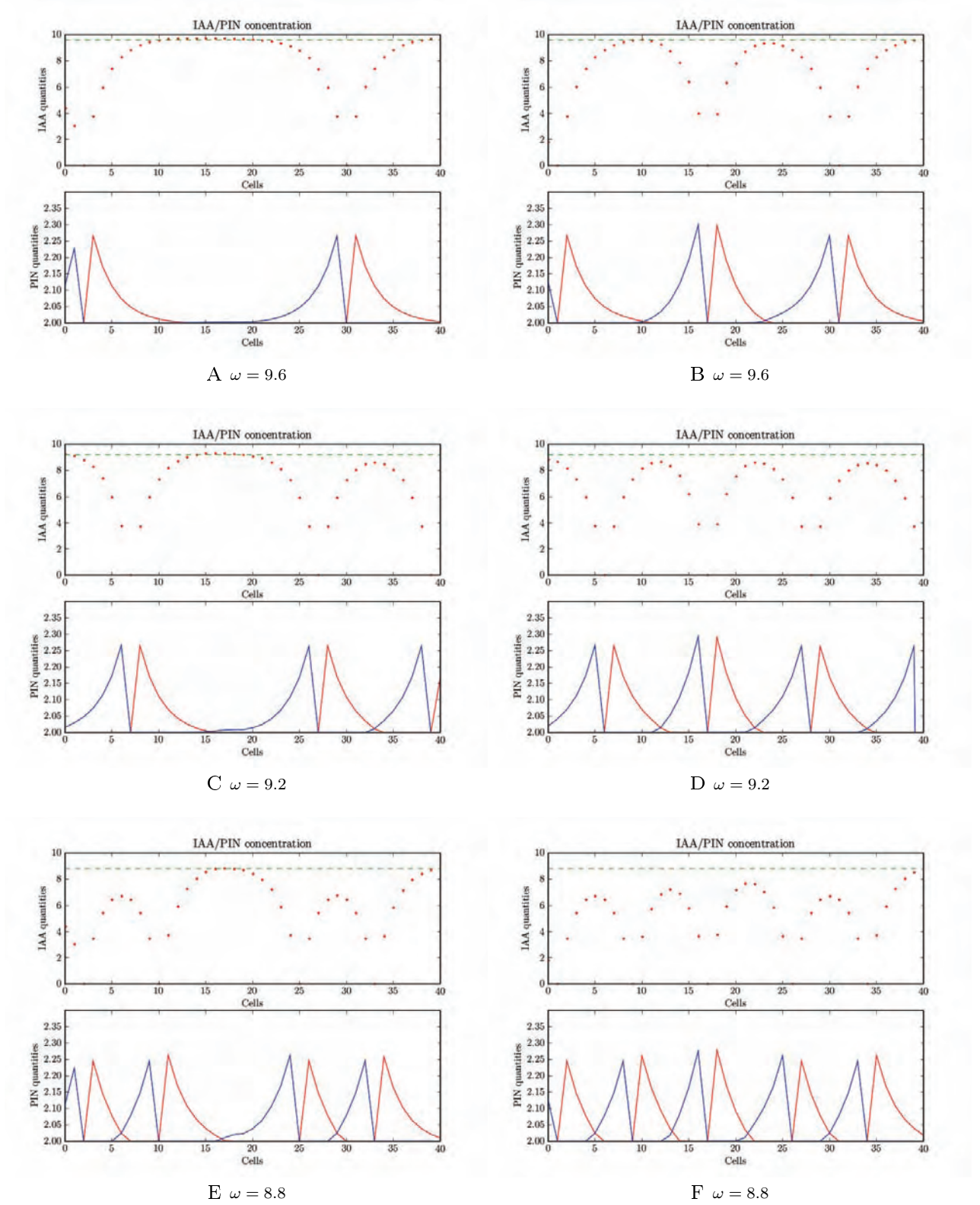
Fig. 4: Dynamic patterning with canalization. Figures 4A-4B, 4C-4D, 4E-4F present three simulations respectively with different thresholds \omega for primordium initiation. Figures 4A, 4C, 4E present the step just before primordium initiation for different models and Figures 4B, 4D, 4F present the step just after primordium initiation. The frequency of primordium initiation increases with a decrease of the initiation threshold \omega .
