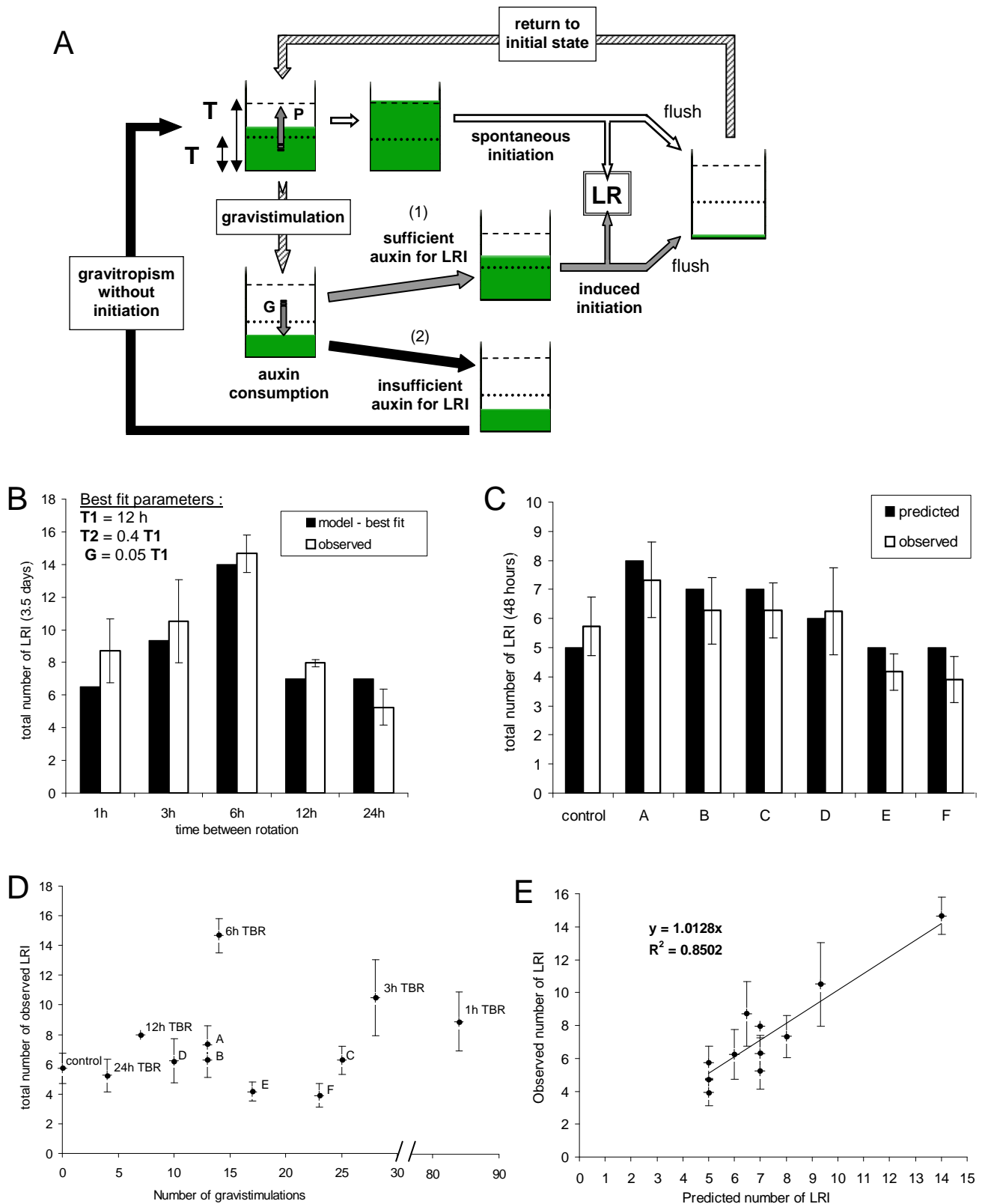
Figure 3. Model of lateral root initiation regulation. (A) Logical circuit of the model. Auxin accumulates with a production rate P , and when its level is above the threshold T1 a lateral root initiation (LRI) occurs. Initiations cause a flush of the auxin pool. Gravistimulations induce an auxin consumption ( G ) and an initiation if the remaining auxin level is higher than a second threshold T2 . (B) Comparison of observed LRI densities and of the best fit output of the logical model. The parameters corresponding to the best fit were determined by extensive automated parameters space exploration. (C) Evaluation of the predictive power of the logical model. The predicted LRI densities and the LRI densities observed for each gravistimulation treatment were compared ( n = 20 , see figure S4 for additional details on the treatments). The control is a non-gravistimulated seedlings lot grown in the same condition as the gravistimulated seedlings ( n = 20 ). (D) There is no relation between the number of gravistimulations and the number of LRI. Each point corresponds to one of the treatments presented in (B) or (C), as identified by the corresponding tag. TBR: time between rotations. (E) Number of observed LRI as a function of the predicted number of LRI. Each point corresponds to one of the treatments presented in (B) or (C). This graph shows that the values observed match closely the predicted value.
