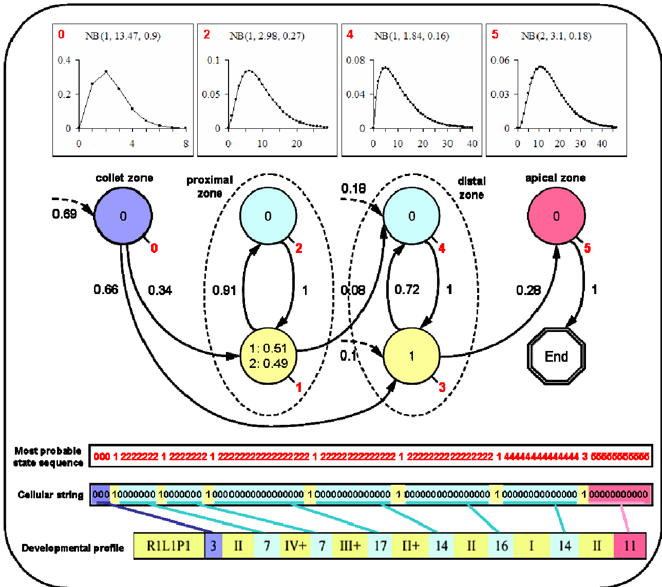
Figure 5. Statistical model of root development
