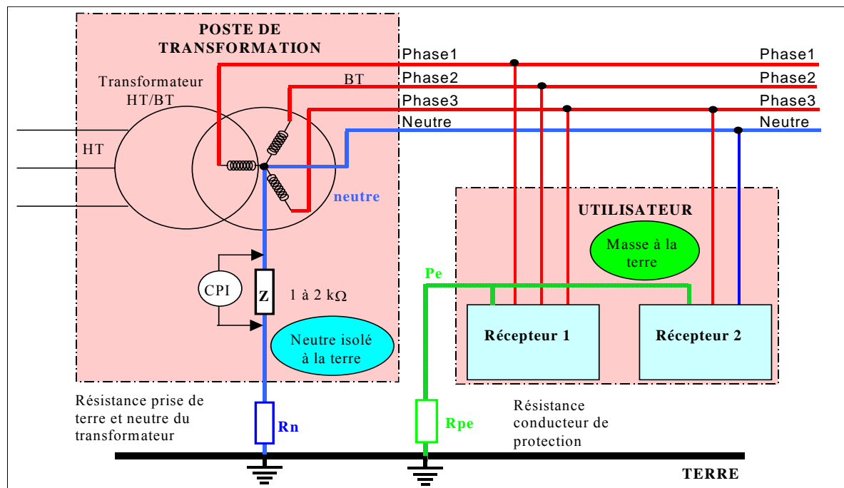
Figure 104 : Régime IT.
