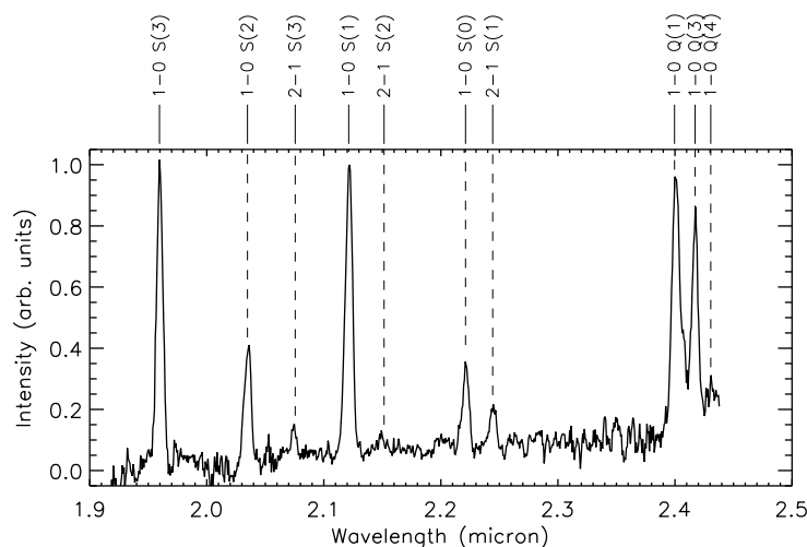
Figure 6.7: K-band spectrum of knot A, BHR137. Detected H_2 lines are marked. Intensity is in arbitrary units.
