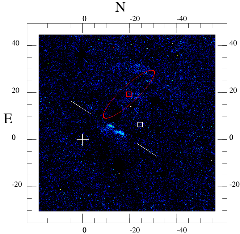
Figure 6.2: Finding chart for BHR137 showing continuum-subtracted H_2 emission from the v=1-0 S(1) line. The slit position is marked by the two white lines. The IRAS source is marked by the red rectangle and the error ellipse is shown. The white square shows the 1.3 mm-source (Reipurth et al. 1996). See also Fig. 1.13.
