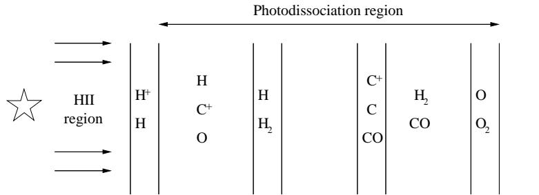
Figure 1.7: Schematic view of a PDR, showing the different zones surrounding an O or B star. Adapted from Hollenbach & Tielens (1999).
