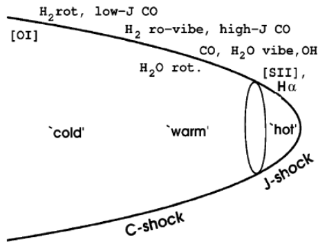
Figure 1.5: Schematic of a bow shock. The bow shock is dissociative at the tip. The locations where radiative coolants make their primary contributions are indicated. From Smith et al. (2003).
