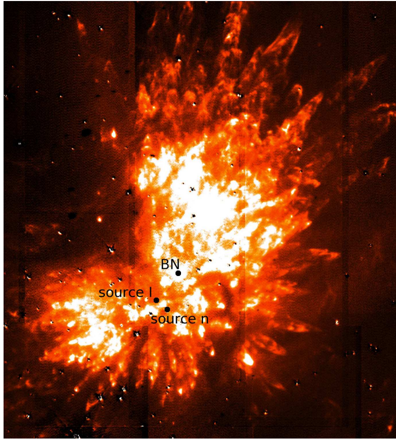
Figure 1.10: Structure of continuum-subtracted H_2 2.12 \mu\text{m} emission in OMC1. The positions of BN, radio source I and radio source n are marked. IRC2 is located \sim 1'' N of radio source I. The image was obtained with the Subaru Telescope.
