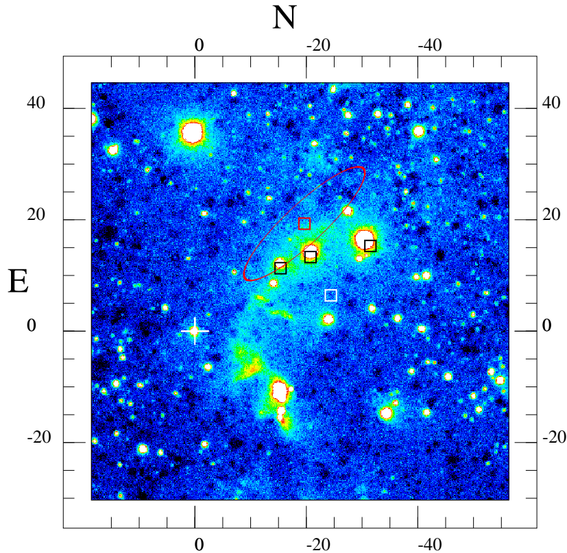
Figure 1.13: H_2 v=1-0 S(1) + continuum finding chart for the BHR137 region. The red box marks the location of the IRAS source with its associated error ellipse, the three black boxes show the YSOs (Santos et al. 1998) and the white box shows the location of the mm source (Reipurth et al. 1996).
