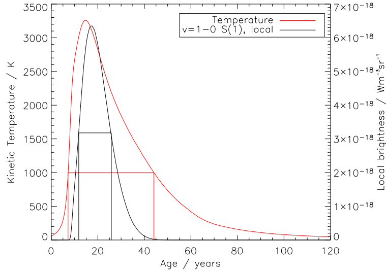
Figure 2.12: The three different definitions of shock age displayed for a C-type shock with preshock density 5 \times 10^5 \text{ cm}^{-3} , shock velocity 49 \text{ km s}^{-1} , initial ortho/para ratio 3.0 and b is 6.0. The kinetic temperature and \text{H}_2 v=1-0 S(1) local emissivity profiles are shown. The ordinate displays the steady-state timescale (age at 50 K; 120 years) and the red vertical lines display the age at 1000 K (37 years). The black vertical lines display the \text{H}_2 v=1-0 S(1) local emission FWHM (14 years) (Kristensen et al. 2007b).
