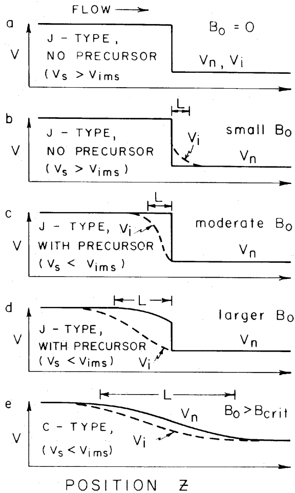
Figure 1.4: Evolution from a J-type shock to a C-type shock by increasing the magnetic field. In the top panel (a) there is no magnetic field, and the shock is a J-type shock. Increasing the magnetic field causes the origin of magnetic precursors, and when the magnetic field is larger than some critical value, the shock is a C-type shock. L is the typical length scale. Velocities are given in the restframe of the shock-front (Draine 1980).
