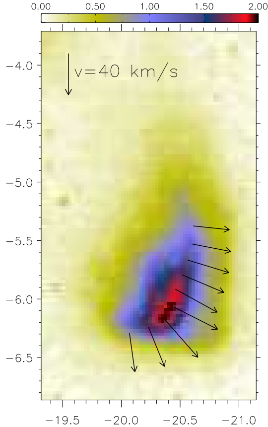
Figure 5.8: Velocity variations along the bow superposed on an image of the bow shock as observed in v=1-0 S(1). Coordinates and colour bar are as in Fig. 5.4. The lengths of the arrows are scaled with velocity and the arrow in the top left corner has a length corresponding to 40 \text{ km s}^{-1} .
