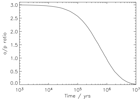
Figure 1.3: Ortho/para ratio as a function of time in a cold dark cloud (Kristensen et al. 2007a). See text for initial conditions.
