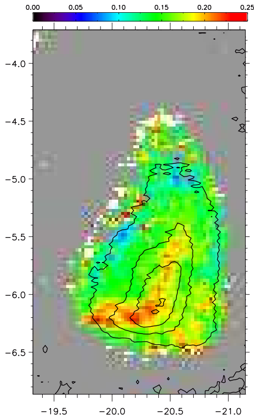
Figure 5.11: v=2-1 S(1) / v=1-0 S(1) line ratio in object 3. Coordinates are given with respect to TCC0016 and the colour bar is for the ratio. Contours are for v=1-0 S(1) absolute brightness. Contour levels are at 0.5, 1.0, 1.5 and 2.0 \times 10^{-5} \text{ W m}^{-2} \text{ sr}^{-1} .
