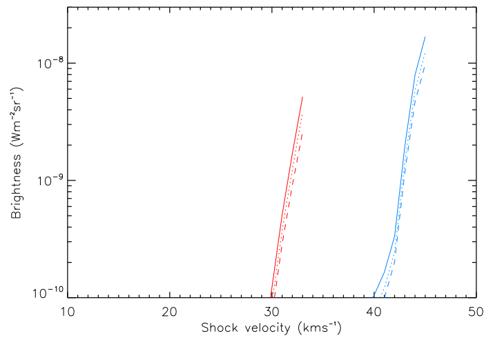
Figure 2.17: [\text{FeII}] emission in C-type shocks as a function of shock velocity. Linestyles are as above, Fig. 2.16. Brightness is displayed for a preshock density of 10^6 \text{ cm}^{-3} and b is 1.0 (red) and 3.0 (blue).
