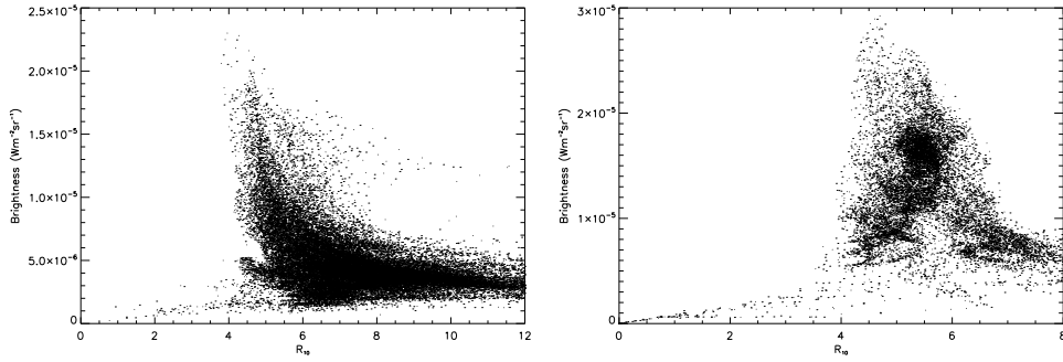
Figure 5.1: Brightness of the v=1-0 S(1) line vs. the line ratio, R_{10} in region West (left) and north (right). Data have been rebinned to a third of the original size, so the effective pixel size is 0''.081 , slightly lower than the resolution.
