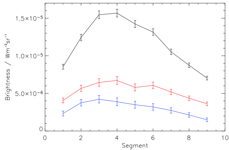
Figure 5.6: Brightness integrated over the FWHM along the bow for the three lines v=1-0 S(1) (black), v=1-0 S(0) (red) and v=2-1 S(1) (blue) in each segment. Error bars show 1\sigma uncertainties.
