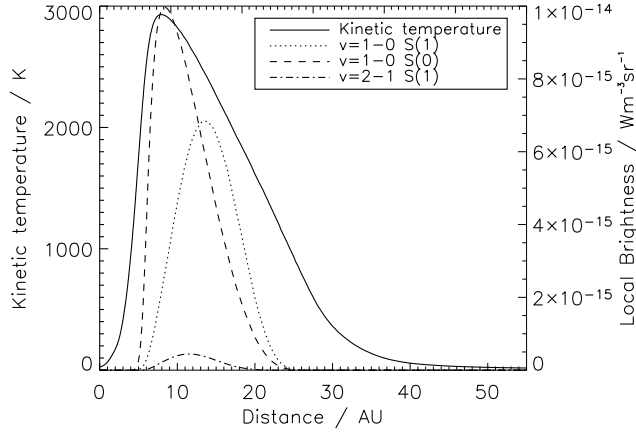
Figure 2.2: The temperature profile of a C-type shock with preshock density 10^6 \text{ cm}^{-3} , shock velocity 20 \text{ km s}^{-1} , initial ortho/para ratio 0.01 and b equal to 1. Also shown are local brightness profiles for the \text{H}_2 v=1-0 \text{ S}(0) , v=1-0 \text{ S}(1) and v=2-1 \text{ S}(1) lines. Zero distance is set to be the point at which the kinetic temperature starts to rise (Kristensen et al. 2007a).
