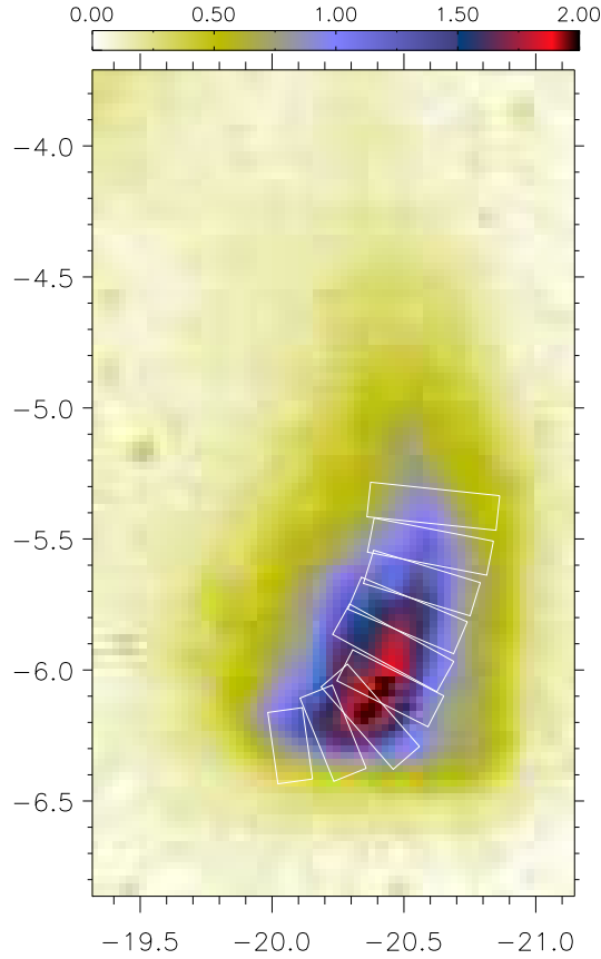
Figure 5.4: Location and extent of the 9 segments we have chosen to study overlaid on a map of continuum subtracted H_2 v=1-0 S(1) emission. Coordinates are relative to TCC0016 and the colorbar is given in units of 10^{-5} \text{ W m}^{-2} \text{ sr}^{-1} . The location of the shock is shown in Fig. 5.3. We have labelled segments 1 and 9 for easy identification. The arrow shows a position angle of 235^\circ and the length corresponds to 150 AU.
