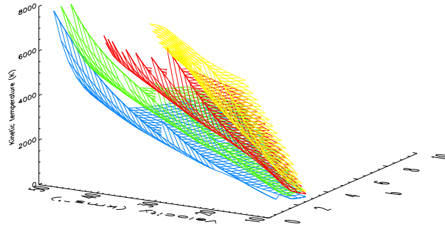
Figure 2.4: The kinetic temperature in C-type shocks as a function of shock velocity and magnetic scaling factor, b . Different sheets corresponds to different preshock densities. Blue: 10^4 \text{ cm}^{-3} , green: 10^5 \text{ cm}^{-3} , red: 10^6 \text{ cm}^{-3} and yellow: 10^7 \text{ cm}^{-3} .
