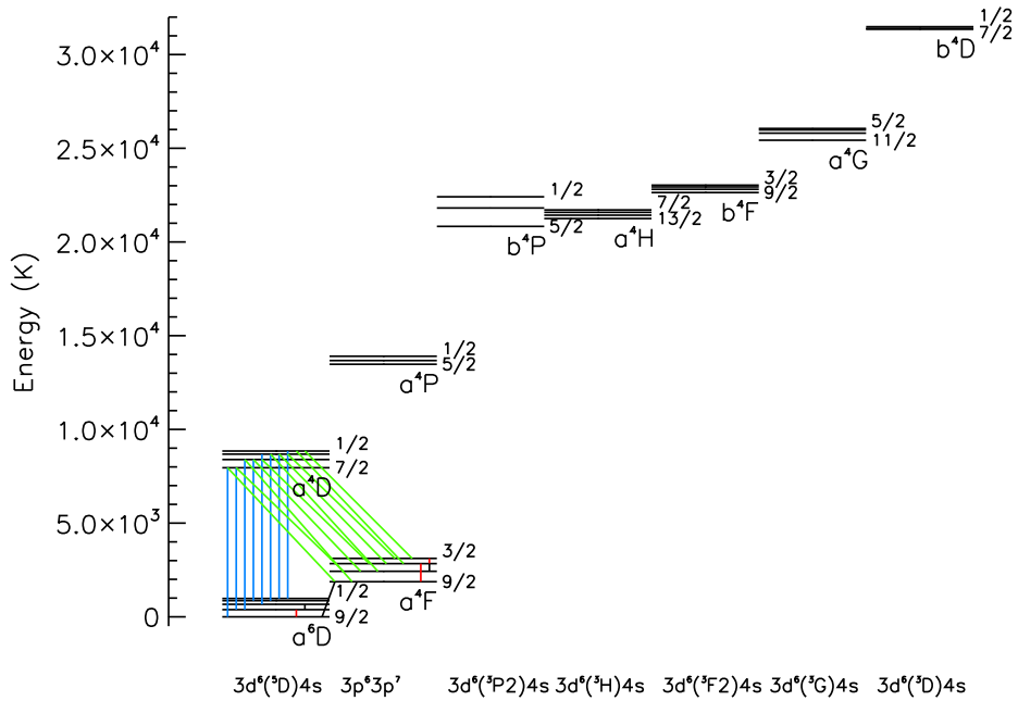
Figure 2.1: Grotrian diagram showing the levels of \text{Fe}^+ for which populations are calculated in the models. On the abscissa the electronic configuration is shown. We display levels according to terms (2S+1)L_J where the range of J is shown for each level. Line brightness for eight transitions between the a^4D and a^6D terms (blue), ten transitions between the a^4D and a^4F terms and three fine-structure transitions (red) are calculated. Furthermore three transitions observed by Spitzer (Neufeld et al. 2007) are shown (black).
