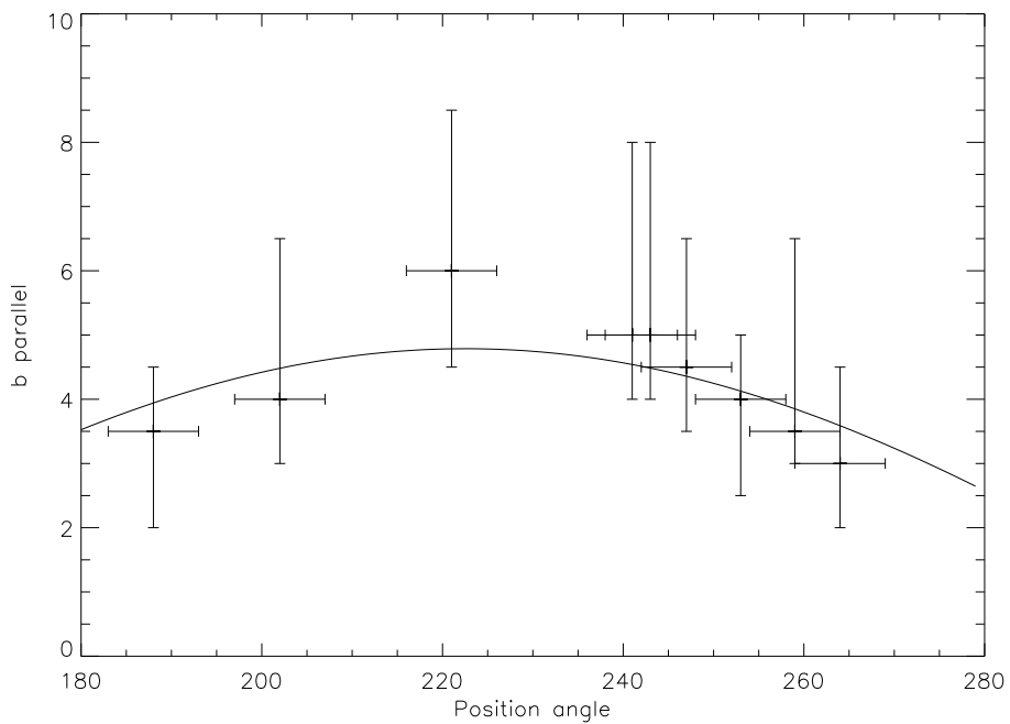
Figure 5.10: The magnetic scaling factor b , as a function of position angle. The curve shows the best-fit solution to Eq. 5.2.2.
