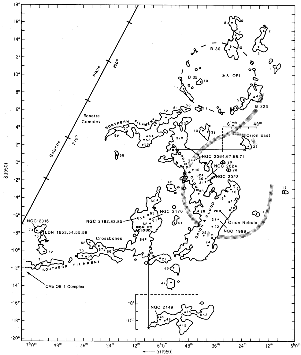
Figure 1.8: The Giant Orion Molecular Cloud as observed through CO emission. The Orion Nebula is shown at co-ordinates -5^\circ 32' , 5^h 25^m (Maddalena et al. 1986).
