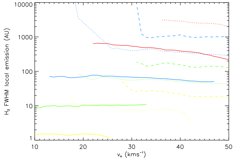
Figure 2.15: Width of C-type shocks as FWHM of local \text{H}_2 v=1-0 S(1) emission as a function of shock velocity. Colours and line styles are as above in Fig. 2.13.
