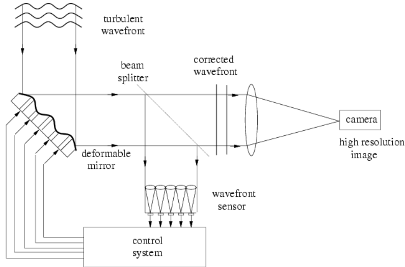
Figure 3.1: Schematic view of an adaptive optics system.
