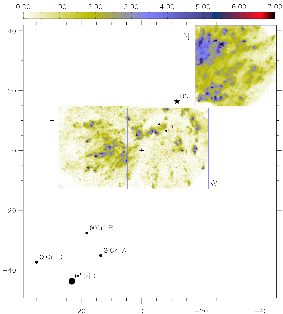
Figure 3.4: Finding chart for VLT-NACO/FP observations. Data show continuum-subtracted H_2 emission in the v=1-0 S(0) line at 2.23\mu\text{m} . The colourbar is in units of 10^{-6} \text{ W m}^{-2} \text{ sr}^{-1} . The positions of the Trapezium stars are marked. Axes are in arcseconds and offsets are given with respect to TCC0016 marked by a cross (+). Our observed fields are outlined in blue boxes, each with a size of 27'' \times 27'' . The position of radio sources I and n are also given as well as BN (Menten & Reid 1995).
