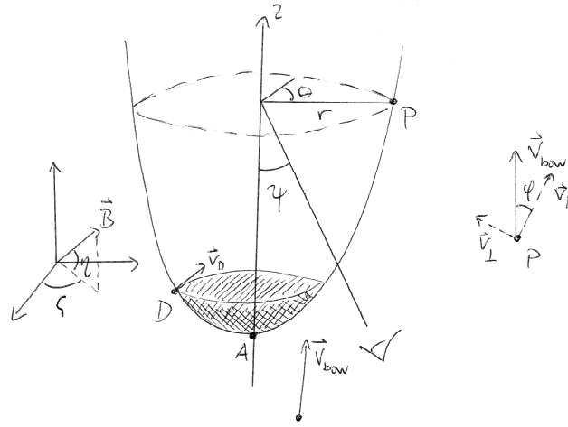
Figure 2.19: Schematic presentation of a bow shock from the reference frame of the shock. The ambient gas is streaming past the shock at a velocity, v_s .
