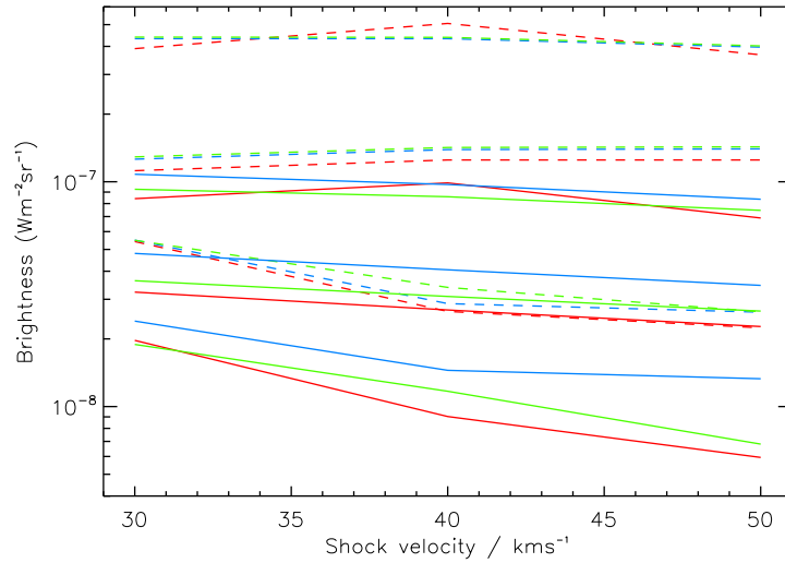
Figure 2.11: Effects of H_2 reformation in the postshock zone of dissociative J-type shocks. The brightness of the v=1-0 S(1) transition (dashed line) and the v=2-1 S(1) transition (full line) are shown. Formation scenario 1 is displayed in red, scenario 2 in blue and scenario 3 in green (see text for explanation of formation scenarios). Preshock densities are 10^3 , 10^4 and 10^5 \text{cm}^{-3} , where lower preshock density results in lower brightness.
