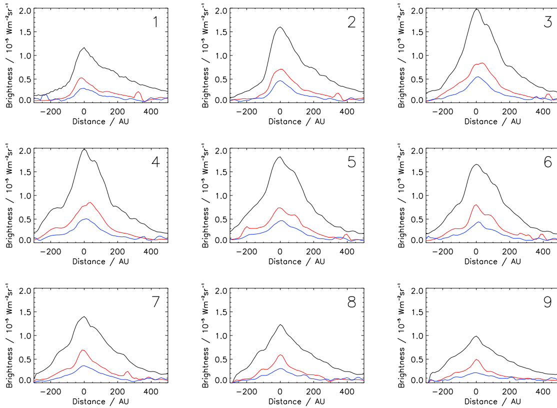
Figure 5.5: Intensity cuts through the bow of the H_2 v=1-0 S(1) (black), v=1-0 S(0) (red) and v=2-1 S(1) (blue) lines in each segment. Distances are given in AU and the zero point is the location of the brightness maximum. This point does not change significantly for the other two lines. Negative distances indicate that this brightness is outside the bow, while positive distances are inside. The number in each profile refers to the segment number (see Fig. 5.4).
