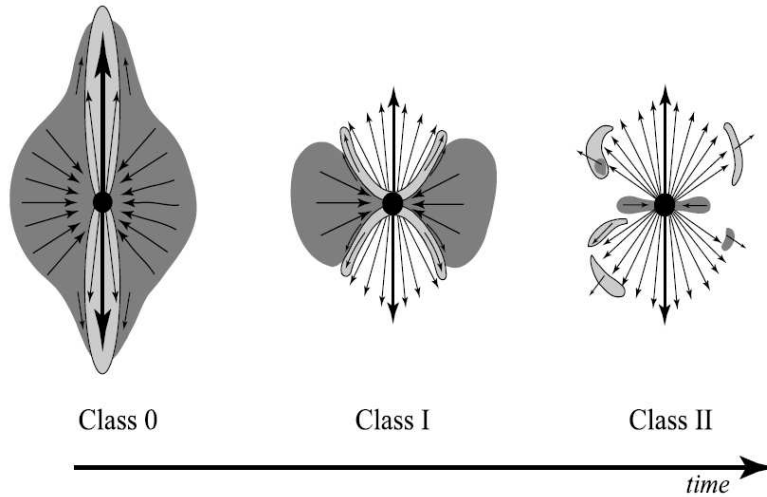
Figure 1.1: Differences between outflows from class 0, I and II sources. In class 0 sources the outflow is very collimated, whereas in class II sources the outflow resembles a stellar wind. From Arce & Sargent (2006).
