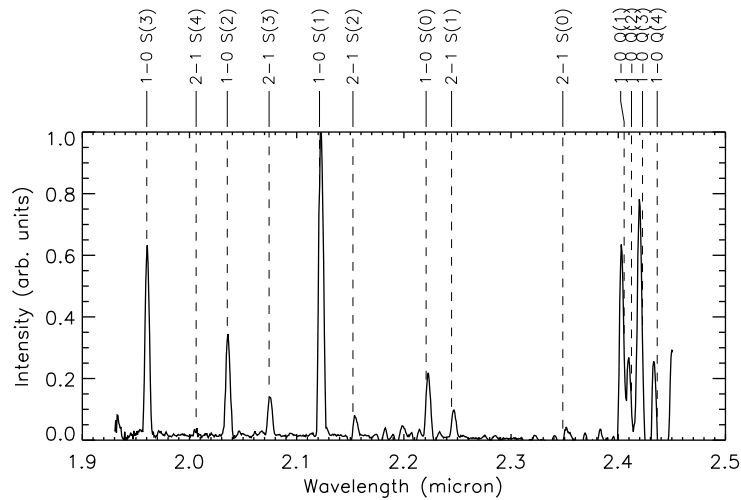
Figure 6.4: K -band spectrum of knot 1, BHR71. Detected H_2 lines are marked. Intensity is in arbitrary units.
