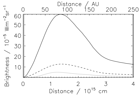
Figure 5.16: Brightness profiles relative to each other: v=1-0 S(1) (full line), v=1-0 S(0) (dashed line) and v=2-1 S(1) (dotted line). These brightness cuts are made along the grey line indicated in Fig. 5.13 going through the apex.
