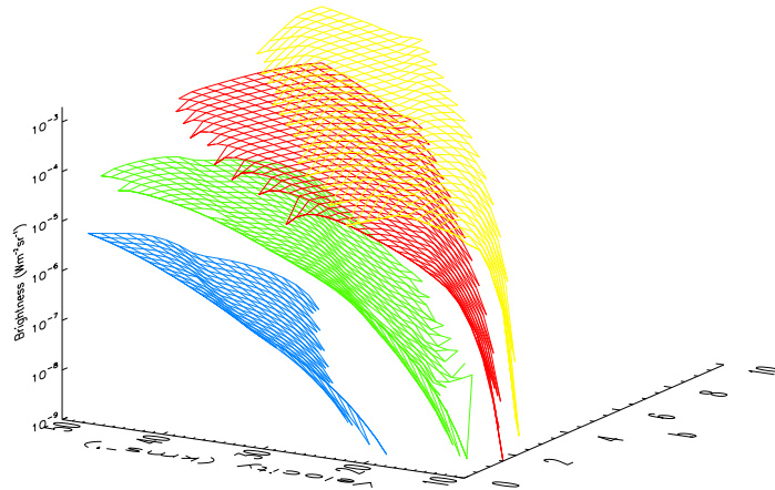
Figure 2.7: The \text{H}_2 v=1-0 S(1) brightness in C-type shocks as a function of shock velocity and b for four different preshock densities, 10^4 \text{ cm}^{-3} (blue), 10^5 \text{ cm}^{-3} (green), 10^6 \text{ cm}^{-3} (red) and 10^7 \text{ cm}^{-3} (yellow).
