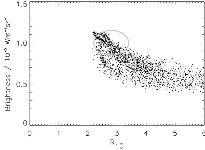
Figure 4.6: A plot of brightness in the v=1-0 S(1) line for object 1 similar to Fig. 4.2 for object 1, but without spatial rebinning. The oblong encloses those data used for comparison with models.
