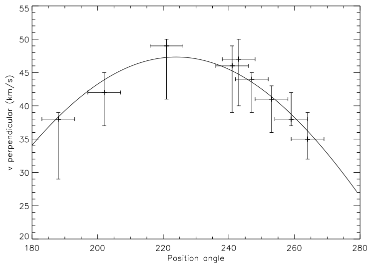
Figure 5.9: The shock velocity perpendicular to the bow, as a function of position angle. The curve shows the best-fit solution to Eqn. 5.2.1.
