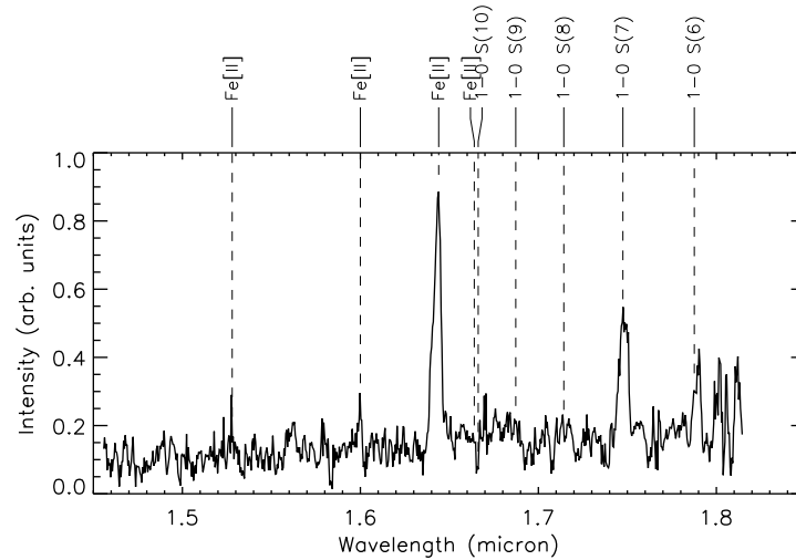
Figure 6.8: H -band spectrum of knot A, BHR137. We show the location of several H_2 and [FeII] lines. Intensity is in arbitrary units.
