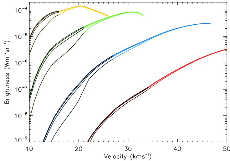
Figure 2.10: As in Fig. 2.9 but for C-type shocks. The black section of each line indicate where the kinetic temperature is less than 3200 K and there is ongoing para-to-ortho-interconversion. b is equal to 1.
