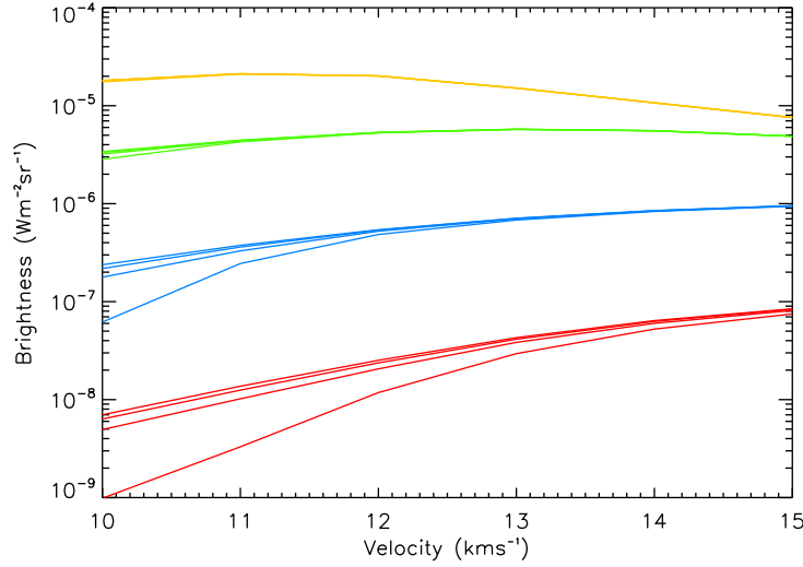
Figure 2.9: The \text{H}_2 v=1-0 S(1) brightness in J-type shocks for different preshock densities, 10^4 \text{ cm}^{-3} (red), 10^5 \text{ cm}^{-3} (blue), 10^6 \text{ cm}^{-3} (green) and 10^7 \text{ cm}^{-3} (yellow) and different initial ortho/para ratios. For each value of the preshock density, the lower the line the lower the value of the initial ortho/para ratio.
