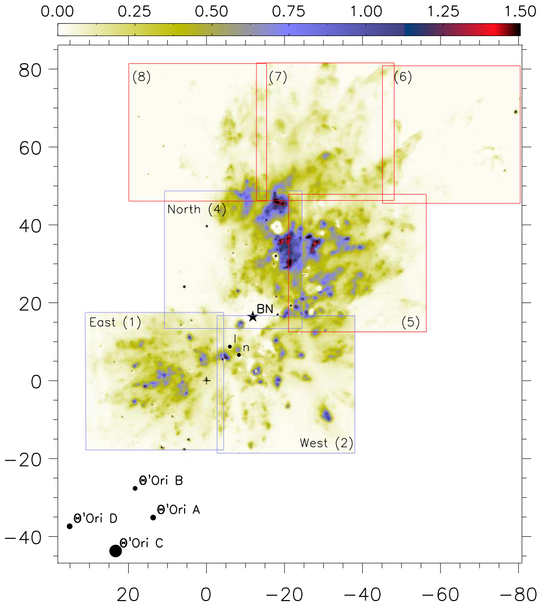
Figure 3.2: Finding chart of CFHT observations. Data show continuum-subtracted H_2 emission in the v=1-0 S(1) line at 2.12\mu\text{m} . The colourbar is in units of 10^{-5} \text{ W m}^{-2} \text{ sr}^{-1} . The positions of the Trapezium stars are marked. Axes are in arcseconds and offsets are given with respect to TCC0016 marked by a cross (+). The position of radio sources I and n are also given as well as BN (Menten & Reid 1995). Boxes indicate the location of our 7 fields of view, each measuring 36'' \times 36'' . Blue boxes marks fields which have been used in the data-analysis while red fields have not (see text for further details). Numbers in parentheses are the region numbers.
