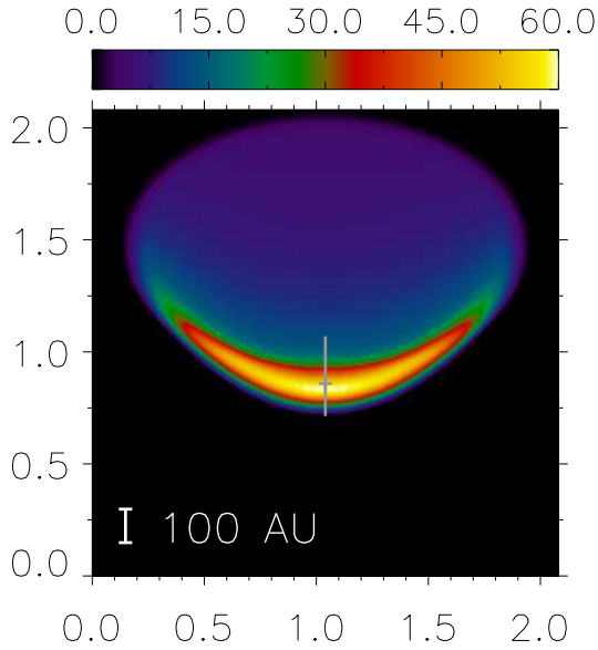
Figure 5.13: 3D model results for object 3 shown for the v=1-0 S(1) transition. The inclination with respect to the line of sight is 50^\circ . The colour bar is in units of 10^{-5} \text{ W m}^{-2} \text{ sr}^{-1} . Axes are in 10^{16} \text{ cm} . The cross indicate the location of the apex.
