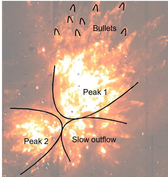
Figure 1.11: Schematic showing the distinct outflows in the OMC1, BN-KL region. The bullets, the bipolar outflow and the slower outflow are illustrated (see text for descriptions). The background image shows continuum-subtracted v=1-0 S(1) emission; from the Subaru Telescope.
