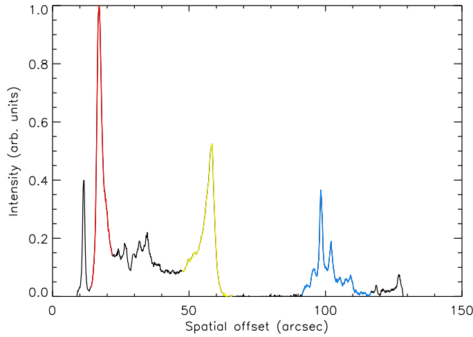
Figure 6.3: Spatial distribution of H 2 v=1-0 S(1) emission in BHR71 as observed through the centre slit in Fig. 6.1. In red is HH321A (knot 1), yellow shows emission associated with IRS 1 (knot 2) and in blue is emission located north of IRS 1 (knot 3). The abscissa is in arcseconds with the zero point set arbitrarily. The ordinate is for v=1-0 S(1) emission in arbitrary units.
