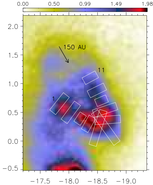
Figure 5.17: Continuum-subtracted image of object 1 shown in v=1-0 S(1) emission. Boxes show location and extent of the 11 segments. Segments 1 and 11 are marked for identification. The arrow has a position angle of 220^\circ and a length corresponding to 150 AU. Coordinates are relative to TCC0016 and the colour bar is for brightness in units of 10^{-5} \text{ W m}^{-2} \text{ sr}^{-1} .
