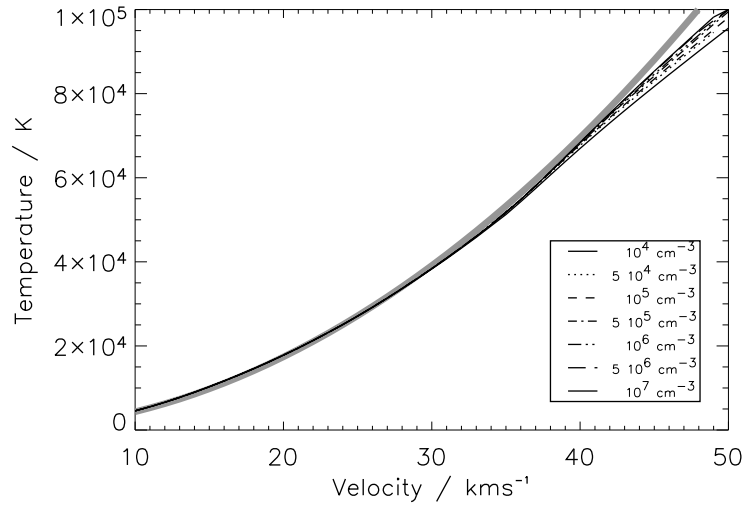
Figure 2.3: The kinetic temperature in J-type shocks as a function of shock velocity. The gray line shows the prediction from Eq. 2.2.1.
