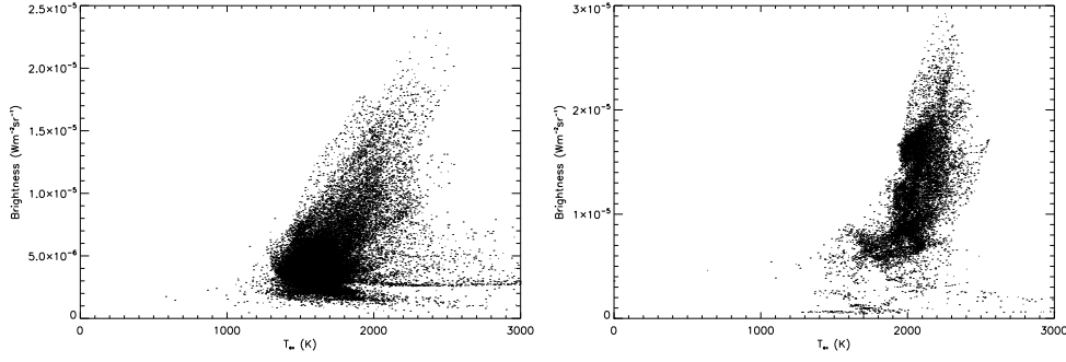
Figure 5.2: Brightness of the v=1-0 S(1) line vs. excitation temperature for region West (left) and North (right). Data have been rebinned to a third of the original size, so the effective pixel size is 0''.081 , slightly lower than the resolution.
