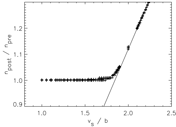
Figure 2.18: The compression factor in C-type shocks as a function of v_s/b . Each cross corresponds to a model result. The line corresponds to Eqn. 2.2.10.
