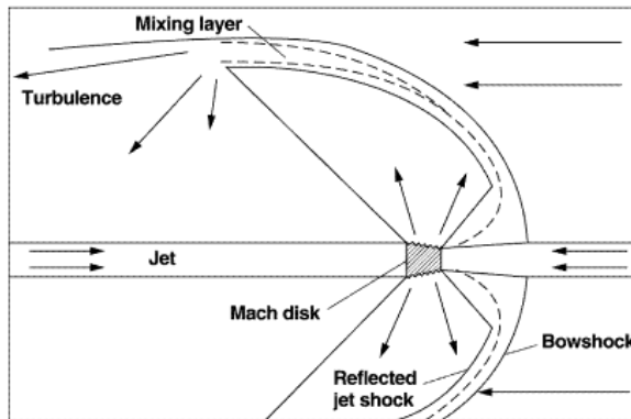
Figure 1.6: Detailed view of the internal shock structures in a bow shock as seen from the reference frame of the internal working surface (Mach disk). The jet and ambient material are both impinging on the Mach disk in the reference frame of the shock. From Hollenbach (1997).
