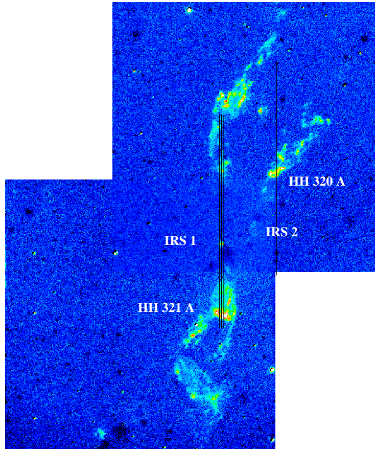
Figure 6.1: Finding chart for BHR71 showing continuum-subtracted H 2 emission from the v=1-0 S(1) line. The four different slit positions are marked with black lines. Each image measures 152'' \times 152'' and North is up, East is left.
