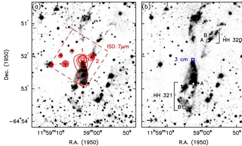
Figure 1.12: Finding chart for the BHR71 region. (a) Image shows K' -band emission with ISO LW2 contours ( 5.0\text{--}8.5\ \mu\text{m} ) showing the locations of IRS1 and 2. (b) \text{H}_2 v=1-0 S(1) emission + continuum. The locations of HH320A/B and HH321A/B are marked with plus signs.
