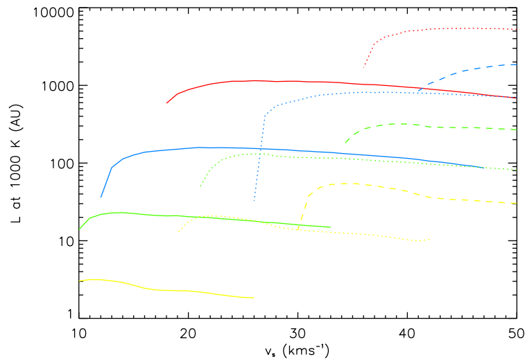
Figure 2.14: Width of C-type shocks at 1000 K as a function of shock velocity. Colours and line styles are as above in Fig. 2.13.
