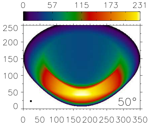
Figure 5.15: The number of points with T > 1000 K for the bow shock model in Fig. 5.13. Axes are in pixels. The projection is smoothed by a 5 \times 5 pixels moving boxcar average. The size of the boxcar is indicated by the small black square in the lower left corner. The colour bar represents the number of points with T > 1000 K.
