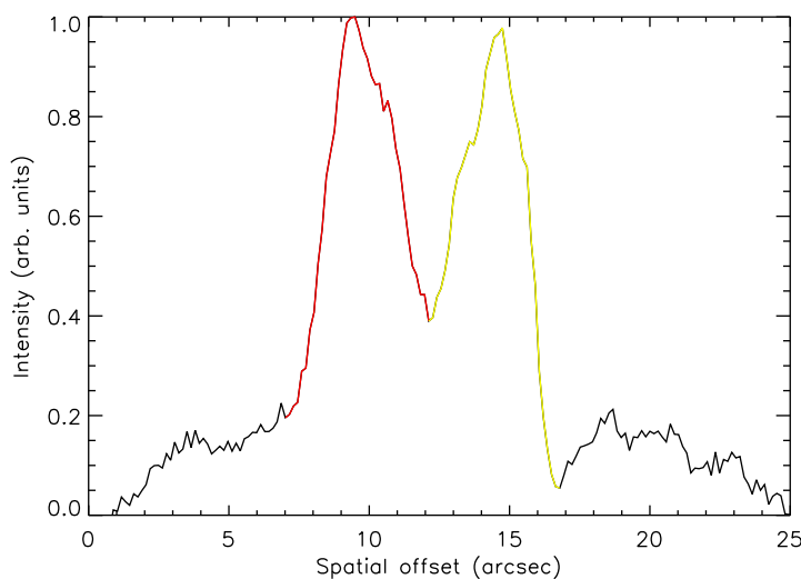
Figure 6.6: Spatial distribution of H_2 v=1-0 S(1) emission in BHR137. In red is knot A, yellow shows emission associated with knot B. The abscissa is in arcseconds. The zero point has been set arbitrarily. The ordinate is for v=1-0 S(1) emission in arbitrary units.
