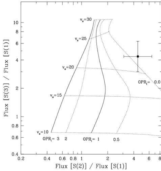
Figure 2.8: Diagnostic diagram of pure rotational H_2 emission. Model predictions are shown for a C-type shock model with preshock density 5 \times 10^5 \text{ cm}^{-3} as a function of shock velocity and initial ortho/para ratio (OPR). Predictions are from (Timmermann 1998). Taken from Neufeld et al. (1998).
