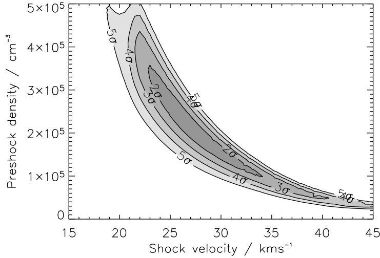
Figure 4.3: The confidence intervals of class A1. The contours are given at intervals of \sigma from 2\sigma to 5\sigma . The models used to make this plot all have an initial ortho/para ratio of 0.01 and b=1.0 . See Sect. 4.4.2 for further description.
