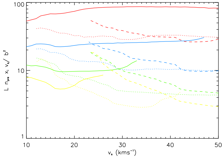
Figure 2.13: ( L n_{\text{pre}} x_i v_s / b^2 ) as a function of v_s (see Eqn. 2.2.7). Results are displayed for four different preshock densities, 10^4 \text{ cm}^{-3} (red), 10^5 \text{ cm}^{-3} (blue), 10^6 \text{ cm}^{-3} (green) and 10^7 \text{ cm}^{-3} (yellow) and three different values of b , b=1.0 (full line), b=5.0 (dotted line) and b=10.0 (dashed line).
