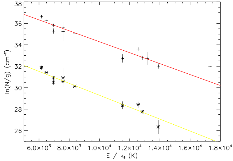
Figure 6.9: Boltzmann diagram for the two knots of emission identified. Red is knot A, yellow is knot B. Vertical lines show 1\sigma errors. The lines show the best fit through the data. The corresponding excitation temperature is given in Table 6.2. Results for knot B have been displaced vertically by 5.
