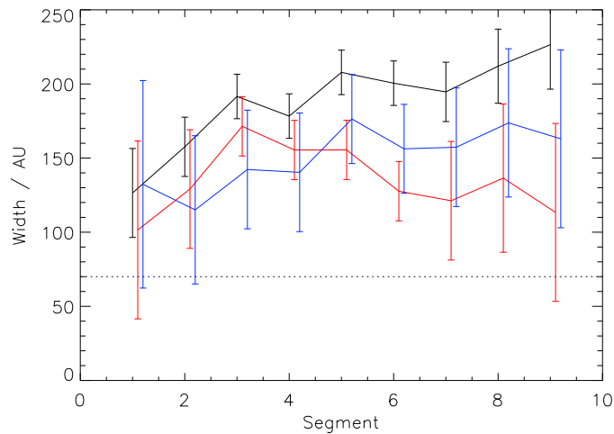
Figure 5.7: The FWHM of H_2 emission for the three lines v=1-0 S(1) (black), v=1-0 S(0) (red) and v=2-1 S(1) (blue) in each segment. The dotted line at 70 AU shows the spatial resolution (see text). Errorbars show 1\sigma uncertainties. Points representing v=1-0 S(0) and v=2-1 S(1) widths have been shifted horizontally by 0.1 and 0.2 respectively so as to clearly separate the error bars.
