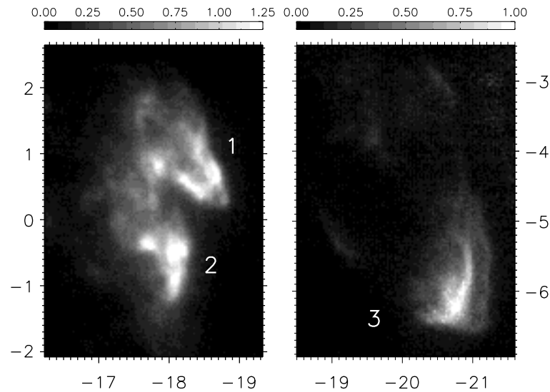
Figure 4.5: ESO-VLT NACO images of three objects where the bowshocks have been resolved. The greyscale bar is in units of 10^{-5} \text{ W m}^{-2} \text{ sr}^{-1} (Lacombe et al. 2004). Coordinates are as in Fig. 3.2.
