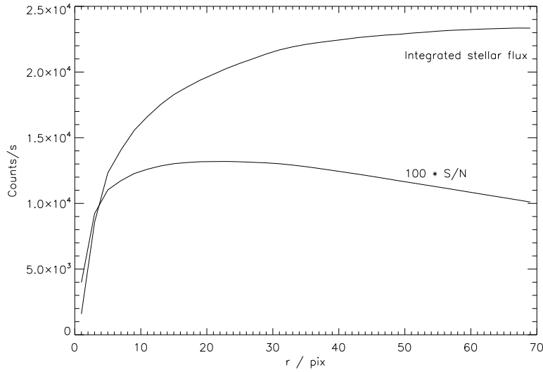
Figure 3.5: Aperture photometry of the calibration star HR1950. The total count rate within radius r is shown as well as the S/N ratio. The latter has been multiplied by 100. The S/N ratio peaks at a radius of \sim 23 pixels.
