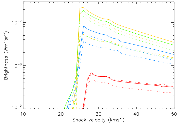
Figure 2.16: [\text{FeII}] emission in J-type shocks as a function of shock velocity. Brightness is shown for the transitions at 1.257 \mu\text{m} (full line), 1.644 \mu\text{m} (dotted line) and 17.936 \mu\text{m} (dashed line). Brightness is displayed for four different preshock densities: 10^4 \text{ cm}^{-3} (red), 10^5 \text{ cm}^{-3} (blue), 10^6 \text{ cm}^{-3} (green) and 10^7 \text{ cm}^{-3} (yellow).
