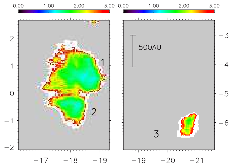
Figure 4.4: Map showing \phi_{10} in objects 1, 2 and 3 identified in Fig. 4.5. The area in grey represents regions in which emission is below specified signal levels (see text). The colour bar is for \phi_{10} and coordinates are in arcsec and relative to TCC0016 (see Fig. 3.2).
