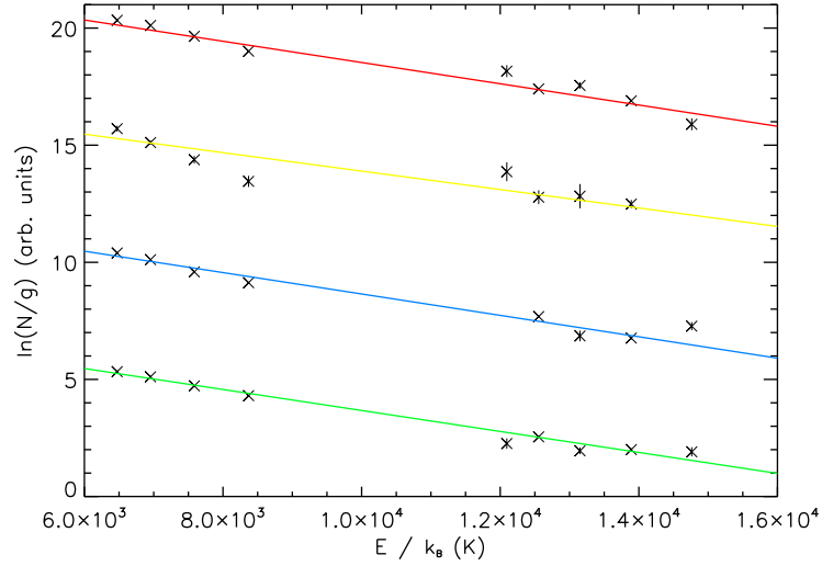
Figure 6.5: Boltzmann diagram for the four knots of emission identified. Red is knot 1 (HH321A), yellow is knot 2, blue is knot 3 and green is knot 4 (HH320A). 1\sigma error bars are shown as vertical lines. The lines show the best fit through the data. The corresponding excitation temperature is given in Table 6.1. Results have been displaced vertically by 5 so as to better show them.
