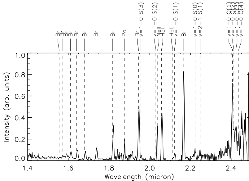
Figure 7.2: Example of H- and K-band spectrum of N159-5. Units of intensity are arbitrary. Identified lines are marked. Br indicate the Brackett series and Pa is Paschen \alpha .
