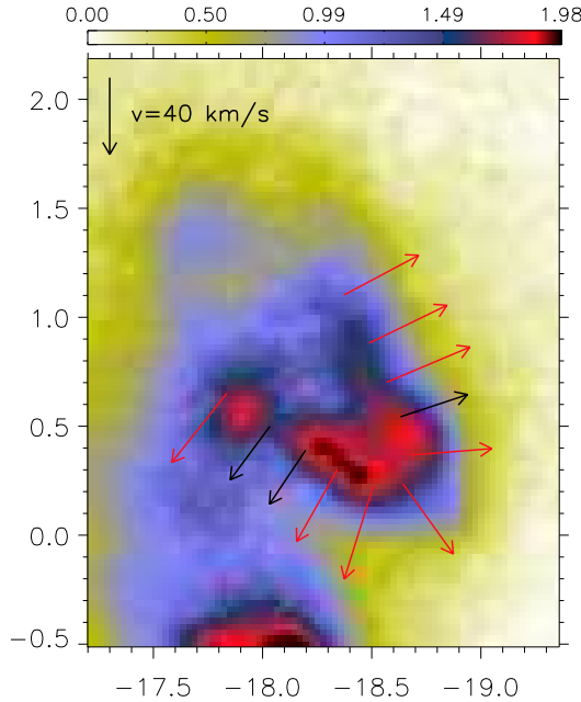
Figure 5.18: Velocity variations along the bow superposed on an image of object 1 as observed in v=1-0 S(1). Coordinates and colour bar are as in Fig. 5.17. The lengths of the arrows are scaled with velocity and the arrow in the top left corner has a length corresponding to 40 \text{ km s}^{-1} . Red arrows indicate a preshock density of 5 \times 10^5 \text{ cm}^{-3} while black arrows represent 10^6 \text{ cm}^{-3} .
