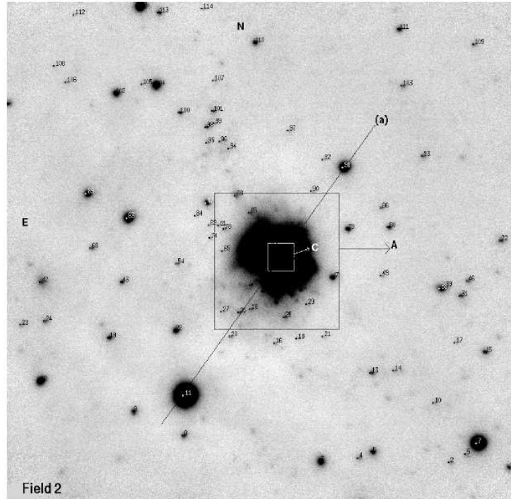
Figure 7.1: Finding chart for N159-5 showing K_s band emission obtained with the S27 camera. Stars detected are marked with numbers. The inset A ( 6' \times 6' ) contains the HEB N159-5. The small inset C ( 1' .34 \times 1' .34 ) contains the central star #2-55. The location of the slit (a) used in the spectroscopic mode is indicated by a solid line. Total field size is 26' .9 \times 23' .8 corresponding to 7 \text{ pc} \times 6 \text{ pc} .
