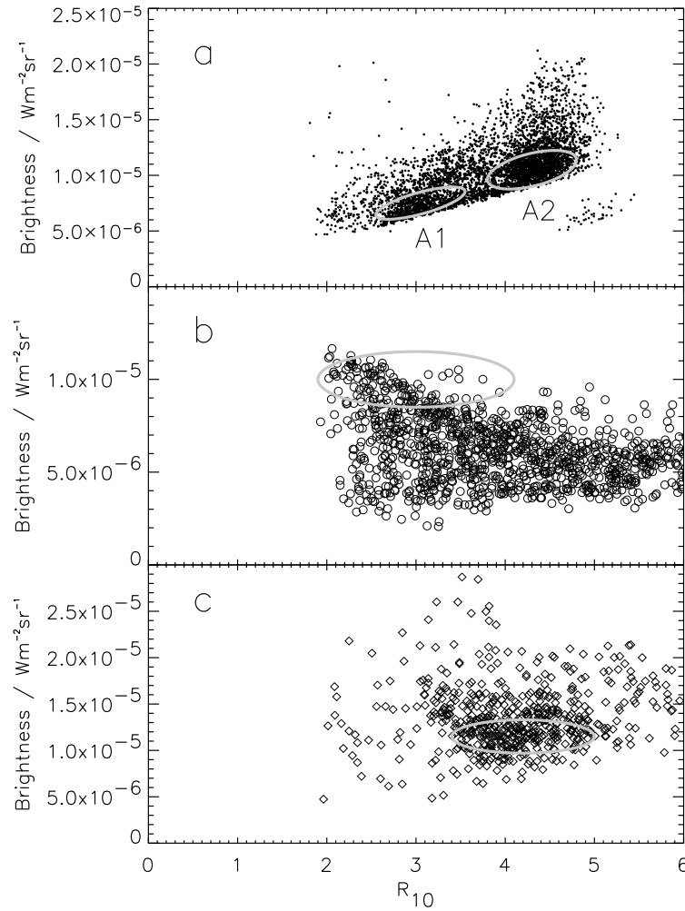
Figure 4.2: a : Region North: brightness of \nu=1-0 S(1) vs. the line ratio R_{10} . b : Region West : similarly for the blueshifted clumps in this zone. c : Region East. All data have been rebinned to 500 \times 500 pixels from the original field size of 2000 \times 2000 pixels. The effective pixel size becomes 0''.14 or 3 times better than the resolution. The grey oblongs identify those parts of the data whose characteristics are given in Table 4.1.
