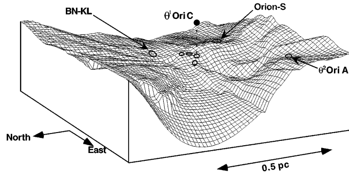
Figure 1.9: Three-dimensional image showing the surface described by the main ionization front on OMC1. \theta^1 Ori C is located 0.25 pc above the ionization front (O’Dell 2001).
