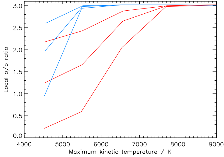
Figure 2.6: The H_2 ortho/para ratio as function of the maximum kinetic temperature reached in J-type shocks. Results are displayed for preshock densities of 10^4 \text{ cm}^{-3} (red) and 10^5 \text{ cm}^{-3} (blue) and for initial ortho/para ratios of 0.01, 1.0 and 2.0.
