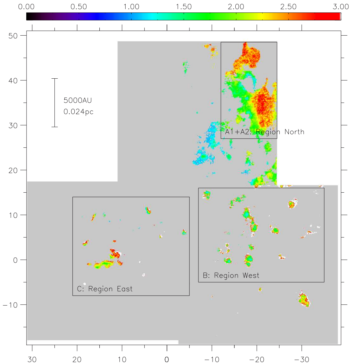
Figure 4.1: A map of the approximate ortho/para ratio, \phi_{10} , calculated from v=1-0 S(0) and S(1) emission, for the field identified in Fig. 3.2 estimated using Eqn. 4.1.5. The area in grey represents regions in which emission is below specified signal levels (see text). The colour bar is for \phi_{10} . Coordinates are relative to TCC0016 as in Fig. 3.2. The absolute coordinates of TCC0016 are 05^{\text{h}}35^{\text{m}}14.91, -05^{\circ}22'39'.31 (J2000). Original images have been smoothed using a boxcar average over 7 \times 7 pixels. The three large squares delineated by grey borders are named East, West and North, as illustrated in Fig. 3.2. The black rectangles, A1+A2, B and C, delineate regions which have been chosen for special study.
