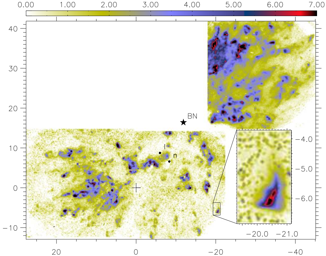
Figure 5.3: Finding chart for the bow shock we analyse with our 2D model. The map shows the VLT observations of continuum-subtracted H_2 emission in the v=1-0 S(0) line at 2.23 \mu\text{m} . The colourbar is in units of 10^{-6} \text{ W m}^{-2} \text{ sr}^{-1} . Axes are in arcseconds and offsets are given with respect to TCC0016. The box, which is magnified in the inset, shows the bow shock we are analysing.
