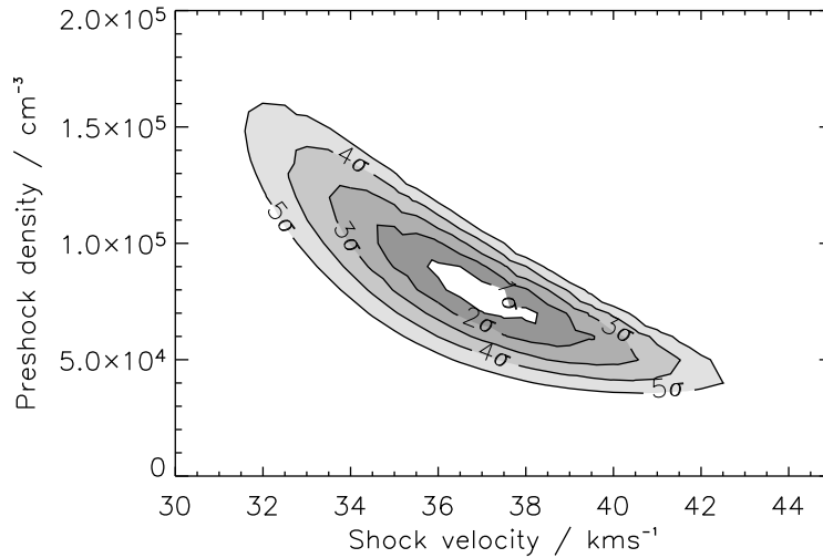
Figure 4.7: Confidence intervals for object 2. Model parameters are initial ortho/para=0.01 and b=1.0 .
