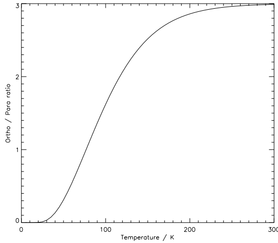
Figure 1.2: LSE ortho/para ratio as a function of kinetic temperature. For temperatures greater than \sim 300 K the ortho/para ratio is 3, while it is \sim 0 for temperatures lower than 20 K.
