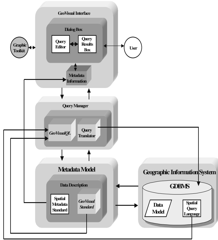
Figure 2.3 - GeoVisual Framework
