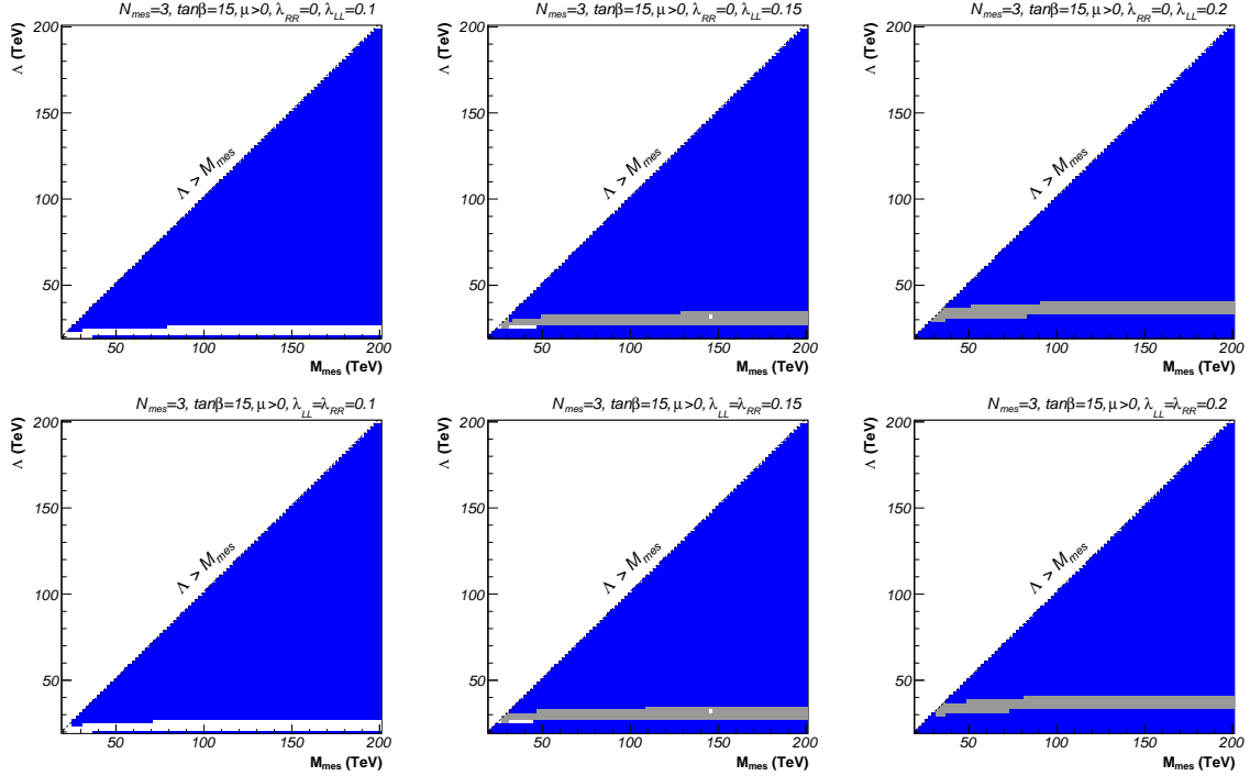
Figure 2.11: Same as Fig. 2.10 for N_{\text{mes}} = 3 , \tan\beta = 15 , and \mu > 0 .
