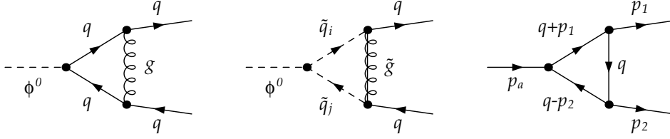
Figure C.4: Feynman diagrams for the gluon (left) and gluino (centre) correction to the Higgs-quark-quark vertex and generic diagram (right) indicating the notation for masses and momenta.
