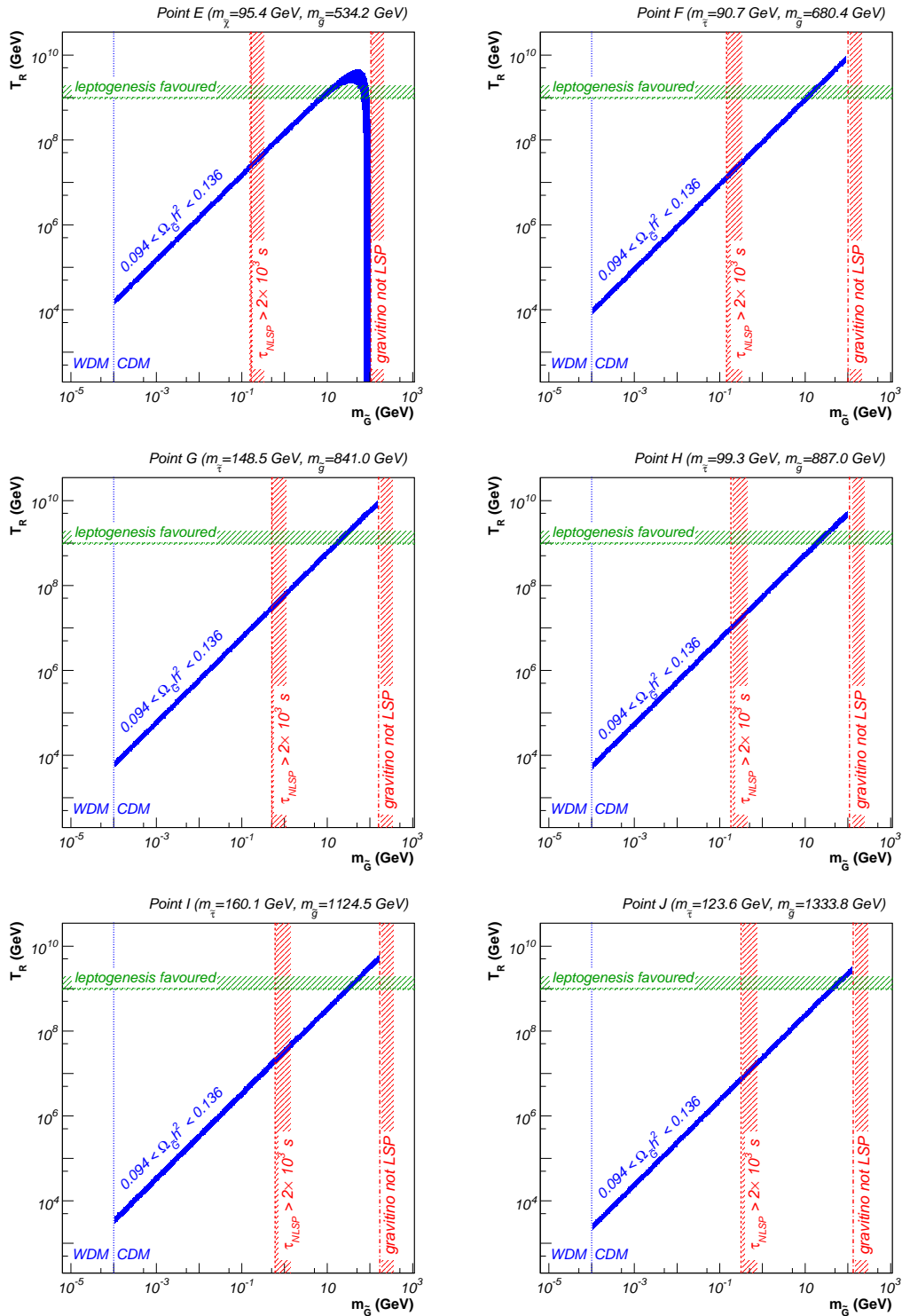
Figure 2.22: The cosmologically favoured regions in the m_{\tilde{G}}-T_R plane for our benchmark scenarios E, F, G, H, I, and J with respect to WMAP data (blue), the NLSP lifetime (vertical red line), and leptogenesis (horizontal green line).
