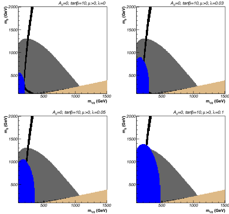
Figure 2.2: The m_0 - m_{1/2} planes for \tan \beta = 10 , A_0 = 0 , \mu > 0 , and \lambda_{LL} = 0, 0.03, 0.05 , and 0.1 . We show a_\mu (grey) and WMAP favoured (black) as well as b \rightarrow s\gamma (blue) and charged LSP (beige) excluded regions of the mSUGRA parameter space in constrained minimal ( \lambda_{LL} = 0 ) and (non-)minimal ( \lambda_{LL} > 0 ) flavour violation.
