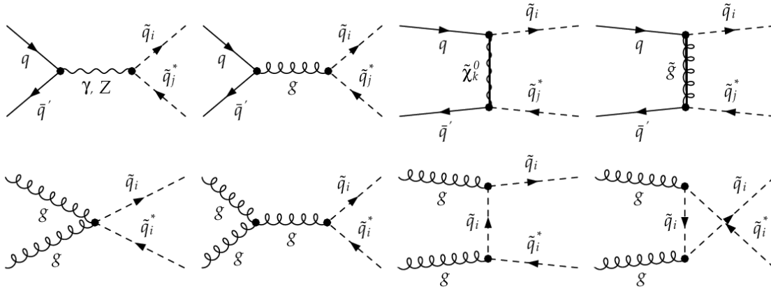
Figure 5.2: Tree-level Feynman diagrams for the production of neutral squark-antisquark pairs.
