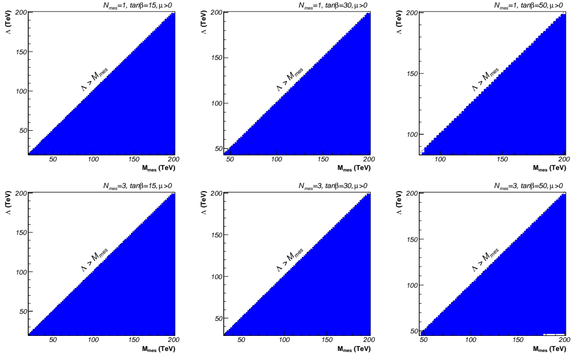
Figure 2.9: The \Lambda - M_{\text{mes}} planes for \tan\beta = 15, 30 , and 50 , N_{\text{mes}} = 1 and 3 , \mu > 0 . We show the b \rightarrow s\gamma excluded (dark blue) regions in constrained minimal flavour violation (cMFV). The region \Lambda > M_{\text{mes}} above the diagonal is theoretically excluded due to non-physical solutions to the renormalization group equations.
