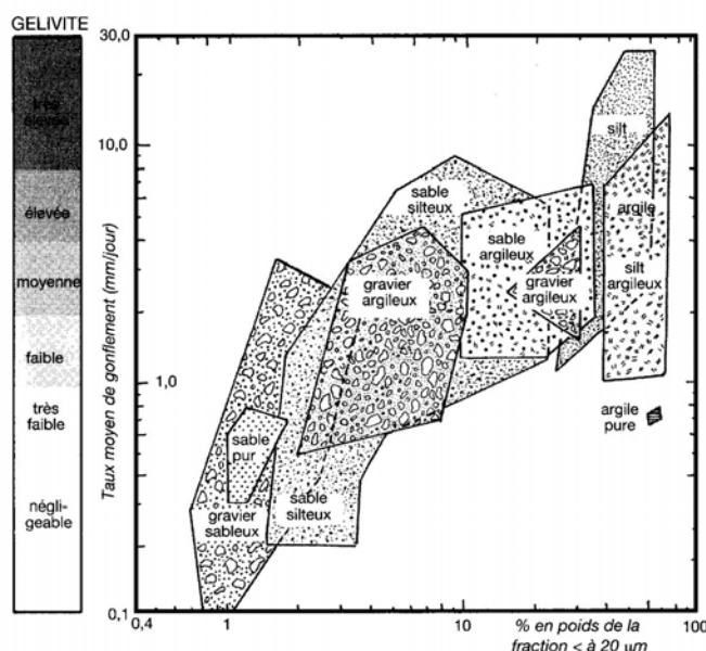
Mean frost-heave variations with granulometry of soil.
