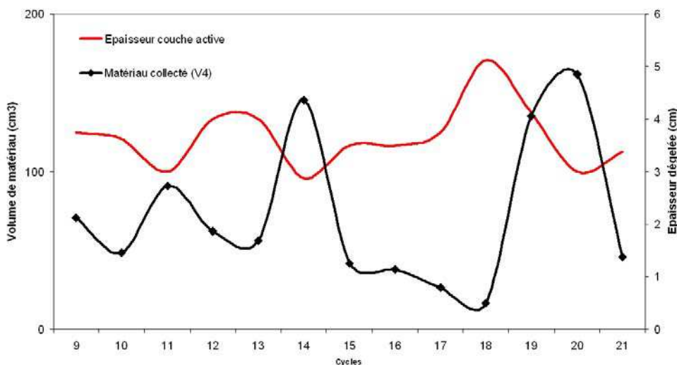
versant. Active layer thickness vs downslope deposit volume (V4).
