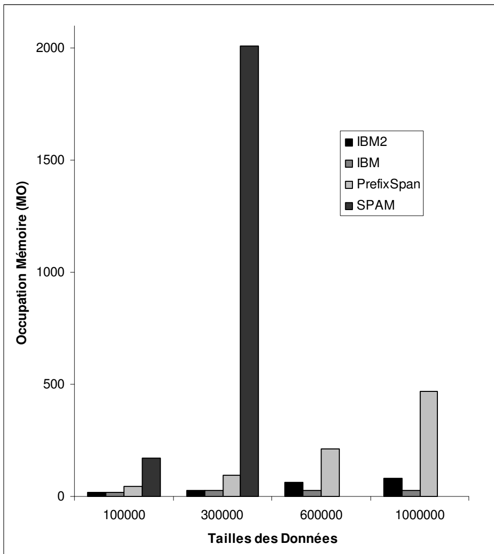
Figure 34: Consommations mémoire
