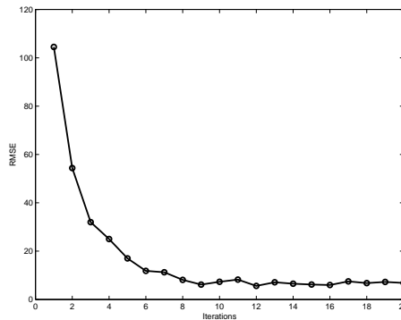
Figure 8.7: RMS error for the first twenty iterations. It can be noticed how the RMS values decrease drastically within the first iterations.
