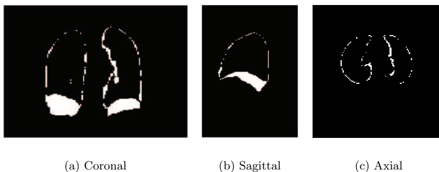
Figure 6.21: Absolute image difference between lungs image segmentation at \bar{x} + 3\sqrt{\lambda_1} and \bar{x} - 3\sqrt{\lambda_1} .
