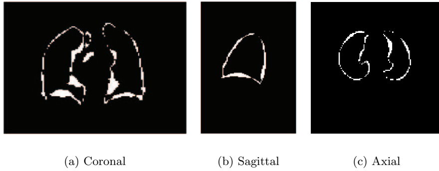
Figure 6.28: Absolute image difference between lungs image segmentation at \bar{x} + 3\sqrt{\lambda_4} and \bar{x} - 3\sqrt{\lambda_4} .
