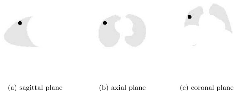
Figure 8.6: Sagittal, axial and coronal activity image planes of the reference state. The lesion is modelled as a sphere with a 15 mm diameter.
