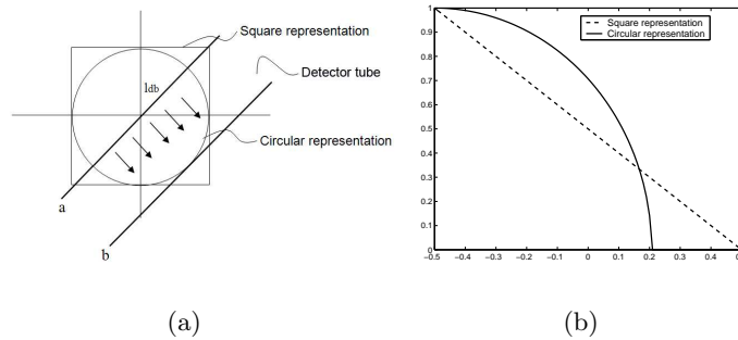
Figure 6.4: Modelling emission elements. The circular representation is illustrated and compared with the square one (2-D case) (a). Fig. 6.4(b) is a plot of intersection lengths (equivalent to the detection probability) when a detector tube (represented as a line) moves from point a towards point b , where a minimum is reached for the circular representation.
