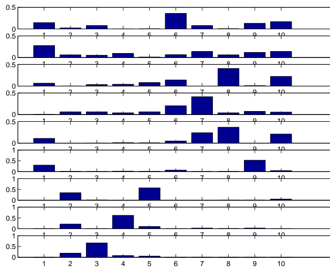
Figure 6.15: Contribution of each subject (columns) to each mode (rows) with subjects one and three rejected. Mode order is increasing starting with first one at the upper row.
