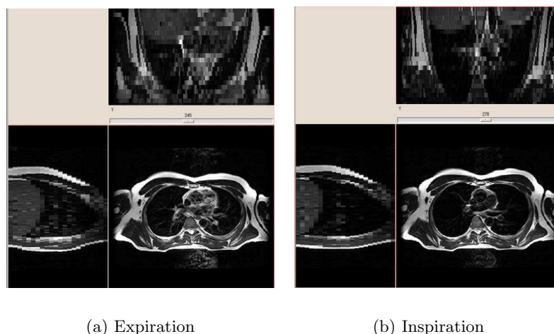
Figure 6.5: Two MRI images from a volunteer (taken at inspiration and expiration) were non-rigidly registered to create a real and known respiratory motion deformation.
