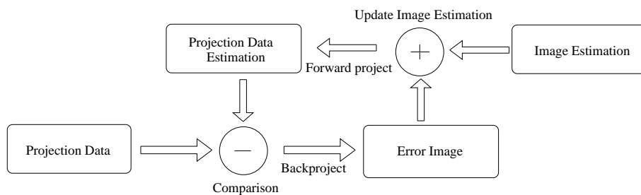
Figure 4.5: The basic idea behind algebraical reconstruction algorithms. Iteratively, a new image estimate is computed and its forward projection is compared with the acquired projection data. The residual error is backprojected into the image space to update the image estimation.
