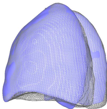
Figure 6.23: Superimposition of isosurfaces representing \bar{x} + 3\sqrt{\lambda_2} (wireframe) and \bar{x} - 3\sqrt{\lambda_2} (blue surface) for the second mode of variation. Notice the deformation at the base of the lungs.
