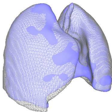
Figure 6.27: Superimposition of isosurfaces representing \bar{x} - 3\sqrt{\lambda_4} (wireframe) and \bar{x} + 3\sqrt{\lambda_4} (blue surface) for the fourth mode of variation. Notice the regular distance between surfaces compared with previous one.
