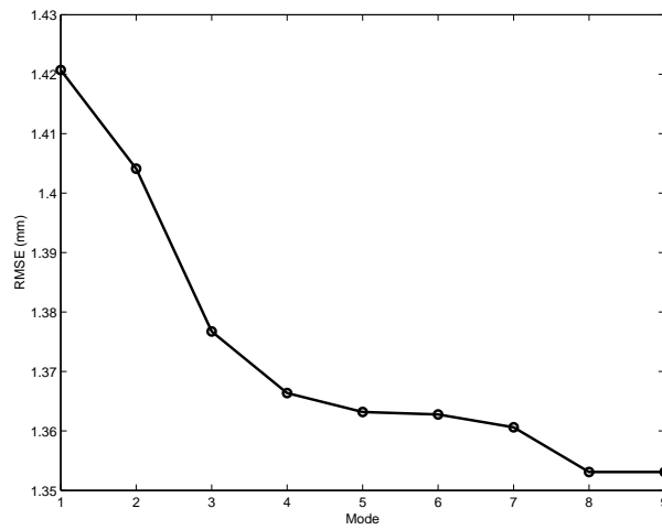
Figure 6.29: Leave-one-out study performed with the data set of ten observations. The mean error over the set of observations is plotted against the number of modes used to reconstruct the subject "left out".
