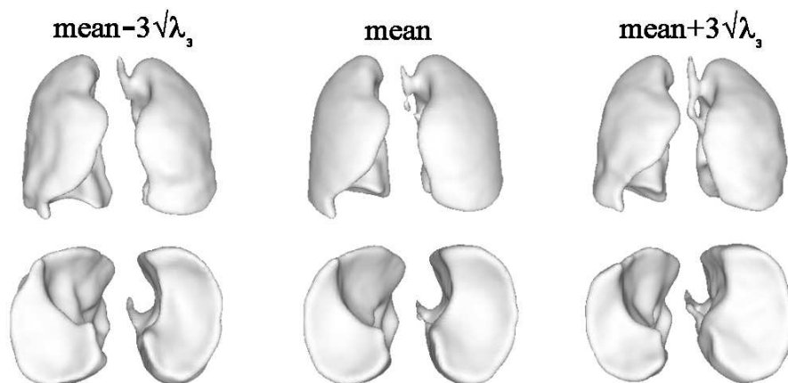
Figure 6.25: Third mode of variation. The modal amplitude for the third mode is varying in the range -3\sqrt{\lambda_3} \leq b_3 \leq +3\sqrt{\lambda_3} .
