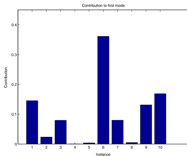
Figure 6.16: Contribution of each subject to the first mode after subjects one and three have been rejected. A much better balanced contribution is seen.
