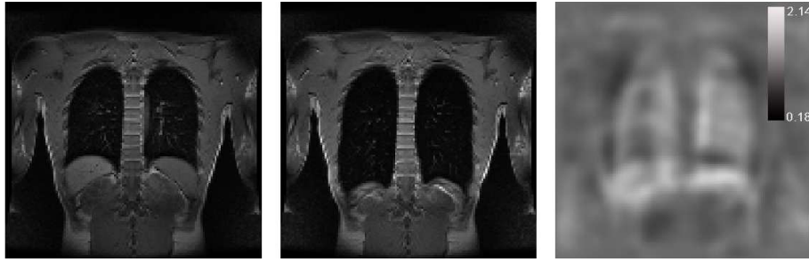
Figure 6.2: Jacobian map of a DVF obtained after non-rigid registration of two MRI images of the same volunteer taken at expiration (left) and inspiration (center). Expansion in the lungs are clearly visible with values of |\nabla\varphi| > 1 .
