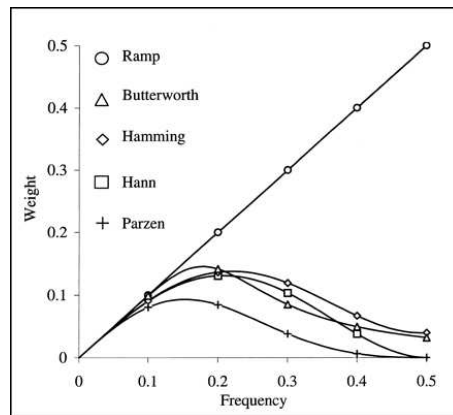
Figure 4.3: Different filters used in FBP. Ramp filter alone increases high frequencies. Low pass filters associated with the ramp filter limit the noise component.
