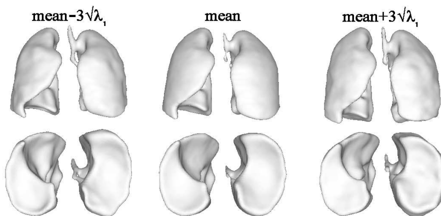
Figure 6.19: First mode of variation. The modal amplitude for the first mode is varying in the range -3\sqrt{\lambda_1} \leq b_1 \leq +3\sqrt{\lambda_1} .
