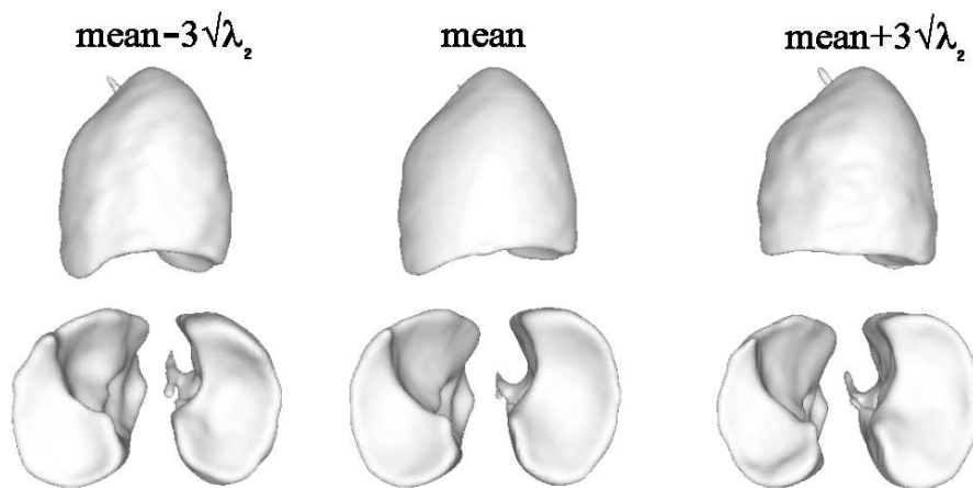
Figure 6.22: Second mode of variation. The modal amplitude for the second mode is varying in the range -3\sqrt{\lambda_2} \leq b_2 \leq +3\sqrt{\lambda_2} .
