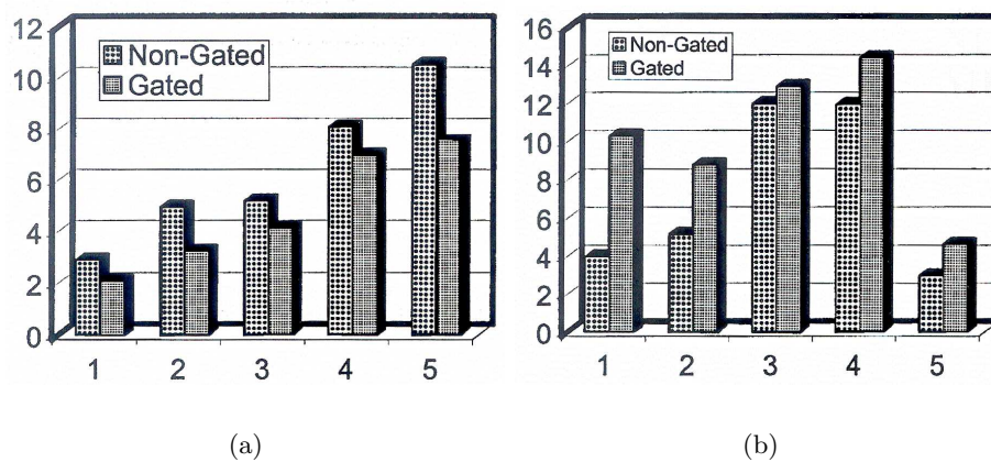
Figure 5.8: Volume changes between gated and non-gated images in five patients (a). A noticeable volume reduction is observed when gating is used. Quantitative results indicate that larger SUV values are found in gated reconstructed images in comparison with its non-gated counterpart (b), which indicates larger concentrations over the true lesion volume. Image source: [83]
