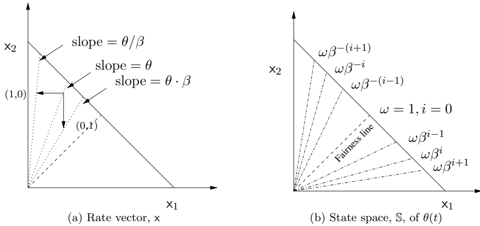
Figure 4.4: Geometric interpretation.
