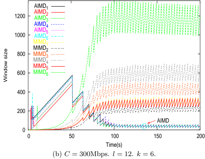
Figure 4.7: Window evolution of sessions.
