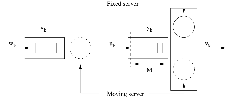
Figure 6.2: The discrete-time tandem queue model.
