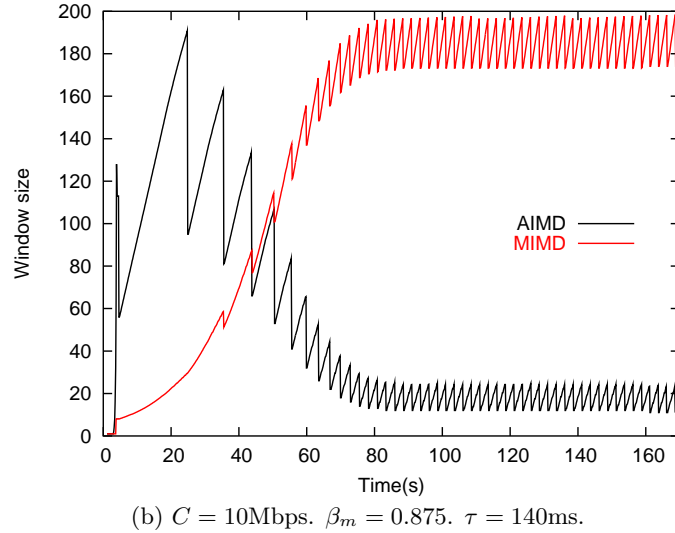
Figure 4.8: Window evolution for one MIMD session and one AIMD session.
