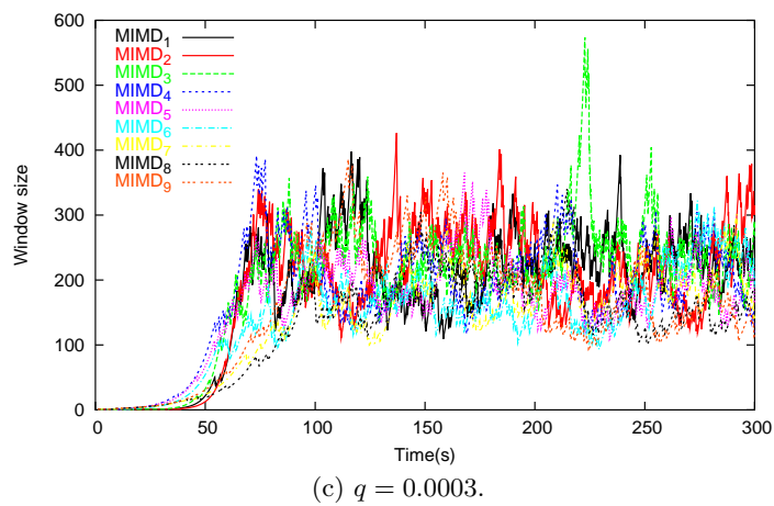
Figure 4.6: Window evolution of MIMD sessions. RTT_1 = 50ms . RTT_2 = 90ms . RTT_3 = 140ms .
