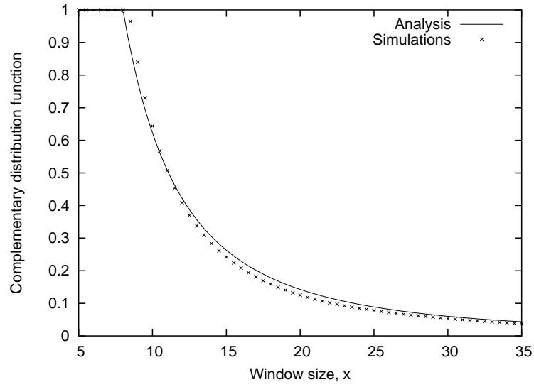
Figure 3.7: Time-average complementary distribution function of the window size, X . \frac{s^*}{\alpha} = 2.12 .
