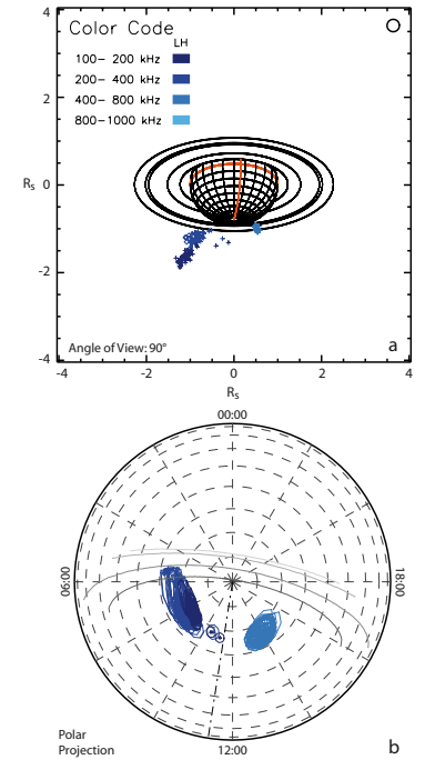
Figure 11. Simulation of errors on real data. The data shown on this figure is selected as follows: day 2006-268, 18:40 to 18:45 SCET, \text{SNR} > 20 \text{ dB} and 0.8 > V > 1.1 . Panel a shows the directions of arrival of the waves, as viewed from Cassini, and panel b, the corresponding footprints of the active magnetic field lines on a polar projection. The crosses + and diamonds \diamond are representing data points intersecting or not \mathcal{F}_{oc} (respectively). For directions of arrival intersecting \mathcal{F}_{oc} , the projected simulated errors are shown in thin line. These projected errors have been computed with a 2^\circ -error on the observed direction of arrival. This figure has been built from one frame of Fig. S1.
