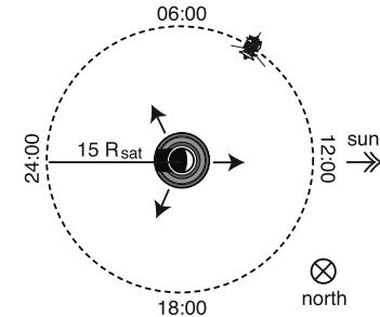
464 Figure A1. Schematic geometrical configuration for a 465 spacecraft on a circular orbit at 15 R_S in the equatorial plane, 466 observing southern radio sources defined by \lambda_B = -70^\circ and 467 LT = 0400, 1200, and 2000 (black arrows). Results of simulations of both loss-cone- and shell-driven emissions are displayed in Figures A2 and A3.
