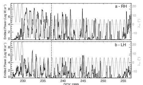
Figure 3. Time series of RH and LH radiated powers, smoothed over 3 hours. The magnetic latitude of Cassini is superimposed (grey line, identical in both panels). The dashed line at day 237 marks the transition from anticorrelated to correlated variations of RH and LH emissions.
