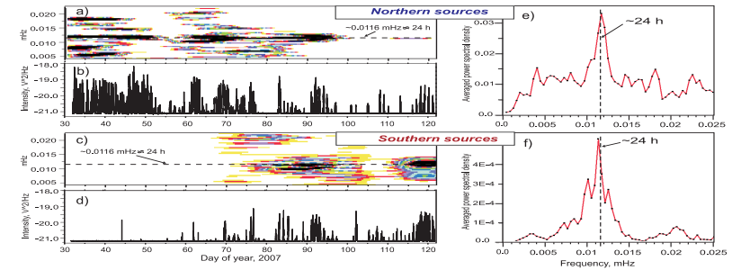
Figure 2. SWF dynamical spectra of modulations (panels a, c) and intensity profiles (panels b, d) of AKR emitted by Northern and Southern sources. Black color in the modulation spectra means the highest and yellow denotes the lowest values of the spectral density. The panels (e) and (f) show the time averaged profiles of the SWF dynamical spectra.
