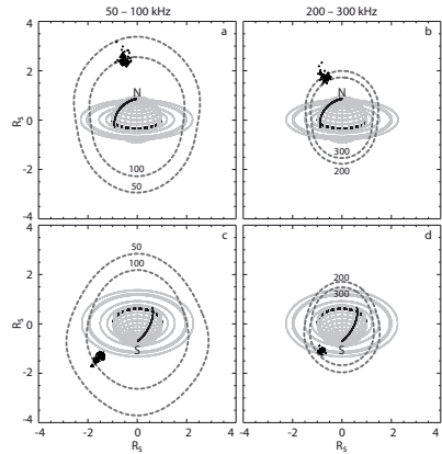
Figure 4. 2D maps projected on the y - z plane (see Fig. 2). The upper and lower row are respectively showing data acquired in the northern (time interval: 2006/269, 02:00 to 02:15 SCET; distance to Saturn: 5.7 R_S ; Latitude of the spacecraft: +21.0^\circ ; local time: 16:15 LT) and southern (time interval: 2006/268, 16:30 to 16:45 SCET; distance to Saturn: 4.5 R_S ; Latitude of the spacecraft: -36.5^\circ ; local time: 09:25 LT) hemispheres. Left and right columns are respectively showing data with 50-100kHz and 200-300kHz frequency selection. The data is also selected with a minimum SNR of 20dB and a circular polarization degree |V| > 0.8 . The gray dashed lines are the contour of \mathcal{F}_{ce}(f) as seen from Cassini for the labeled frequency (also called “radio horizon”), as seen for the Cassini spacecraft. The noon meridian and the equator are drawn in black on Saturn.
