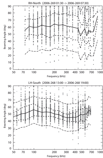
Figure 7. Beaming Angle with respect to frequency for Northern (top panel) and Southern (bottom panel) sources. The data was selected with respect to circular polarization degree only: V > 0.9 for the southern hemisphere data and V < -0.9 for the northern hemisphere data. The crosses (+) and diamonds ( \diamond ) represent the data points whose associated direction of arrival is intersecting or not \mathcal{F}_{ce} , respectively. Each panel is displaying six hours of data, as mentioned in their respective title. The average (plain line) has been computed for each frequency, using only the directions of arrival intersecting \mathcal{F}_{ce} . The corresponding standard deviation of the distribution is displayed in dashed line ( \pm 1 standard deviation levels). The mixed lines are showing the maximum simulated error adding a 2^\circ -error on each direction of arrival.
