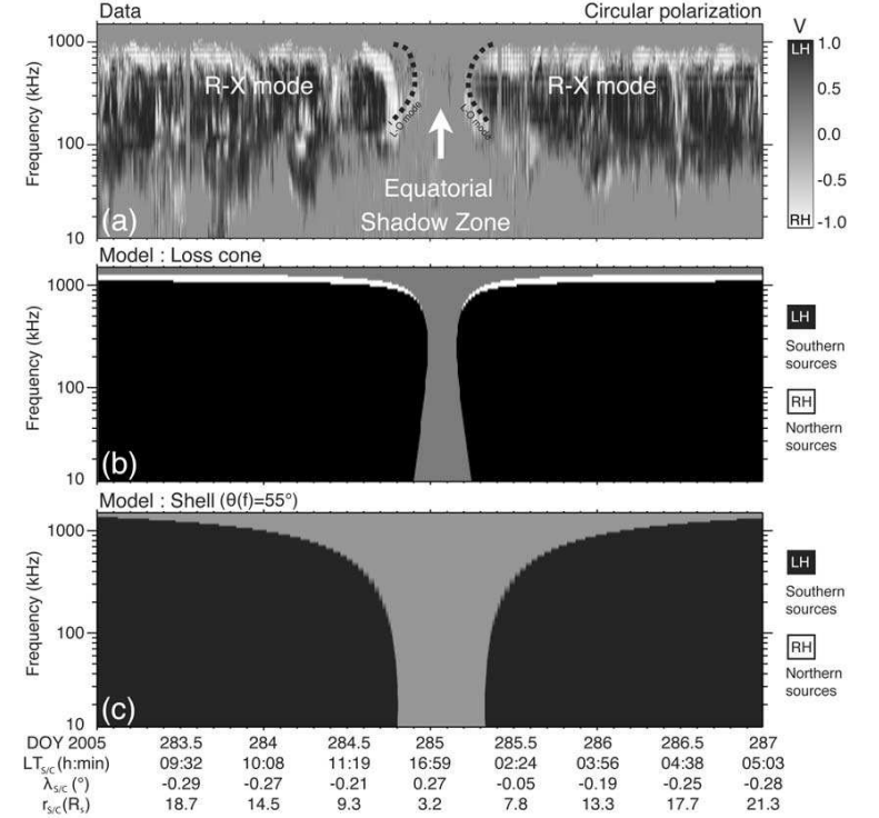
Figure 3. (a) Observed dynamic spectrum of SKR circular polarization degree during a crossing of the ESZ (adapted from Figure 6a of Lamy et al. [2008]). (b) Simulated dynamic spectrum under the assumption of a loss-cone-driven CMI generation of southern (black) and northern (white) sources distributed at all LT around the planet (with a 30 s temporal resolution) on magnetic field lines defined by \lambda_B = -70^\circ . Regions of the (t, f) plane which are simultaneously illuminated by the RH and LH components are plotted in black in order to take the predominance of the LH emission into account. (c) Same as Figure 3b for shell-driven simulations using \theta(f) = 55^\circ . In this case, the RH component is systematically masked by the LH one.
