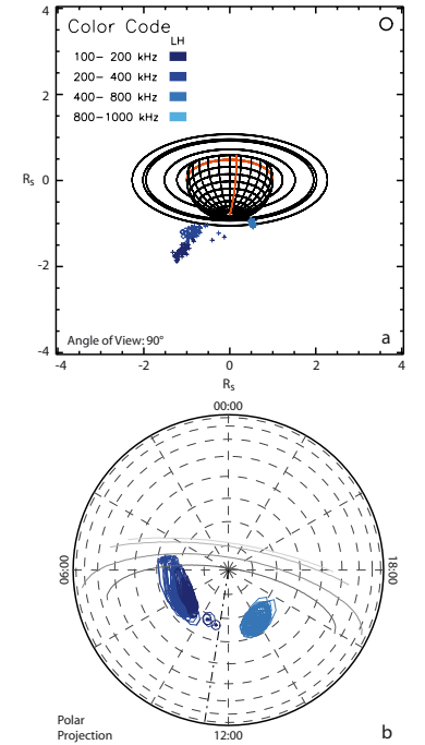
Figure 11. Simulation of errors on real data. The data shown on this figure is selected as follows: day 2006-268, 18:40 to 18:45 SCET, \text{SNR} > 20 \text{ dB} and 0.8 > V > 1.1 . Panel a shows the directions of arrival of the waves, as viewed from Cassini, and panel b, the corresponding footprints of the active magnetic field lines on a polar projection. The crosses + and diamonds \diamond are representing data points intersecting or not \mathcal{F}_{oc} (respectively). For directions of arrival intersecting \mathcal{F}_{oc} , the projected simulated errors are shown in thin line. These projected errors have been computed with a 2^\circ -error on the observed direction of arrival. This figure has been built from one frame of Fig. S1.
