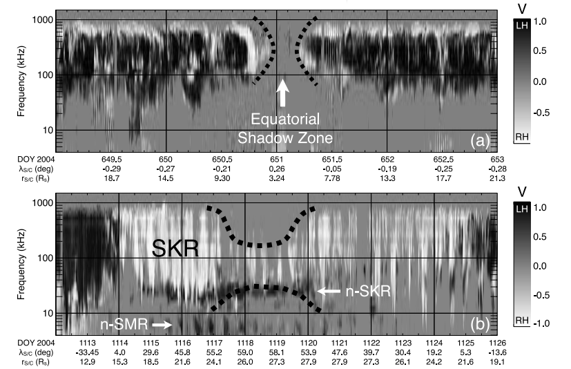
Figure 6. Dynamic spectra of the SKR circular polarization degree, quantified by the grey scale bar on the right-hand side of the plots. The spectra are shown for time intervals corresponding to an equatorial and a polar disappearance of the radio emission. (a) During the near-equatorial passage on DOY 649–653, containing the observation of a perikrone with closest approach at 3.01 R_s (DOY 651), SKR disappears during several hours at the crossing of the equatorial shadow zone, whose extent versus frequency is emphasized by the dashed thick lines. The equatorial extent of the shadow zone is minimum at 200 kHz, where it is about 4 R_s . It increases up to \sim 6 – 7 R_s , at 80 and 900 kHz. (b) During the northern pass on DOY 1113–1126, with \lambda_{sc} reaching 59.2^\circ on DOY 1118, the upper (and to a lesser extent the lower) frequency ends of the SKR range disappear for \lambda_{sc} > 55^\circ , as again emphasized by the dashed thick lines. The figure also shows the occurrence of n-SMR and n-SKR at low frequencies for high latitudes.
