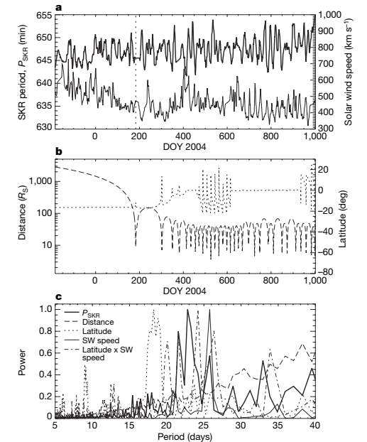
Figure 2 'Short-term' variations in P_{\text{SKR}} compared with solar wind speed at Saturn and variations in orbital parameters of Cassini. The same 3.25-year interval as in Fig. 1 is shown. a , Variations in P_{\text{SKR}} (heavy line; left scale) obtained as explained in the text and in Supplementary Figs 1–3. The solar wind speed plotted below (light line; right scale), measured by the ACE and WIND spacecraft near the Earth's orbit ( http://omniweb.gsfc.nasa.gov/ ) and projected to Saturn, shows similar fluctuations on a timescale of 20–30 days. Solar wind projection includes ballistic radial projection from ~1 to 10 AU, plus a delay compensating for the longitude difference between Earth and Saturn. The dotted vertical line indicates Cassini's Saturn orbit insertion. b , Cassini orbital parameters: distance to Saturn (dashed; left scale; 1 R_S = 1 Saturn radius = 60,300 km) and latitude (dotted; right scale). c , Fourier power spectrum of the fluctuations of all the above quantities, plus the quantity (latitude × solar wind speed) which provides a simple way of simulating beating between latitudes (and thus visibility of the radio emission) and variations in the solar wind speed.
