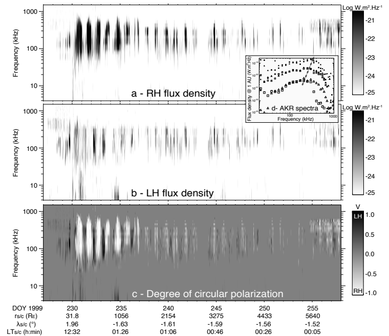
Figure 1. Dynamic spectra of (a) RH and (b) LH AKR flux densities normalized to 1 AU over the entire Earth's fly-by. (c) Circular polarization degree, from purely RH (white) to purely LH (black). Cassini ephemeris are indicated in abscissa. r_{sc} , \lambda_{sc} and LT_{sc} respectively indicate the distance to Earth, the geographic latitude and the local time of the spacecraft. (d) Flux densities normalized to 1 AU reached by AKR 50, 10 and 1% of the time, as a function of frequency (big, medium and small symbols, respectively). Triangles refer to RH emission and squares to LH emission. RPWS detection threshold was here \sim 10^{-23} W.m^{-2}.Hz^{-1} . The grey arrow emphasizes the shift of the AKR spectral peak toward higher frequencies with increasing intensity.
