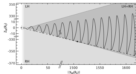
Figure 4. Sketch of Cassini trajectory in magnetic coordinates in a meridian plane. The envelope of its southernmost excursion is represented by the dashed line. The Earth lies at (0,0). The equatorial AKR shadow zone is filled in white, regions illuminated by either RH or LH sources in light-grey, and the region illuminated by both sources in darker grey. The transition described in the text is represented by the black dot. Note that the precise location of the dotted-line boundaries are frequency dependent.
