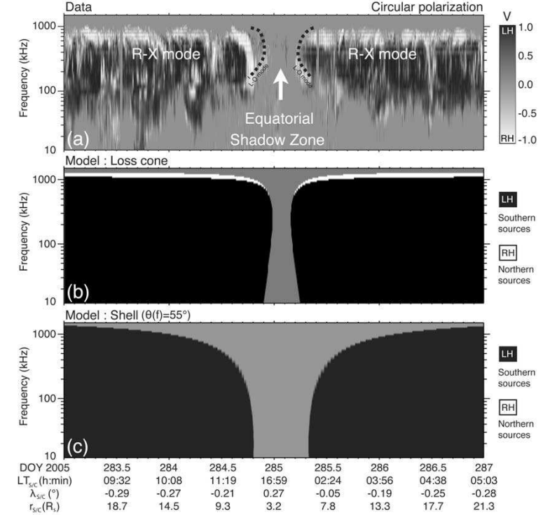
Figure 3. (a) Observed dynamic spectrum of SKR circular polarization degree during a crossing of the ESZ (adapted from Figure 6a of Lamy et al. [2008]). (b) Simulated dynamic spectrum under the assumption of a loss-cone-driven CMI generation of southern (black) and northern (white) sources distributed at all LT around the planet (with a 30 s temporal resolution) on magnetic field lines defined by \lambda_B = -70^\circ . Regions of the (t, f) plane which are simultaneously illuminated by the RH and LH components are plotted in black in order to take the predominance of the LH emission into account. (c) Same as Figure 3b for shell-driven simulations using \theta(f) = 55^\circ . In this case, the RH component is systematically masked by the LH one.
