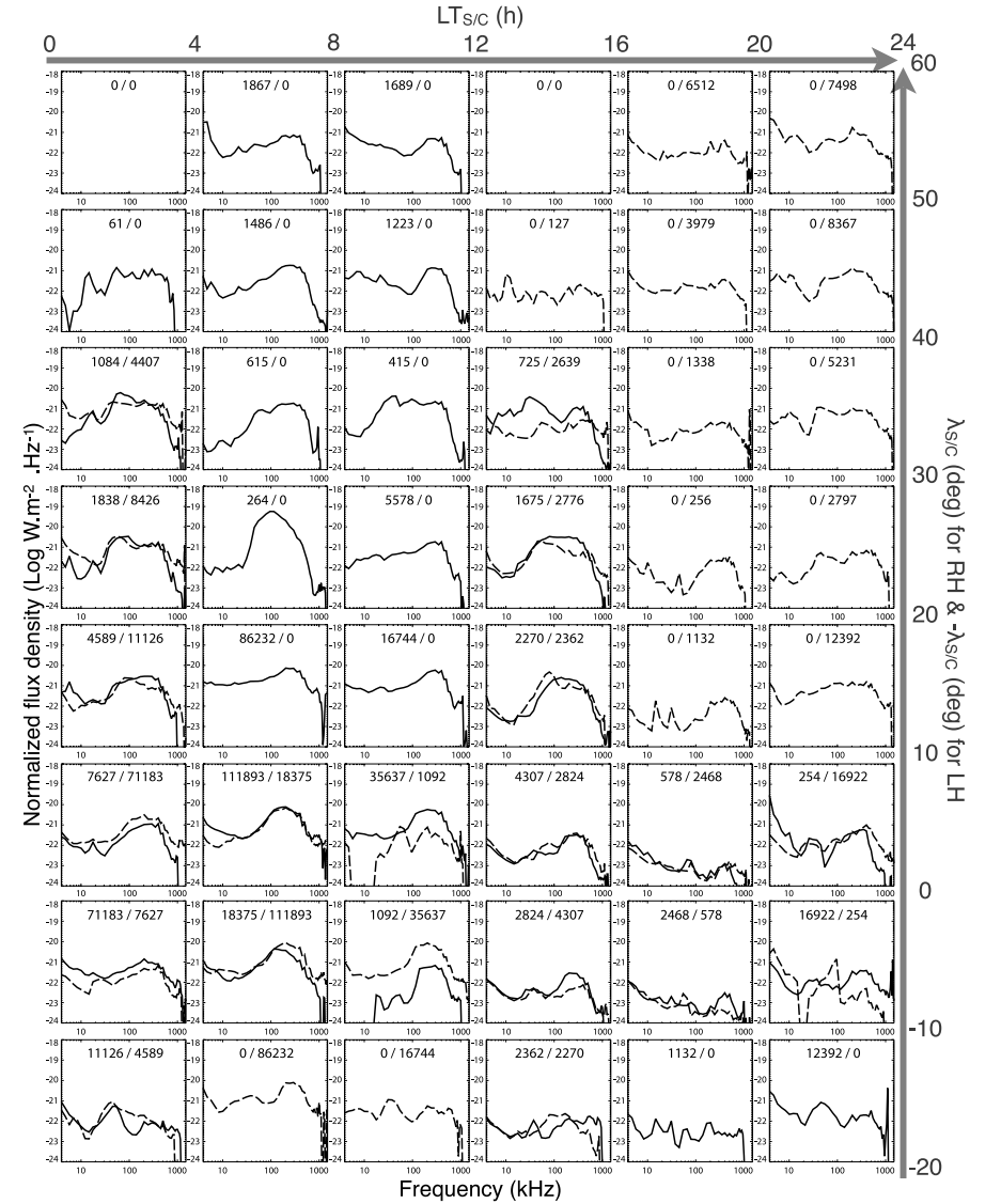
Figure 10. Median flux density spectra over our 2.75 years data set sorted by local time and latitude of the observer. The 50% occurrence spectra of LH (solid) and RH (dashed) SKR are plotted within intervals of 4 h of LT_{sc} by 10^\circ of \lambda_{sc} . RH spectra for a given interval of \lambda_{sc} are superimposed to LH spectra for the same interval of -\lambda_{sc} . The two numbers at the top of each panel are the number of individual (3 min) LH and RH SKR spectra involved in the computation of the median.
