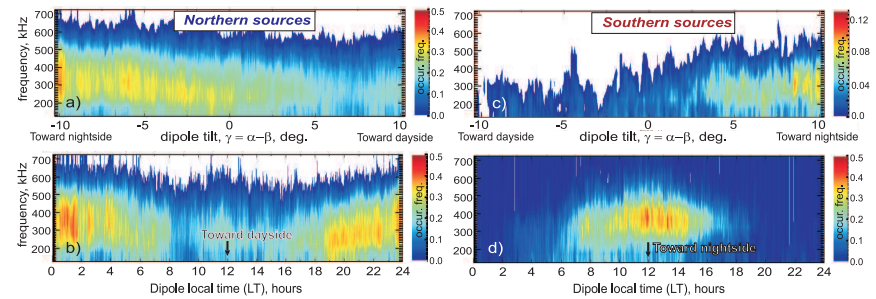
Figure 4. Normalized occurrence frequency and frequency range of the AKR emitted from the Northern and Southern hemispheres as functions of the inclination angle \gamma = \alpha - \beta (top panels) and local time of the axis of the magnetic dipole (bottom panels). Color indicates fraction of AKR occurrence frequency relative to all observations.
