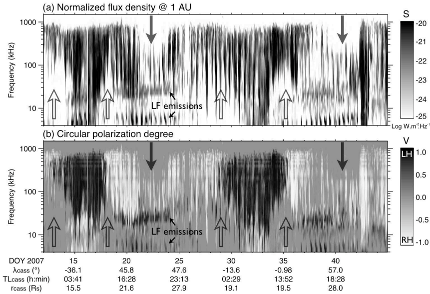
Figure A4: Dynamic spectra of (a) flux density S (in \text{W}/\text{m}^2 \cdot \text{Hz} ) normalized to 1 AU and (b) normalized degree of circular polarization V , with corresponding color bar on the right-hand side of each panel. The displayed interval (from DOY 13 to 45) includes that of the 2007 HST campaign (from DOY 13 to 42). The dynamic spectra not only shows the intense broadband SKR but also non-auroral low frequency emission below 40 kHz. Moreover, as a consequence of the SKR anisotropy combined with the changing location of the spacecraft, two typical visibility effects appear in dynamic spectra. When Cassini crosses the equatorial plane, the frequency extent of the SKR spectrum reduces (empty arrows) whereas when Cassini passes at high northern latitudes ( > 55^\circ ) the SKR highest and lowest frequencies disappear (full arrows). Both visibility effects directly affect the measured SKR power.
