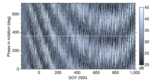
Figure 1 Evidence of short-term variations in P_{\text{SKR}} and their relation to long-term variations. The SKR power-time series (derived as explained in Supplementary Figs 1 and 2) is displayed here over the 3.25-year interval studied, in a format similar to that of Fig. 1 in ref. 17. Variations in SKR power during consecutive rotations are plotted as consecutive vertical lines with a power scale in grey levels, using an assumed fixed period of 10 h 48 min. Time is in day of the year (DOY) 2004. Data gaps are displayed in flat grey (major ones are before DOY = 137 and at about DOY 191 ± 4 and 377 ± 5). Each rotation is plotted twice for clarity, separated by the white horizontal line. The origin of phases—and thus the absolute phase—is arbitrary. Previous authors 17 noted that the fact that the SKR peak wanders with variable slope over the time interval means that a fixed period does not organize the SKR modulation well. We see here the same long-term behaviour. In addition, the quality of our data processing (see the legend to Supplementary Fig. 1a) reveals quasi-periodic oscillations of the SKR period on a timescale of 20–30 days. Those are especially clear after DOY 400, where the long-term drift is small and fewer data gaps are present. The amplitude of these fluctuations is large (~2% peak to peak), and their long-term averaging results in the slow, smaller-amplitude (<1% peak to peak over the studied interval) variation of P_{\text{SKR}} noted by previous authors.
