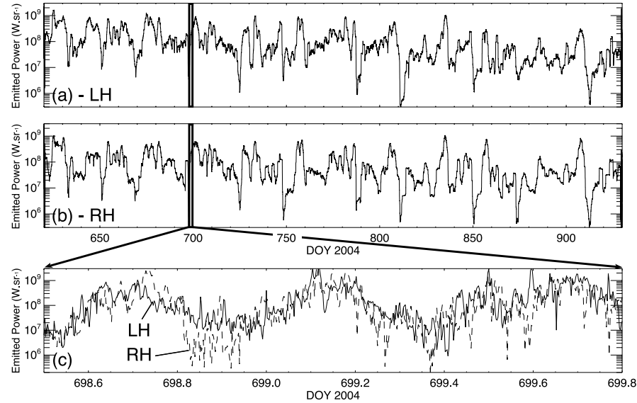
Figure 9. Total power radiated by each polarization component between 100 and 400 kHz (expressed in W \cdot sr^{-1} ). Figures 9a and 9b display LH and RH powers smoothed over 1 day between DOY 620 and 930. This interval corresponds to near-equatorial orbits ( |\lambda_{sc}| < 1^\circ ) when observing conditions of LH and RH polarizations were similar. Figure 9c shows a zoom around DOY 699 where LH (solid) and RH (dashed) powers are superimposed, at the full time resolution of 3 min.
