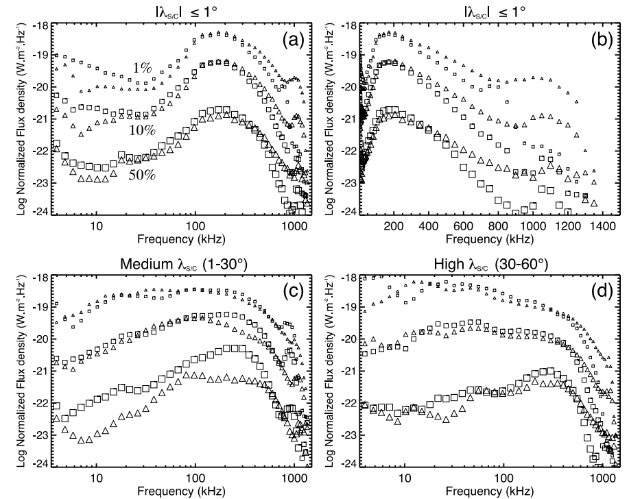
Figure 8. Occurrence levels of LH (squares) and RH (triangles) SKR as a function of frequency over our 2.75 years data set. The flux density levels, normalized to 1 AU, reached 50%, 10%, and 1% of the time are represented respectively as large, medium and small symbols. The median spectra (50% occurrence levels) are a very good proxy for average SKR spectra. Figures 8a and 8b focus on near-equatorial observations ( |\lambda_{sc}| \leq 1^\circ ), Figure 8c on intermediate latitude observations ( -30^\circ \leq \lambda_{sc} < -1^\circ for LH and 1^\circ < \lambda_{sc} \leq 30^\circ for RH), and Figure 8d on high latitude observations ( -60^\circ \leq \lambda_{sc} < -30^\circ for LH and 30^\circ < \lambda_{sc} \leq 60^\circ for RH). The frequency scale is logarithmic in Figures 8a, 8c, and 8d, and linear in Figure 8b.
