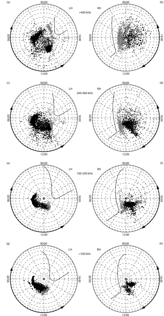
Figure 6. SKR sources magnetic footprint (see Fig. 5). The left (a,c,e,g) and right (b,d,f,h) panels are respectively showing southern-LH and northern-RH observations. Each row of panel show the data for different frequency selection: >400 kHz (a,b), 200-400 kHz (c,d), 100-200 kHz (e,f) and <100 kHz (g,h). The black crosses (+) and the grey diamonds (o) are the footprints of the active magnetic field lines, whether the direction of arrival is respectively intersecting \mathcal{F}_{ce} or not. The magnetic field footprints are obtained as presented in App. B. The plain line gives the merged radio horizon for the whole studied period: before 22:20 SCET (equator crossing) for southern data and after 22:20 SCET for northern data. The radio horizons for the beginning and the end of these periods are shown in dashed grey. The thick arrowed lines show the LT sector in which Cassini is for the displayed data.
