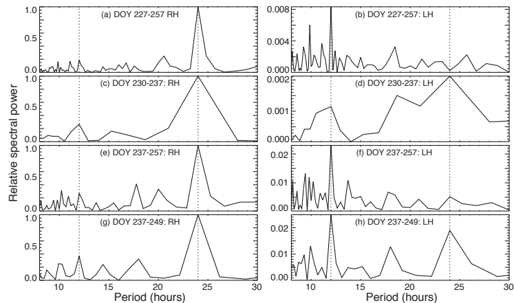
Figure 2. Fourier power spectra of RH and LH emission variations: (a,b) over the entire fly-by; (c,d) along the outbound leg prior to day 237; (e,f) after day 237; (g,h) interval of strong AKR activity). Dashed lines indicate 12h and 24h periods. Pairs of spectra on each row are normalized to the strongest peak in RH spectrum. Horizontal scale is nonlinear (in 1/f ), which causes 24h peaks to be intrinsically broader than 12h ones.
