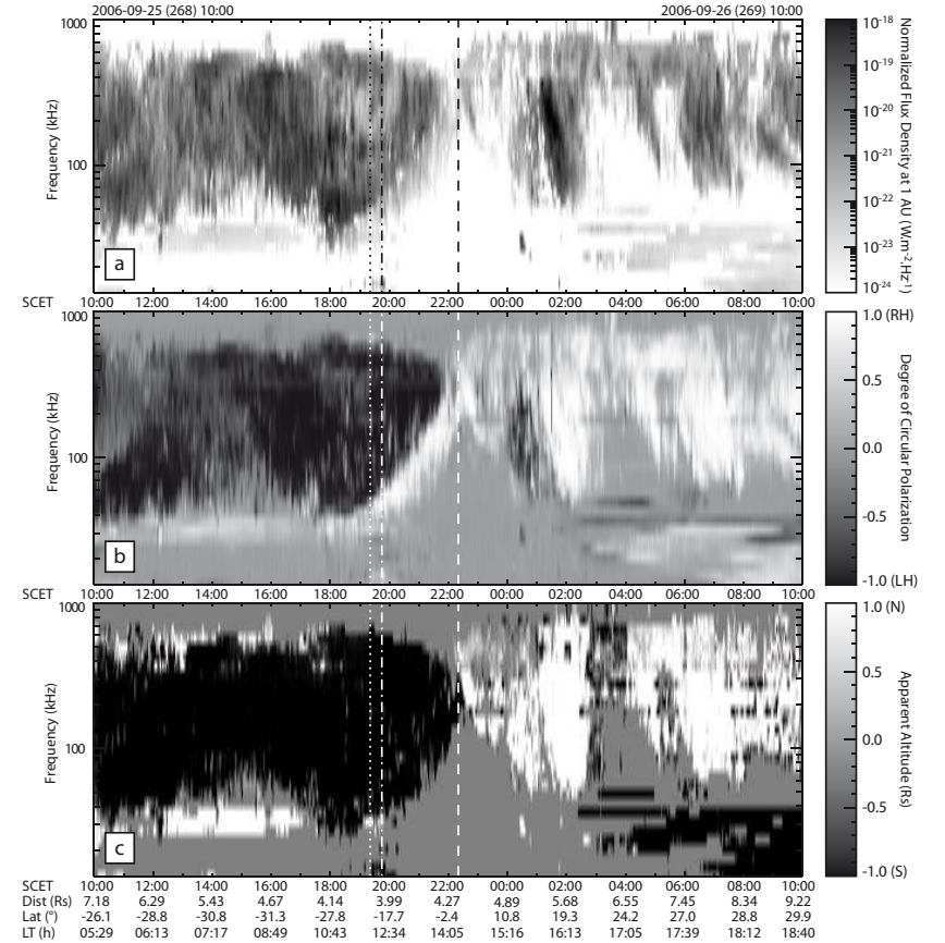
Figure 3. Dynamic spectrum of the SKR flux density (a) in \text{Wm}^{-2}\text{Hz}^{-1} , degree of circular polarization (b) and apparent hemisphere of emission (c) provided by the GP analysis. The orbital parameters are recalled below the bottom panel. See caption of Fig. 1 for the vertical lines. On panel (c), the apparent altitude z as defined in Fig. 2 is saturated outside of the [-1, +1] interval in order to display the hemisphere of emission rather than the projected altitude. For panels a and c, the data was selected with the following condition on the circular polarization degree: |V| > 0.2 .
