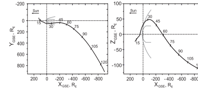
Figure 1. STEREO-Behind orbit in GSE coordinates (solid bold line). Black ticks indicate the day of year, 2007.
