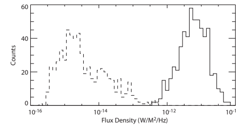
Figure 8. Flux Density distributions for R-X mode (plain line) and L-O mode (dashed line). The time interval selected for the R-X mode data is: 16h19m12s to 17h16m48s SCET; for L-O mode data: 21h07m12s to 22h04m48s SCET. For both R-X and L-O mode, the frequency selection is 100 to 300 kHz.
