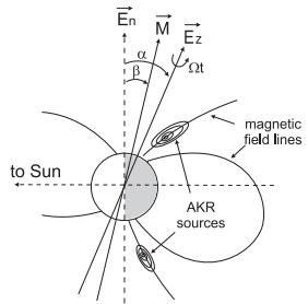
Figure 3. Schematic view of the AKR source region. \vec{E}_n is normal to the ecliptic plane and \vec{M} is the axis of the terrestrial magnetic dipole, tilted by \approx 10.3^\circ from the Earth’s rotation axis \vec{E}_z . Angle \alpha denotes the inclination of the Earth’s rotation \vec{E}_z axis from the normal to ecliptic \vec{E}_n . In half a year, \alpha changes slowly from \approx -23.4 in summer to \approx +23.4 in winter. The angle \beta describes tilt of the axis of the magnetic dipole \vec{M} relative to the ecliptic normal \vec{E}_n .
