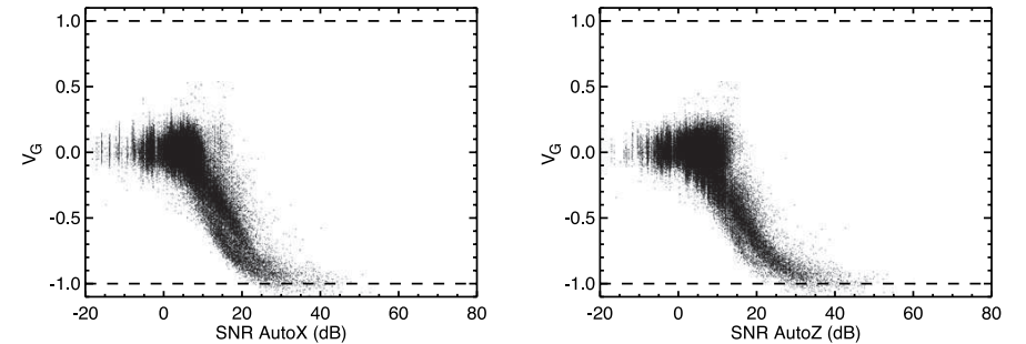
Figure A2. Normalized degree of circular polarization V_G provided by Goniometric inversion for DOY 1100 (predominant RH SKR, i.e., V_G close to -1 ) as a function of SNR of autocorrelation measured on each antenna (dipole X and monopole Z). Only data points corresponding to frequencies above 100 kHz are considered to avoid low-frequency n-SKR emissions. A selection is also applied on the geometric configuration between sources and the antennas plane ( \beta \geq 20^\circ following Cecconi and Zarka [2005]). Both images show that highest SNR match highest V_G .
