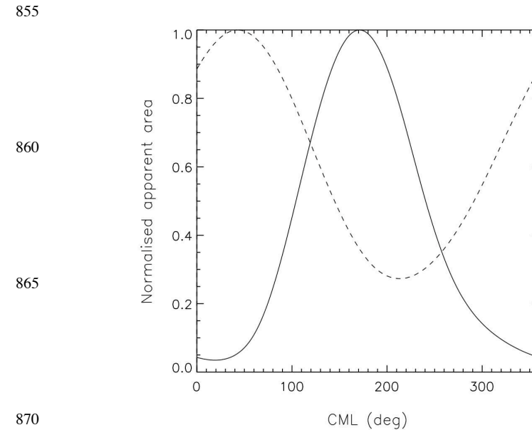
Figure A1: Geometric correction factors for the north (solid) and south (dashed) polar regions applied to Jupiter's auroral brightness data. CML is system III central meridian longitude.
