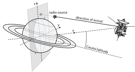
Figure 2. The goniopolarimetric inversions are providing the direction of arrival of a free-space propagating electromagnetic wave. It does not provide the actual source position. It is possible to map the source position as projection of the obtained direction of arrival on a plane (here taken as the plane perpendicular to the Cassini–Saturn line passing through the center of Saturn).
