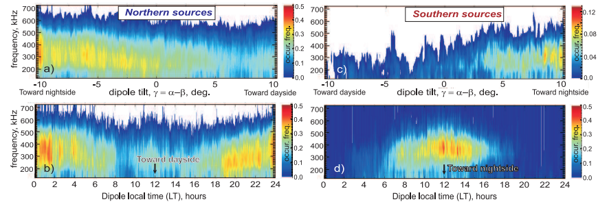
Figure 4. Normalized occurrence frequency and frequency range of the AKR emitted from the Northern and Southern hemispheres as functions of the inclination angle \gamma = \alpha - \beta (top panels) and local time of the axis of the magnetic dipole (bottom panels). Color indicates fraction of AKR occurrence frequency relative to all observations.
