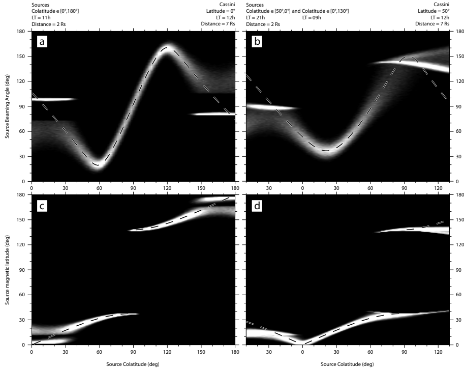
Figure 9. Error analysis on simulated data. The two columns are corresponding to two configurations described on top of them. The top and bottom rows show respectively the simulated beaming angle and the footprint colatitude of the magnetic field on which the source is, with respect to the input source colatitude. On each plot, the dashed line represent the input value of the simulated parameter. The spread of the simulated results are due to a 1^\circ error added on the input direction of arrival.
