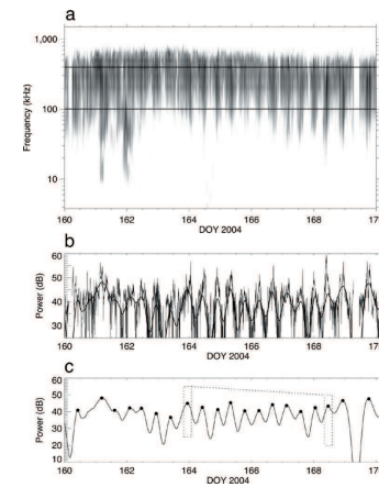
Figure S1: Example of Cassini RPWS data and processing allowing to estimate P_{SKR} accurately down to short timescales. a , Dynamic spectrum of SKR detected in left-hand (LH) polarization, i.e. originating from the southern hemisphere, for 10 days of year 2004 before SOI. Data processing includes selection of SKR emission based on measured circular polarization, followed by elimination of interference and interpolation of resulting data on a regular time-frequency grid, with 3 min time resolution and 48 frequencies between 3.8 and 1500 kHz. Only LH SKR, whose intensity dominates over the time-interval studied, is used in the present analysis. Data gaps of a few hours are present on DOY 160 and 169. b , Frequency-integration over the peak region of the SKR spectrum, between 100 and 400 kHz (horizontal black lines in the Top panel), provides a time series of the SKR power. Most of the SKR power is emitted within this spectral range, over which the SKR spectrum nearly always extends when SKR is present. c , Smoothing of the SKR time series using a 5-hour wide sliding window removes high-frequency fluctuations and enhances the main variation at P_{SKR} (smoothing is applied twice for better efficiency). The smoothed curve is reproduced in panel b for comparison with the original time series. Detection
