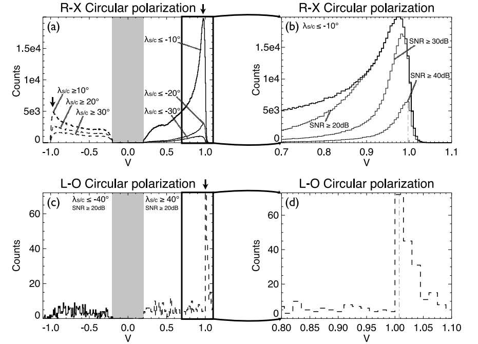
Figure 4. Histograms of SKR circular polarization degree V in the range [100,400 kHz] for high latitude excursions of the spacecraft. (a) LH polarization measured for emissions detected when \lambda_{sc} \leq -10 , -20 , or -30^\circ (solid lines), and RH polarization measured for emissions detected when \lambda_{sc} \geq 10 , 20 , or 30^\circ (dashed lines). (b) Zoom of the LH histogram corresponding to \lambda_{sc} \leq -10^\circ (boldface) and similar LH histograms where an SNR threshold is imposed at 20, 30, and 40 dB (lightface). The distribution corresponding to SNR \geq 40 dB peaks at 0.99 \pm 0.01 . (c) LH polarization measured for emissions detected when \lambda_{sc} \geq 40^\circ and SNR \geq 20 dB (dashed line), and RH polarization measured for emissions detected when \lambda_{sc} \leq -40^\circ and SNR \geq 20 dB (solid line). (d) Zoom of the LH histogram. A peak at 1.00 \pm 0.01 is observed.
