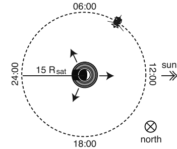
464 Figure A1. Schematic geometrical configuration for a 465 spacecraft on a circular orbit at 15 R_S in the equatorial plane, 466 observing southern radio sources defined by \lambda_B = -70^\circ and 467 LT = 0400, 1200, and 2000 (black arrows). Results of simulations of both loss-cone- and shell-driven emissions are displayed in Figures A2 and A3.
