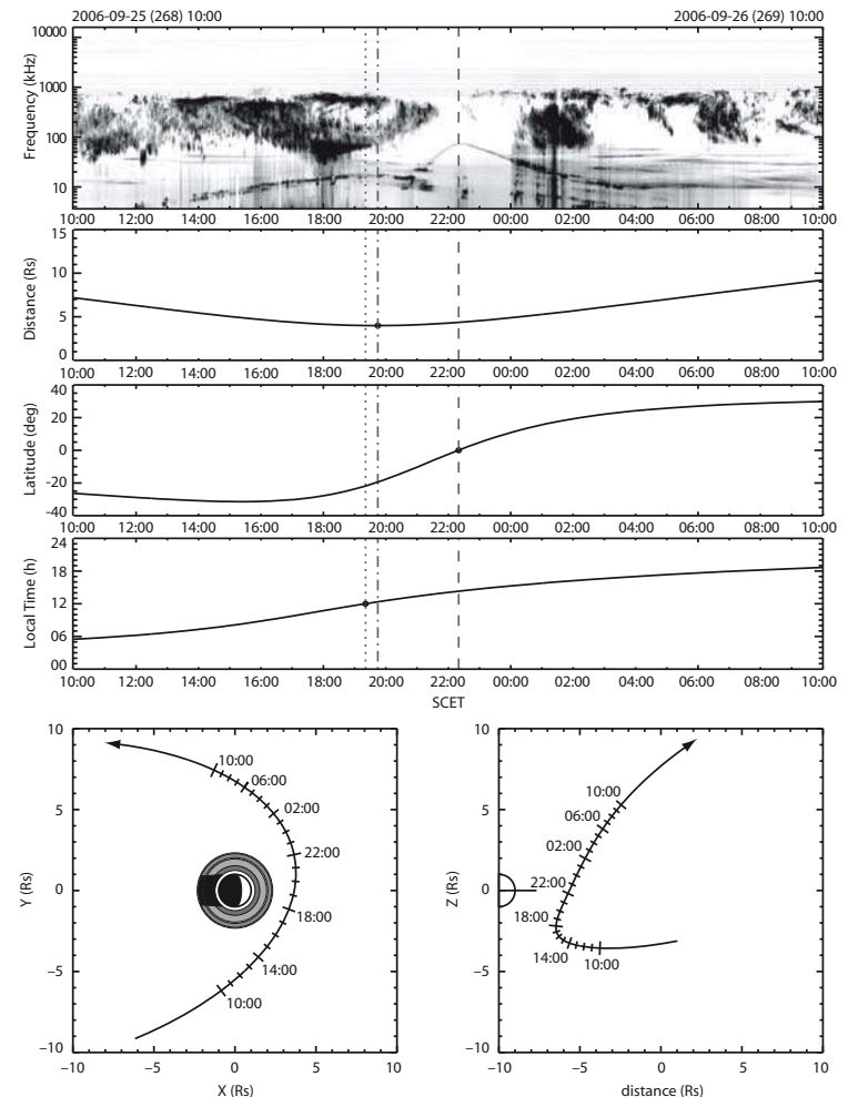
Figure 1. From top to bottom: Dynamic spectrum of the voltage autocorrelation measured on the dipole antenna (a background value has been removed for each frequency); distance to Saturn in Saturn radii ( R_S ); latitude (in degree) in the kronian equatorial frame; local time in hour. The three orbital parameters are displayed with respect to SCET in hours of day. The vertical lines indicates the noon meridian crossing (dotted line), the equator crossing (dashed line) and the closest approach (mixed line).
