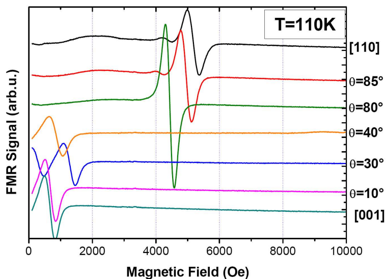
Figure 3.17: FMR spectra of GaMnAs/GaInAs 50nm thick annealed sample ( x \approx 0.07 ) for different orientations of the applied field with respect to the [001] direction of the film for rotation around the [1, \bar{1}, 0] axis, at T=110\text{K} . (X-band)
