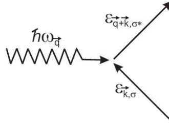
Figure 6.3: Illustration of the spin-flip scattering process.
