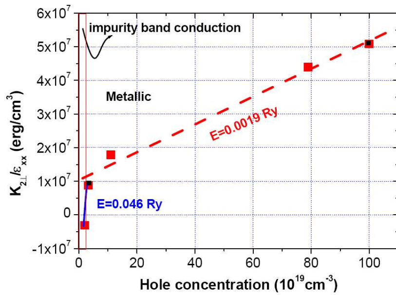
Figure 4.39: The uniaxial anisotropy constant K_{2\perp} divided by \epsilon_{xx} = \Delta a/a , the bulk lattice mismatch, as a function of the hole concentration; T = 4\text{K} . The two different regions with respect to the hole concentration (metallic/impurity band conduction) are indicated. A linear fit by eq. 4.5 in the two regimes gives a coefficient E of 0.046 Ry (impurity band) and 0.0019 Ry (metallic) regime.
