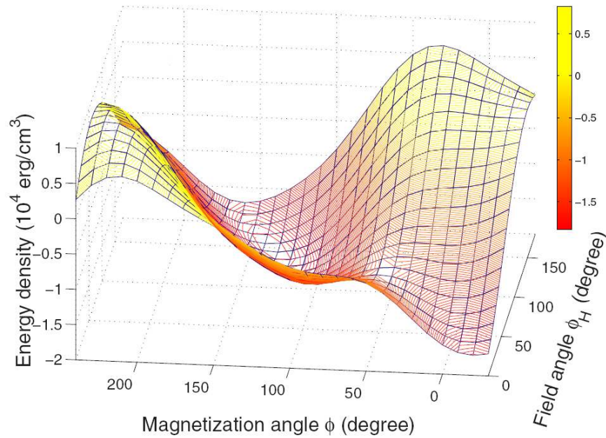
Figure 4.43: The energy density surface for the reference sample as a function of the polar angles \phi_H, \phi for an applied field of H=200\text{Oe} , the configuration is in plane; \theta = \theta_H = 90^\circ and T=20 \text{ K} .
