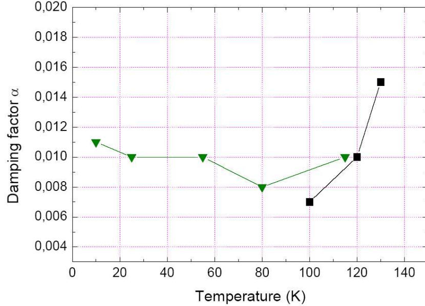
Figure 6.19: GaMnAs/GaInAs damping factor \alpha as a function of temperature and magnetic field orientation; H||[001] squares, H||[110] lower triangles.
