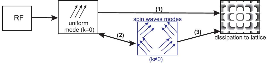
Figure 6.1: Schematic drawing of the possible paths of the relaxation of the magnetization precession [1]
