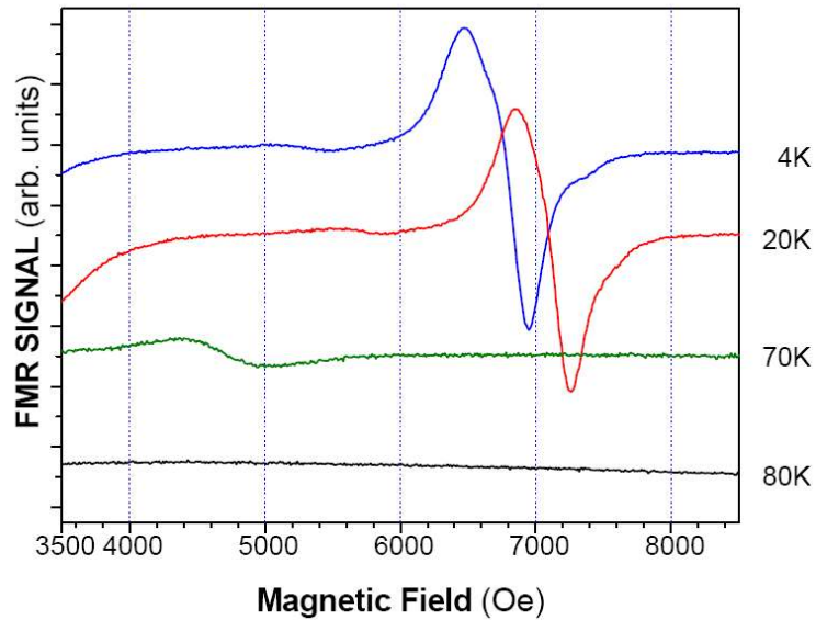
Figure 4.20: FMR spectra of sample D for H||[001] at different temperatures. Increasing the temperature from 4K to 20K shifts the resonance to higher fields.
