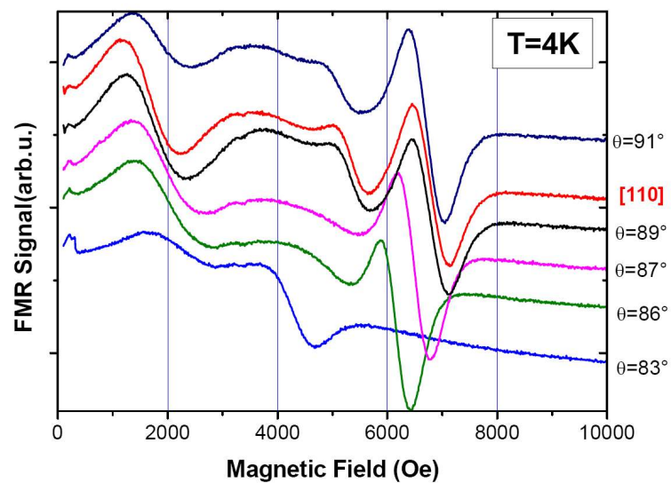
Figure 3.20: FMR spectra of GaMnAs/GaInAs 50nm thick annealed sample ( x \approx 0.07 ) for angular variation of applied field in the [1\bar{1}0] plane at T=4K. (X-band)
