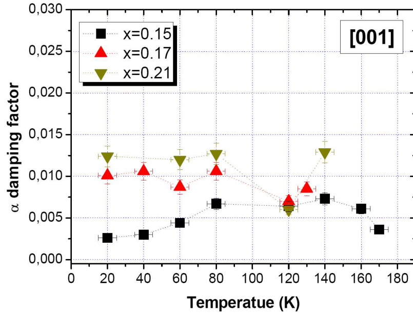
Figure 6.24: \alpha -damping factor as a function of temperature along the [001] hard axis for GaMnAs samples with different indicated Mn concentrations.
