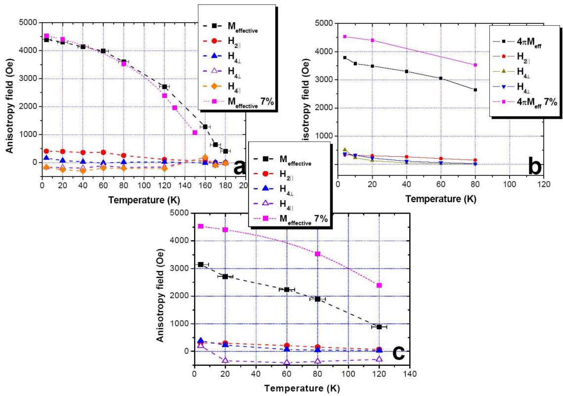
Figure 5.14: The magnetic anisotropy fields as a function of temperature for different samples((a)sample.A, (b)sample.B and (c) sample.C). The second H_{4\perp} in sample.A is related to the second observed resonance field which is attributed to the inhomogeneity of the sample. The Other fields remain unchanged for this resonance.
