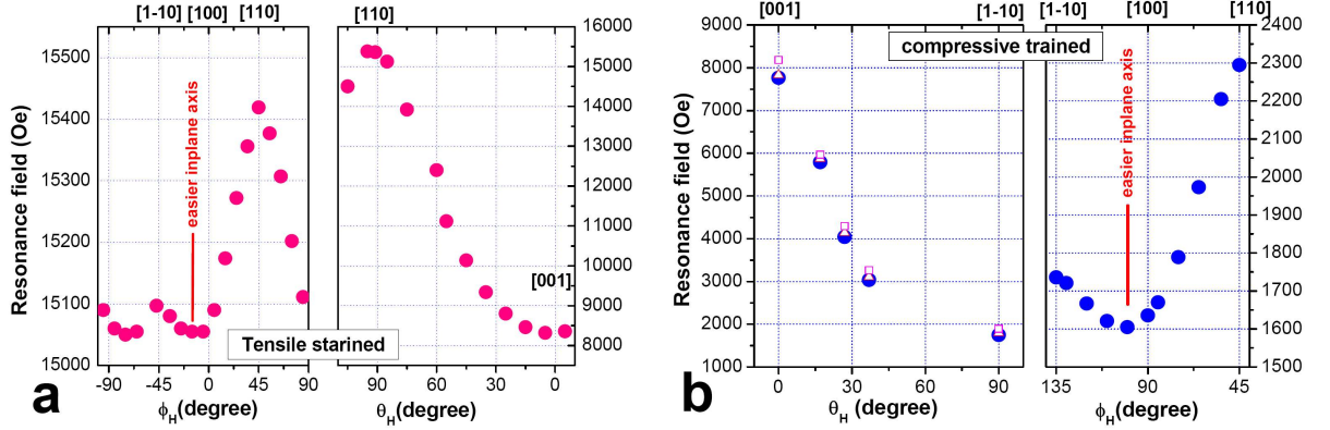
Figure 3.10: Angular variation of FMR resonance field for different orientations of applied magnetic field in [001] and /[1\bar{1}0] planes (presented by \phi and \theta respectively) for GaMnAs/GaInAs (a) and GaMnAs/GaAs (b) annealed samples ( x \approx 0.07 ).
