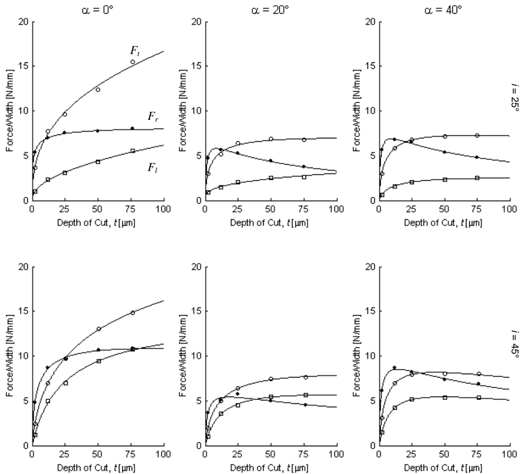
Figure 2.10. Tangential ( \ominus F_t ), radial ( \blacktriangle F_r ) and lateral ( \square F_l ) force components plotted against depth of cut for obliquity angles i = 25^\circ (upper row) and i = 45^\circ (lower row) for three different rake angles in the across cutting mode.
