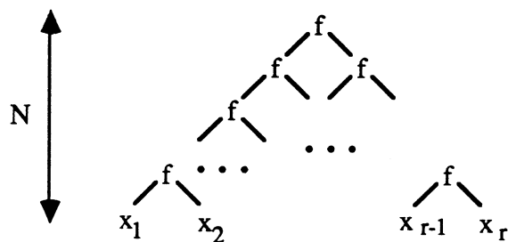
Figure 4.1: construction de \alpha_m
