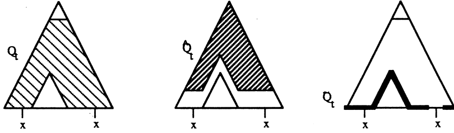
Figure 4.18: Les trois ensembles Q_t , \widetilde{Q}_t et \widetilde{\widetilde{Q}}_t
