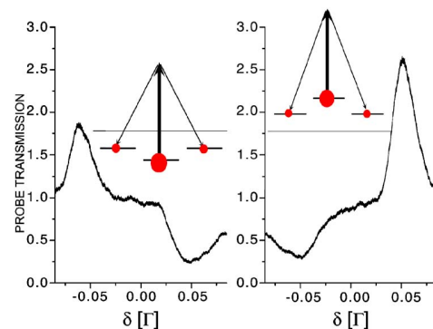
Fig. 4. (Color online) Raman gain mechanism. (a) Gain spectrum for negative pump detuning and corresponding gain spectrum ( \Delta = -5.2\Gamma , s_F = 30 , s_P = 0.07 ). (b) Gain spectrum for positive pump detuning and corresponding gain spectrum ( \Delta = +5.2\Gamma , s_F = 30 , s_P = 0.07 ). Insets indicate the different light shifts and populations corresponding to the gain part of each curve.
