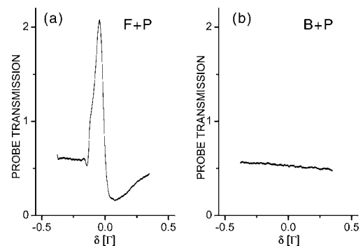
Fig. 3. Gain spectrum for F\parallel B \perp P polarization. (a) for the quasi-co-propagating pump ( F ) and probe ( P ) beams ( s_F = 30 and \Delta = -3\Gamma ). A distinctive gain of \sim 100\% is seen at the Raman condition, for \delta = \omega_{\text{Raman}} . (b) For the quasi-counter-propagating pump ( B ) and probe ( P ) beams ( s_B = 30 and \Delta = -3\Gamma ) no gain is observed.
