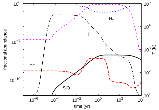
Fig. 8. Chemical evolution in a 25 \text{ km s}^{-1} J shock propagating through a molecular cloud ( n_H = 10^4 \text{ cm}^{-3} ). SiO is not produced through gas-phase reactions but directly from the vaporisation of silicate grains. The SiO is progressively removed from the gas phase by accretion onto grain mantles.
