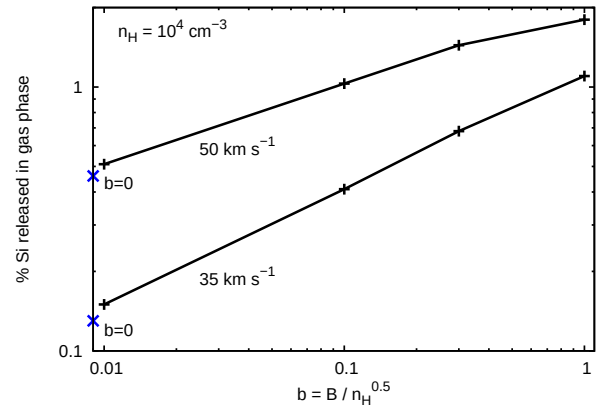
Fig. 6. The percentage of silicon released into the gas phase, for 35 and 50 \text{ km s}^{-1} J shocks propagating into a cloud of pre-shock density 10^4 \text{ cm}^{-3} , as a function of the factor b = B / \sqrt{n_H} . The values for pure hydrodynamical shock ( b = 0 , i.e. B = 0 ) are shown on the left axis.
