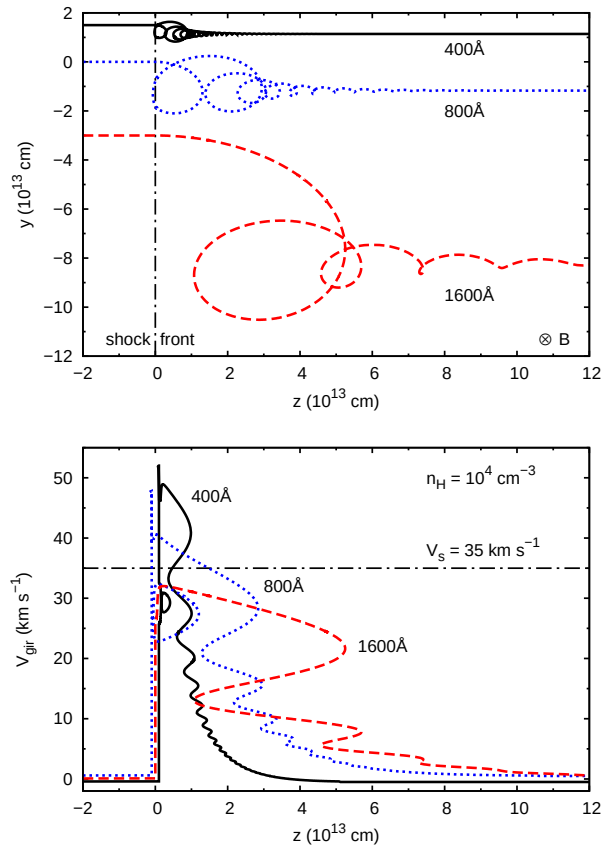
Fig. 2. (top) The trajectories of three silicate test grains of radii 400, 800 and 1600 Å through a 35 \text{km s}^{-1} J shock propagating in a molecular cloud ( n_H = 10^4 \text{ cm}^{-3} ). The grains gyrate around the magnetic field lines transverse to the shock plane. (bottom) The gyration velocity profiles for the same three test grains, i.e. the velocity of the grains relative to the gas. The curves have been a little shifted from z = 0 for clarity.
