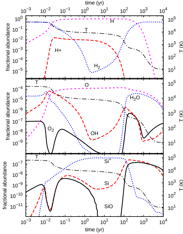
Fig. 9. Same as Fig. 8 but for a dissociative 35 km s -1 J shock. The SiO produced by grain vaporisation is dissociated by H + and reformed later by the gas-phase reaction of Si with O 2 and OH as soon as the ionisation fraction is low enough. Finally, SiO accretes onto the surfaces of grains in the form of icy mantles. In our work we have adopted an initial gas-phase fractional abundance of O 2 of X(\text{O}_2) = 10^{-7} , in accordance with the recent SWAS results (Larsson et al. 2007).
