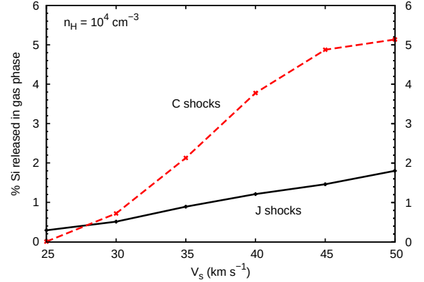
Fig. 11. Percentage of Si released into the gas phase as a function of the shock velocity for C-type (Gusdorf et al. 2008a) and J-type shocks (this study) propagating in a molecular cloud ( n_H = 10^4 cm -3 , B = 100\mu\text{G} , i.e. b = 1 ). The May et al. (2000) sputtering yields were used in both cases. In the work of Gusdorf et al. (2008a), a fractional abundance X(\text{PAH}) = 10^{-6} is necessary in order to raise the magnetosonic velocity to \sim 60 km s -1 (see Paper I, Table 1) and allow for the existence of C-shocks as fast as 50 km s -1 . Both of these shock models show the same order of magnitude for silicate dust destruction (to within a factor 2-3).
