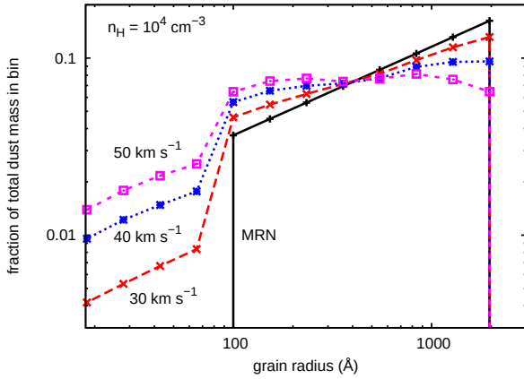
Fig. 7. The silicate dust mass distribution before and after the passage of J shocks propagating through a cloud of density n_H = 10^4 \text{ cm}^{-3} . The results are almost identical for denser clouds with n_H = 10^5 and 10^6 \text{ cm}^{-3} and are similar for carbon grains. However, for carbon the change in the slope of the mass distribution is less pronounced.
