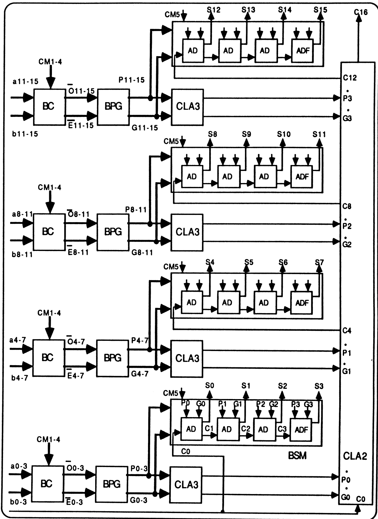
Figure 3.40 : UAL 16 bits à base "Ripple Within Groups, Look Ahead Between Groups Adder".
