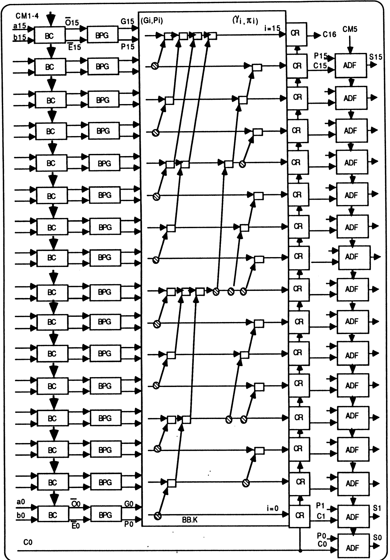
Figure 3.44 UAL type "Brent_Kung"
