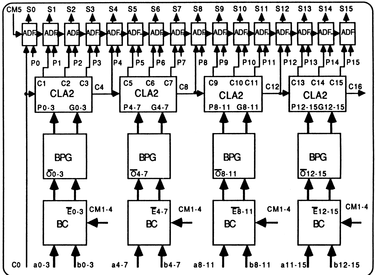
Figure 3.41 : schéma général de l'UAL de type "Carry Look Ahead Within Groups, Ripple Between Groups Adder".
