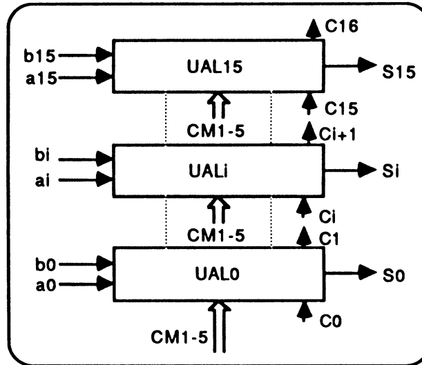
Figure 3.6 : UAL type "Ripple Carry Adder"
