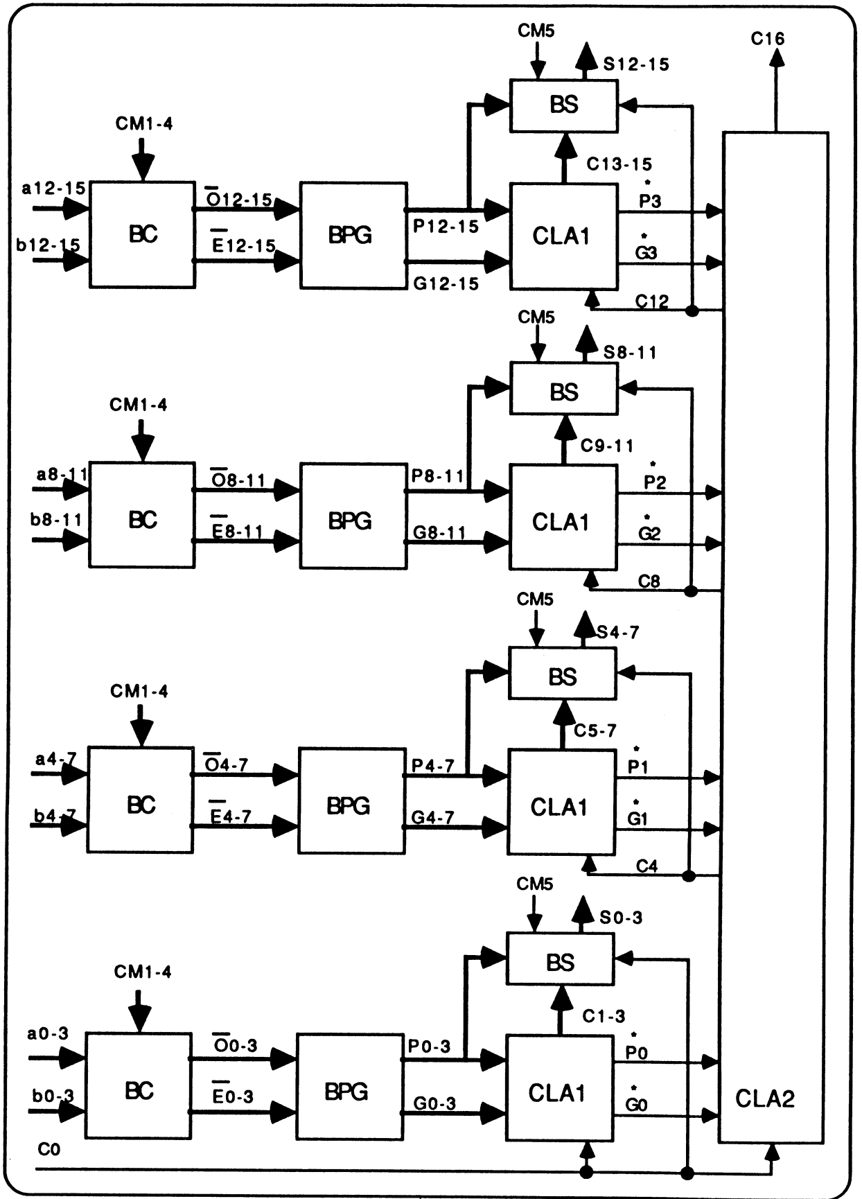
Figure 3.33 : UAL 16 bits de type "Full Carry Look Ahead Adder".
