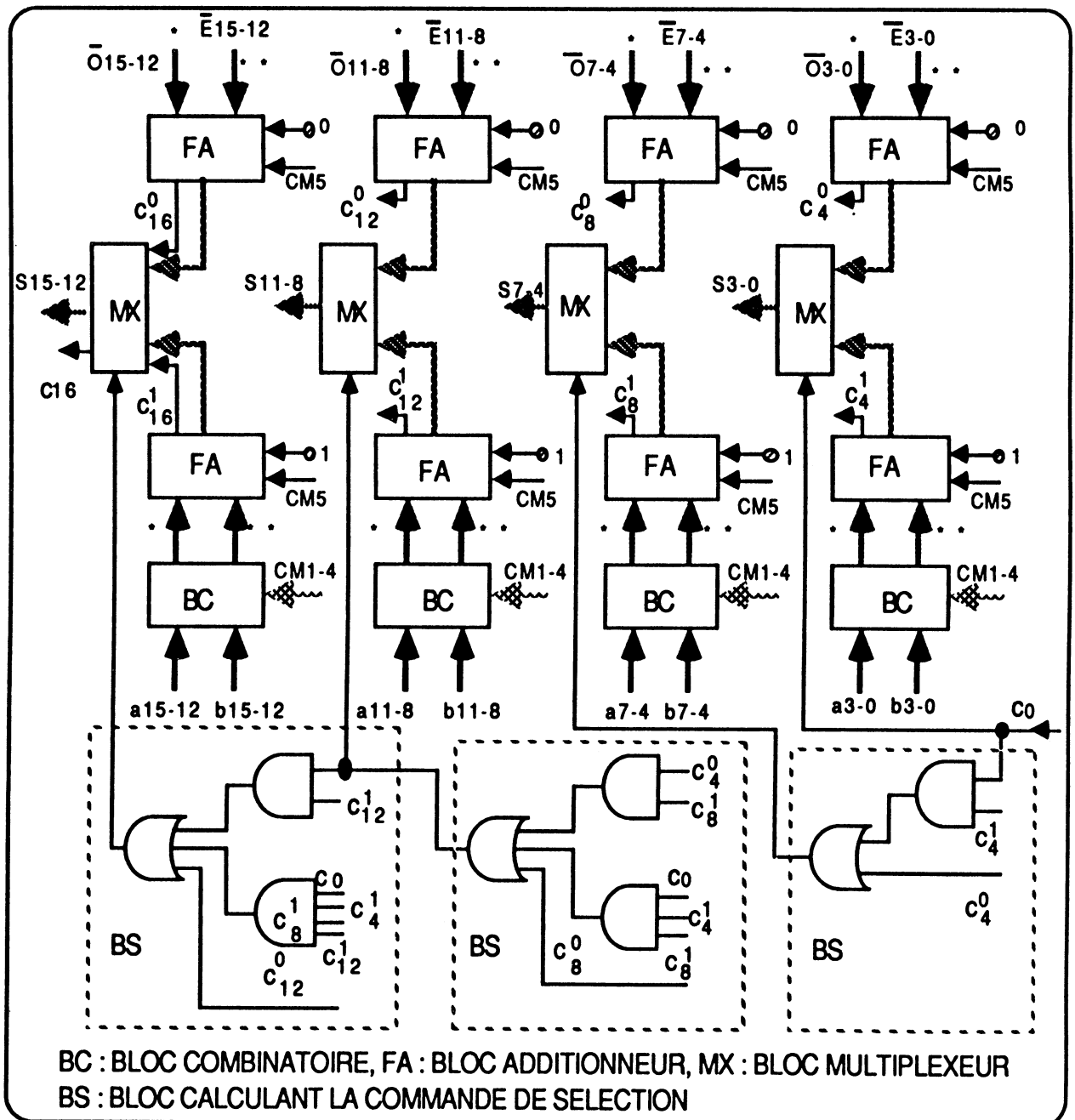
Figure 3.26 : UAL de type "Carry Select Adder"
