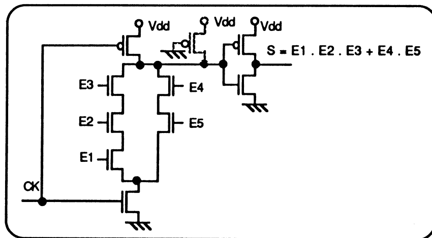
Figure 3.12 : structure CMOS domino.
