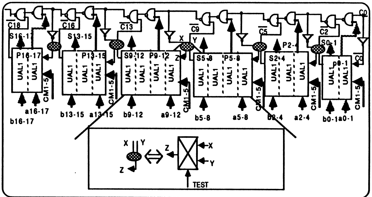
Figure 3.31 : UAL "Carry-Skip" testable.
