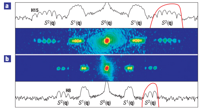
Figure 2 Spectra S(q) of two single-shot interferograms (in log scale). a , Case where harmonics 10–15 are selected using a 200-nm-thick tin filter. b , Case where harmonics 8–10 are selected with a 200-nm-thick indium filter. The transmission curves of these filters are shown as red lines around the S^2(q) term. In both cases, the generation is based on CWE on a silica target, and \alpha_{\omega_L} = 0.57 .
