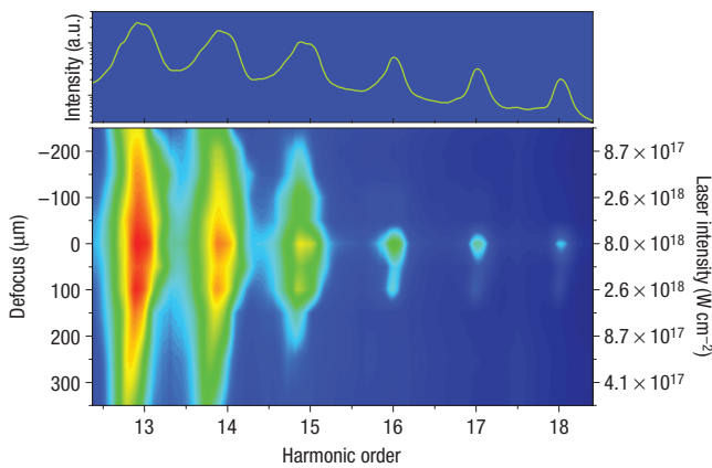
Figure 6 Harmonic spectrum dependency on the laser intensity. Harmonic spectra obtained on plastic plotted in logarithmic scale as a function of distance between the target surface and the laser best focus. The right axis shows the estimated peak intensity corresponding to each position. The intensity at the best focus is about 8 \times 10^{18} \text{ W cm}^{-2} , and the upper panel shows the spectrum obtained at this intensity. Each spectrum is averaged on 5 laser shots, and measurements were carried out for 10 focusing positions.
