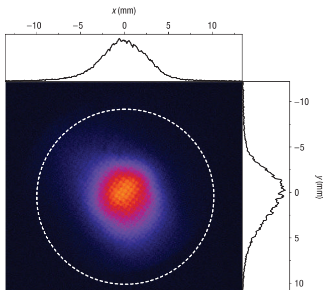
Figure 2 Spatial profile of the harmonic extreme-ultraviolet beam. This beam corresponds to the superposition of harmonics with orders 10 p 15, 37 cm away from the target. The white dashed circle shows the spatial extension of the top-hat laser beam in the same plane. This extreme-ultraviolet beam has a divergence of 14 mrad (full-width at half-maximum).
