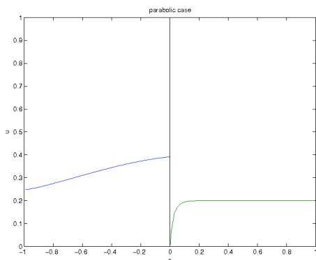
FIG. 5.3 – t = 0.8 , \varepsilon = 0.1 , F_0^n given by (5.78)-(5.79).
