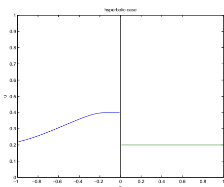
FIG. 5.5 – t = 0.8 , \varepsilon = 0 , F_0^n given by (5.80).
