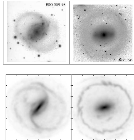
Fig. 7. Two examples showing the morphological structures of ESO 509-98 and NGC 1543 (top panel) compared to simulated galaxies in MOND (bottom panel). Rings and pseudo-rings structures are well reproduced with modified gravity. The size of the box in the simulation (bottom panel) is 80 kpc \times 80 kpc.
