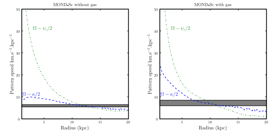
Fig. 10. Localisation of the peanut resonance for the MOND-Sc galaxy without gas (left) and with gas (right). With gas, the bar pattern speed is about 8 \text{ km} \cdot \text{s}^{-1} \cdot \text{kpc}^{-1} (the gray region marks the variation of the bar pattern speed during time, see text) so the peanut resonance occurs near 9 kpc, while it appears at 12 kpc without gas.
