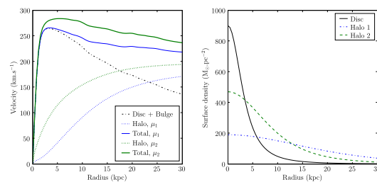
Fig. 2. Left: rotation curves of an Sa-type galaxy using the standard ( \mu_1 , this work) and simple ( \mu_2 , TC07) \mu -functions. In each case, the halo needed in the DM model to obtain the MOND rotation curve is plotted too (Halo, \mu_1 , Halo, \mu_2 curves). Right: Surface density of the stellar disc compared to the dark matter halo (in the Newtonian model) needed to fit the MOND rotation curve if the free function is the standard one (1, this work) or the simple one (2, TC07).
