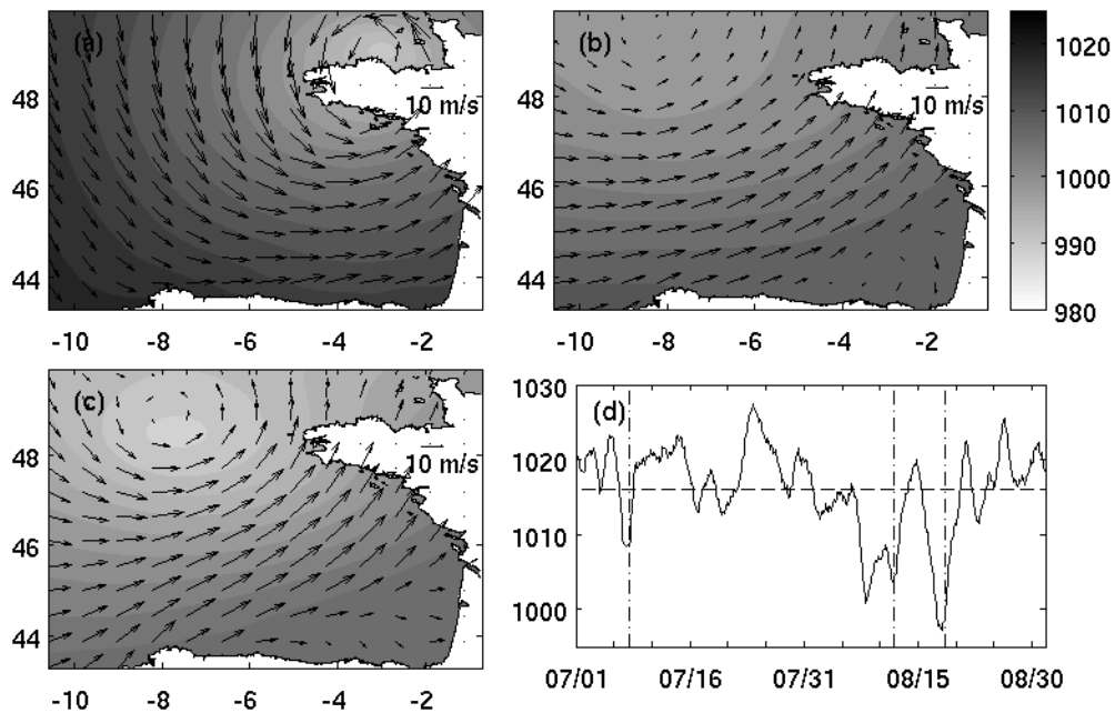
Figure E.4: 10 m wind and atmospheric pressure over the zone on (a) July 7, (b) August 12 and (c) August 19. Wind reference arrow is 10 \text{ ms}^{-1} , P is in hPa. (d) Averaged pressure over the domain during the study period. The dashed line is the time mean of the series, 1016 hPa. Dates of (a), (b) and (c) are in dot-dashed lines.
