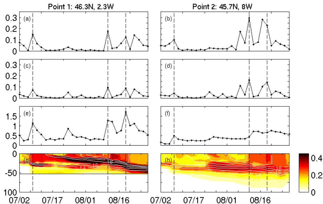
Figure E.9: Left: model outputs from Point 1 (cf. Figure E.5). Right: same for Point 2. (a) and (b) : Evolution of the reference wind stress intensity ( N.m^{-2} ) during the simulation. (c) and (d) : wind stress intensity ensemble standard deviation ( N.m^{-2} ). (e) and (f) : sea surface elevation ensemble standard deviation (cm). (g) and (h) : upper 100 m temperature ensemble standard deviation ( ^{\circ}C ) on the vertical (y-axis, in m). Thin white lines: reference model potential temperature (contour every 1^{\circ}C ). Bottom is indicated (black line) on (g). For all: reference dates from Figure E.4 in dashed lines.
