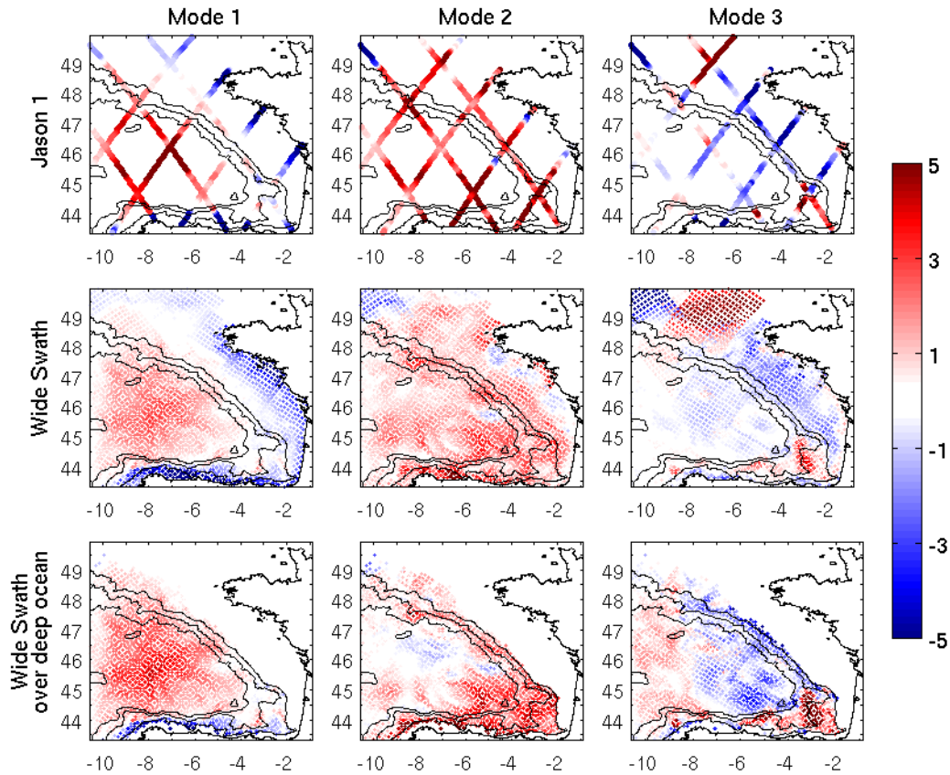
Figure E.12: First 3 dominant eigenmodes (no dimension) of the scaled representer matrices, for the three altimetry experiments from Figure E.11: Jason 1 (top), full Wide Swath (middle) and Wide Swath deep ocean-only (bottom). From left to right: first, second and third modes. Thick line: 200, 2000 and 4000 m isobaths.
