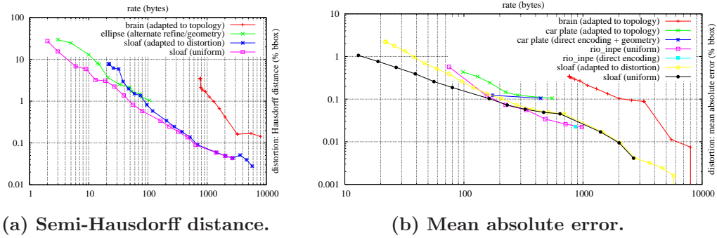
Figure V.22: Compression results: on complex models, topology control is more expensive with progressive encoding.
