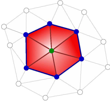
(a) The star of a vertex is the union of the open star (in red) with the link (in blue).
