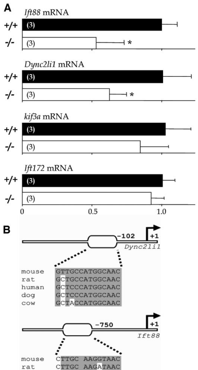
FIG. 3. The expression of RFX3 target genes is reduced in dpc 19 Rfx3 -deficient embryos. A: Dync2li1 , Ift88 , Kif3a , and Ift172 mRNAs were quantified in the pancreases of Rfx3 +/+ and Rfx3 -/- littermates. Values were normalized with respect to TATA-binding protein mRNA and expressed relative to Rfx3 +/+ . The means \pm SE are shown. Numbers of mice analyzed are indicated. * P < 0.05. B: Putative RFX3 binding sites in the Dync2li1 and Ift88 genes are conserved in all vertebrate species for which the sequences are available. Shading indicates identity with the consensus RFX-binding site (GTNRCCNRR-GYAAC).
